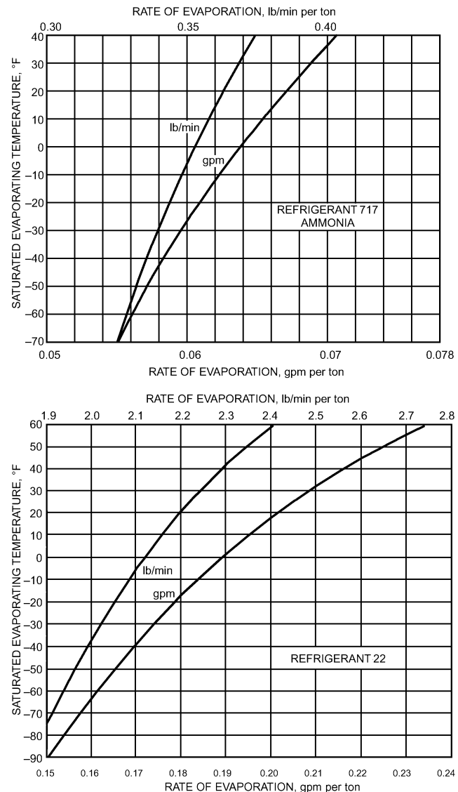
Fig. 7 Charts for Determining Rate of Refrigerant Feed (No Flash Gas)
