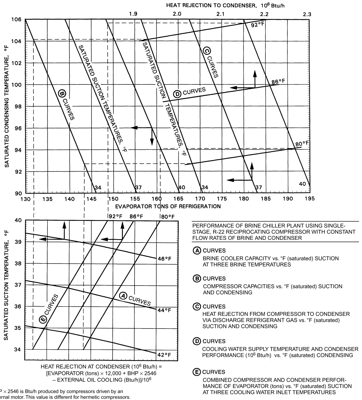
Fig. 1 Brine Chiller Balance Curve
