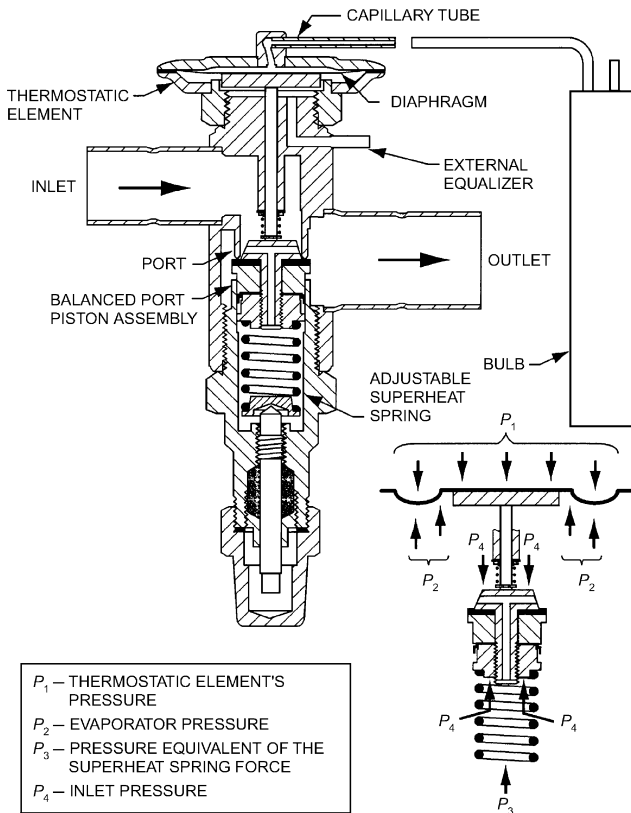
Fig. 10 Typical Balanced Port Thermostatic Expansion Valve
