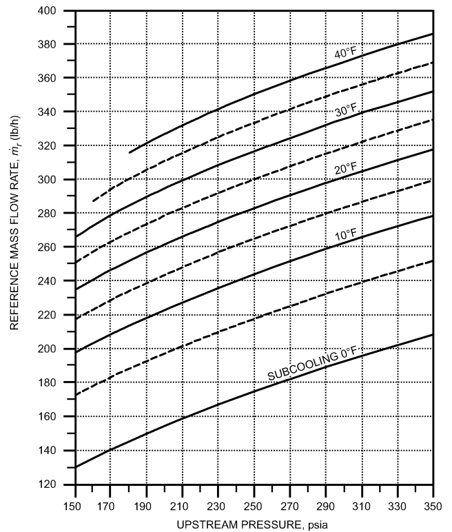
Fig. 61 R-22 Mass Flow Rate vs. Condenser Pressure for Reference Short Tube: L = 0.5 \text{ in.}, D = 0.053 \text{ in.}, \text{Sharp-Edged} (Adapted from Aaron and Domanski 1990)
