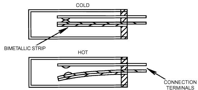
Fig. 4 Direct Temperature Switch
