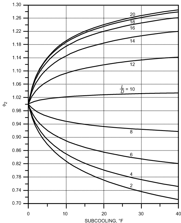
Fig. 63 Correction Factor for L/D vs. Subcooling (R-22) (Adapted from Aaron and Domanski 1990)
