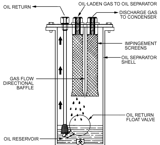
Fig. 40 Discharge-Line Lubricant Separator
