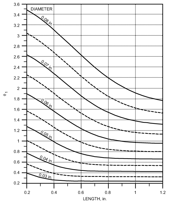
Fig. 62 Correction Factor for Short-Tube Geometry (R-22) (Adapted from Aaron and Domanski 1990)
