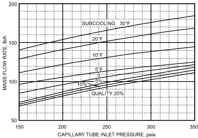
Fig. 50 Mass Flow Rate of R-22 Through Capillary Tube (Capillary tube diameter is 0.066 in. ID and length is 60 in.)
