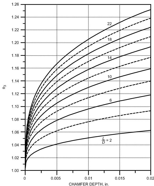
Fig. 64 Correction Factor for Inlet Chamfering (R-22) (Adapted from Aaron and Domanski 1990)
