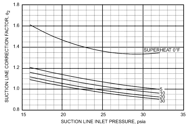
Fig. 58 Suction Line Condition Correction Factor for R-134a Quality Inlet Conditions
