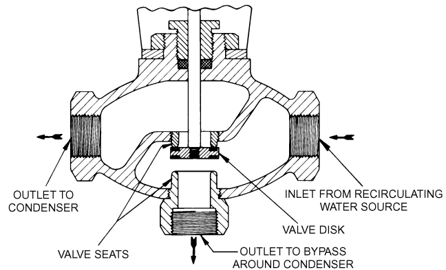
Fig. 36 Three-Way Condensing Water Regulator
