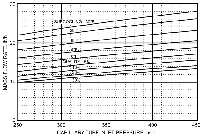
Fig. 47 Mass Flow Rate of R-410A Through Capillary Tube (Capillary tube diameter is 0.034 in. ID and length is 130 in.)
