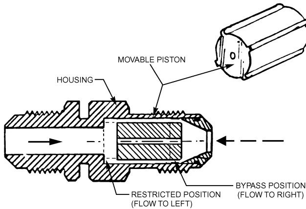
Fig. 59 Schematic of Movable Short-Tube Restrictor
