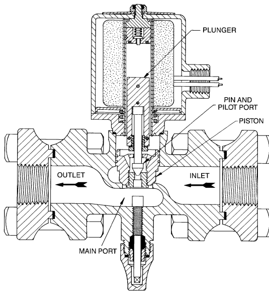
Fig. 32 Normally Closed Pilot-Operated Solenoid Valve with Hammer-Blow and Mechanically Linked Piston-Pin Plunger Features
