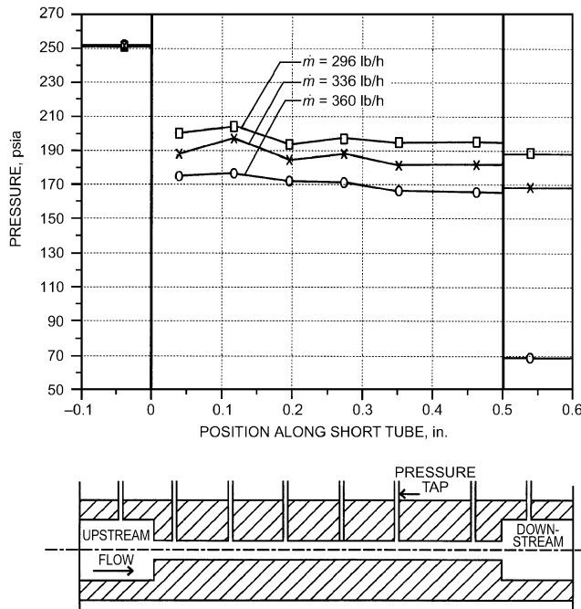
Fig. 60 R-22 Pressure Profile at Various Downstream Pressures with Constant Upstream Conditions: L = 0.5 \text{ in.}, D = 0.053 \text{ in.}, \text{Subcooling } 25^\circ\text{F} (Adapted from Aaron and Domanski 1990)
