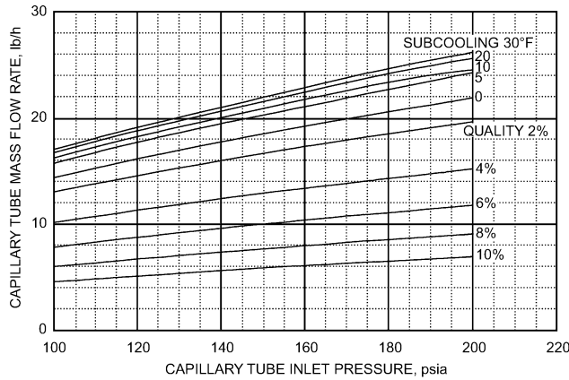
Fig. 53 Inlet Condition Rating Chart for R-134a
