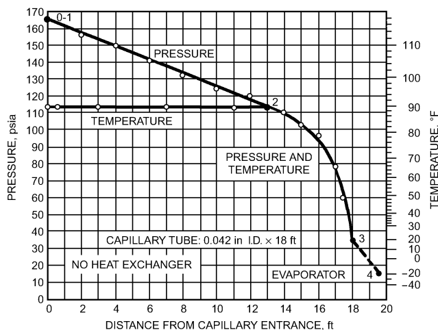
Fig. 41 Pressure and Temperature Distribution Along Typical Capillary Tube (Bolstad and Jordan 1948)
