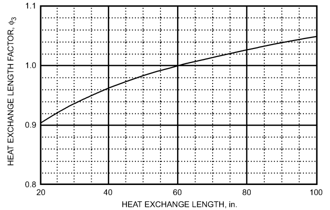
Fig. 56 Heat Exchange Length Correction Factor for R-134a Subcooled Inlet Conditions
