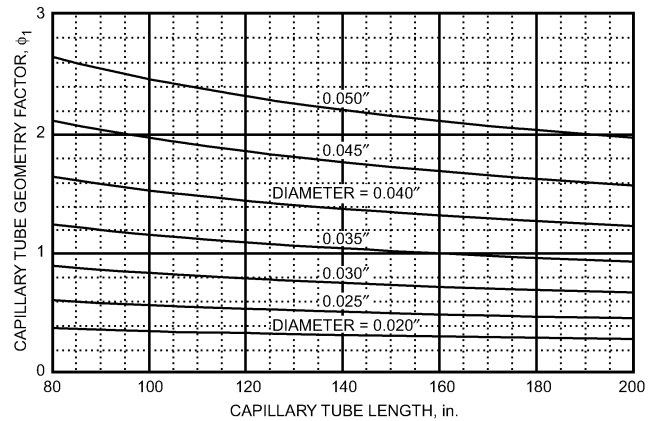
Fig. 57 Capillary Tube Geometry Correction Factor for R-134a Quality Inlet Conditions
