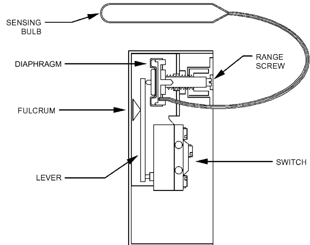
Fig. 3 Indirect Temperature Switch
