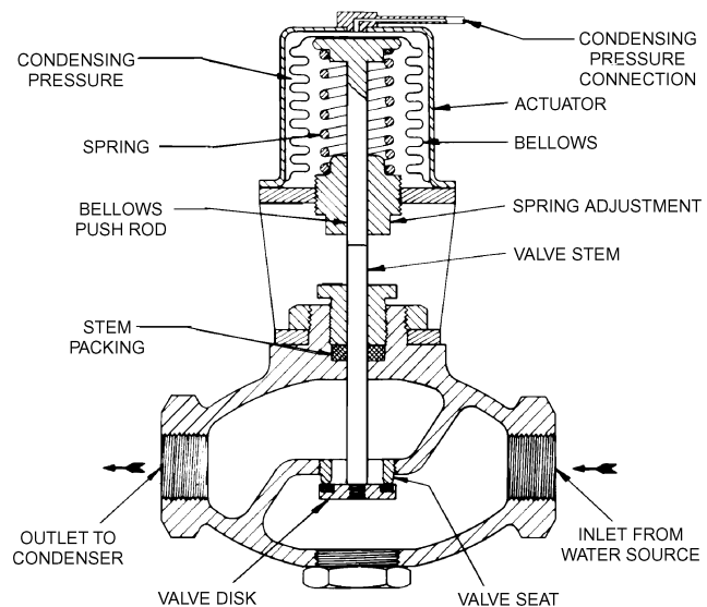
Fig. 35 Two-Way Condensing Water Regulator
