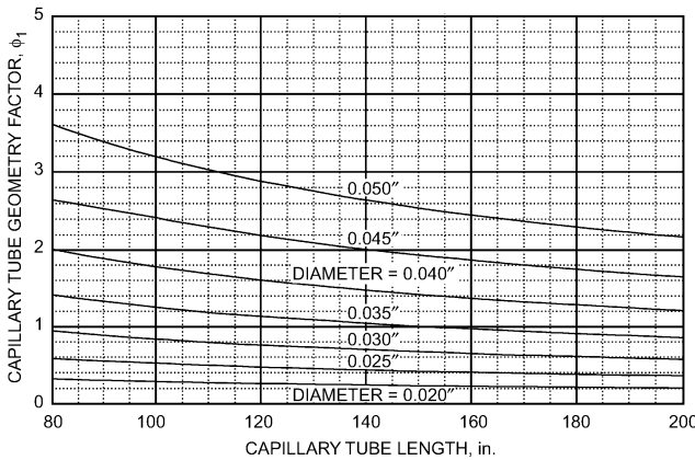
Fig. 54 Capillary Tube Geometry Correction Factor for Subcooled R-134a Inlet Conditions
