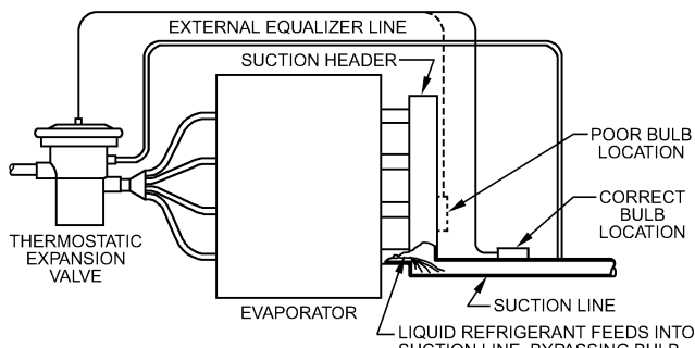
Fig. 15 Bulb Location for Thermostatic Expansion Valve
