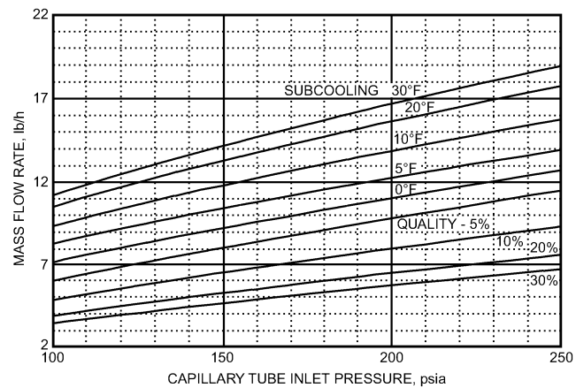
Fig. 45 Mass Flow Rate of R-134a Through Capillary Tube (Capillary tube diameter is 0.034 in. ID and length is 130 in.)
