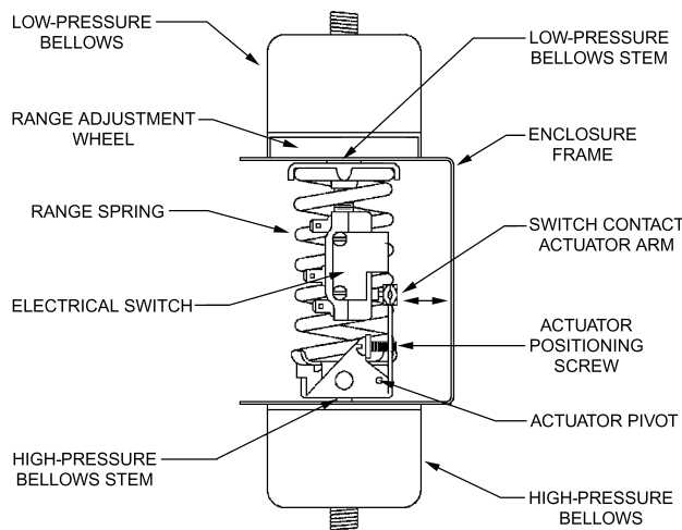
Fig. 6 Differential Pressure Switch
