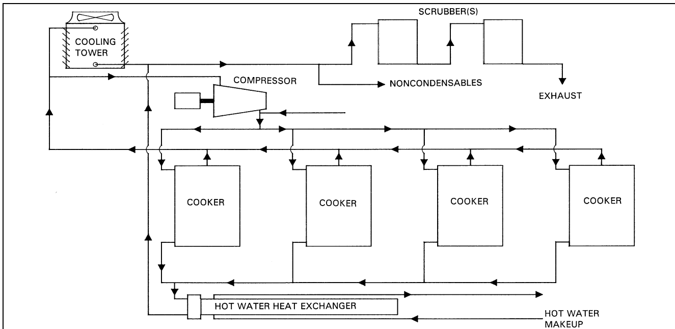
Fig. 19 Heat Recovery Heat Pump System in a Rendering Plant
