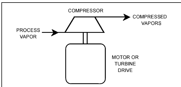
Fig. 3 Open Vapor Recompression Cycle
