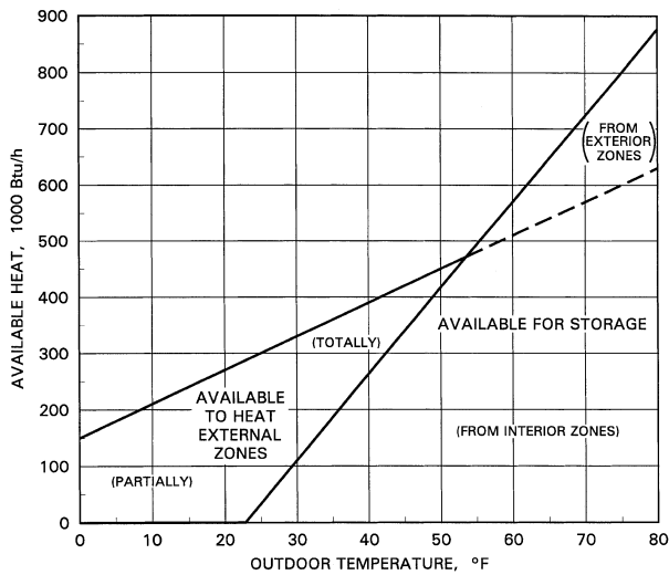
Fig. 27 Internal Heat Available for Recovery During Occupied Periods
