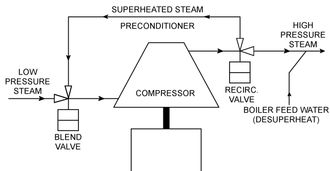
Fig. 15 Recompression of Boiler-Generated Process Steam
