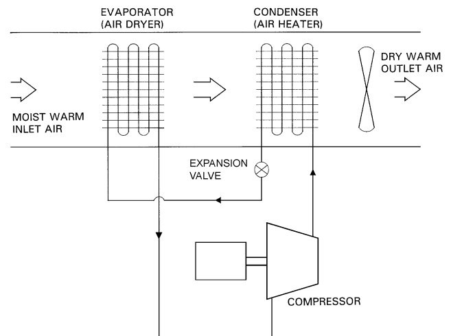
Fig. 10 Dehumidification Heat Pump
