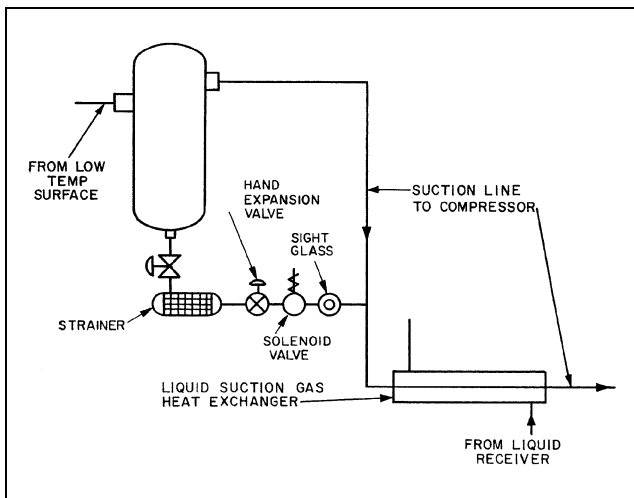
Fig. 7 Suction Line Separator for Protection Against Liquid Floodback
