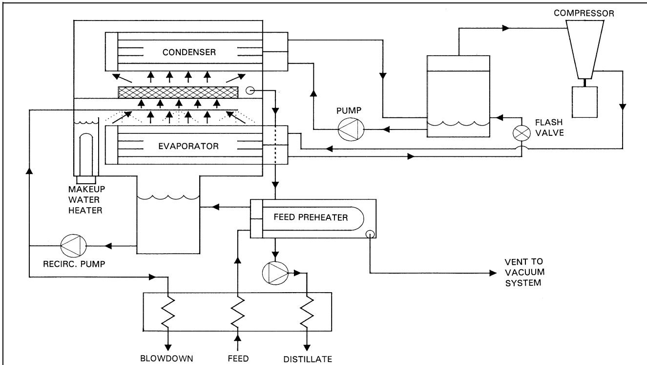
Fig. 14 Closed-Cycle Vapor Compression System
