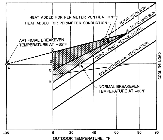
Fig. 34 Non-Heat-Recovery System
