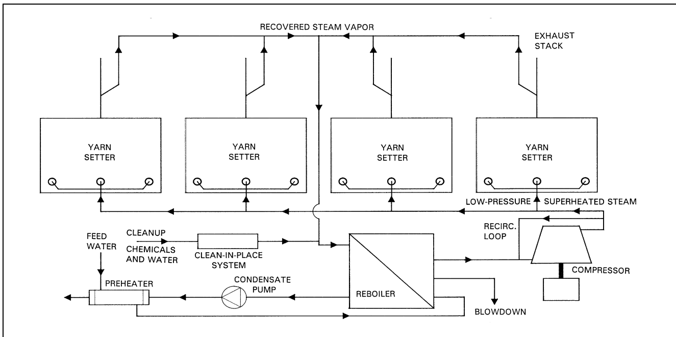
Fig. 20 Semi-Open Cycle Heat Pump in a Textile Plant
