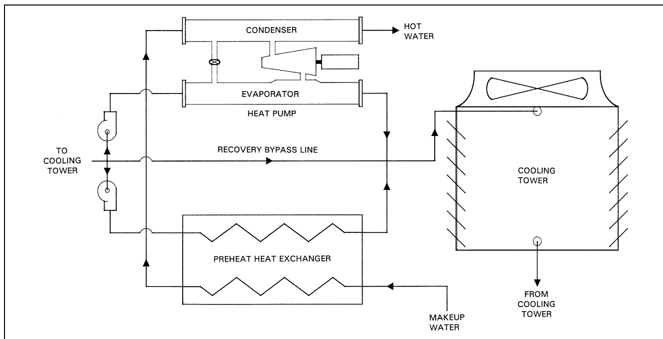
Fig. 11 Cooling Tower Heat Recovery Heat Pump
