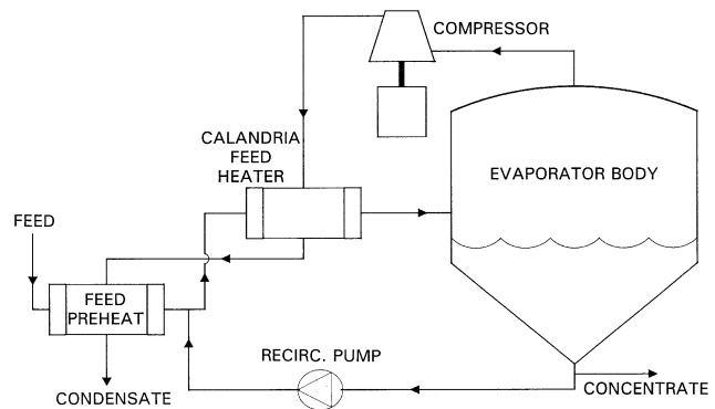
Fig. 16 Single-Effect Heat Pump Evaporator
