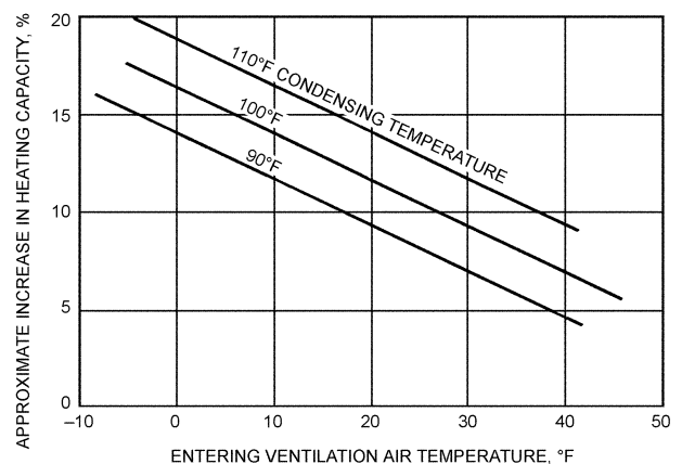
Fig. 9 Typical Increase in Heating Capacity Resulting from Use of Liquid Subcooling Coil
