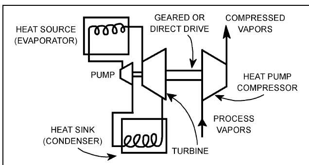
Fig. 4 Heat-Driven Rankine Cycle
