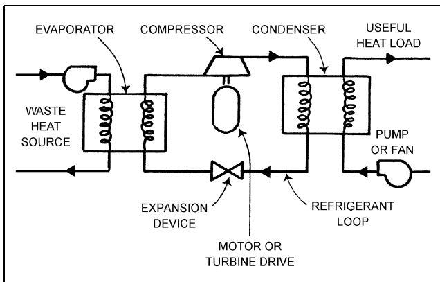
Fig. 1 Closed Vapor Compression Cycle
