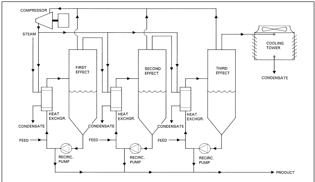
Fig. 17 Multiple-Effect Heat Pump Evaporator
