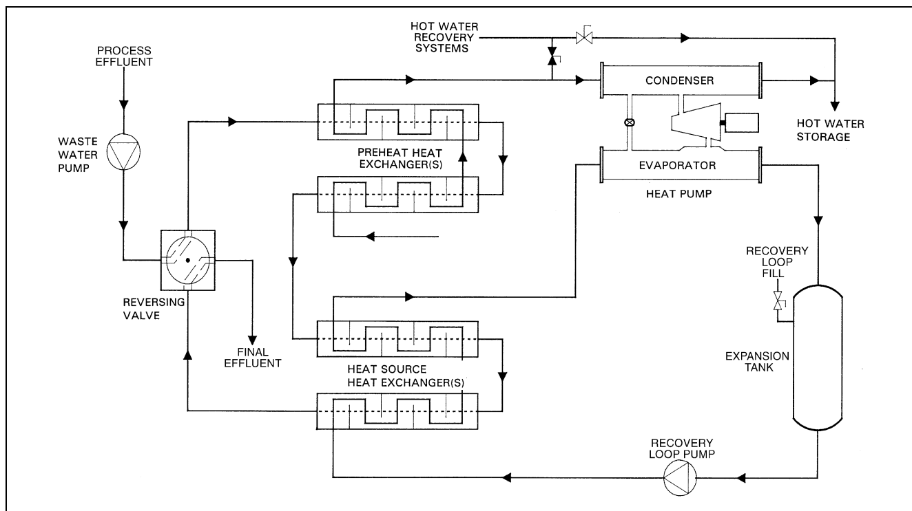
Fig. 12 Effluent Heat Recovery Heat Pump
