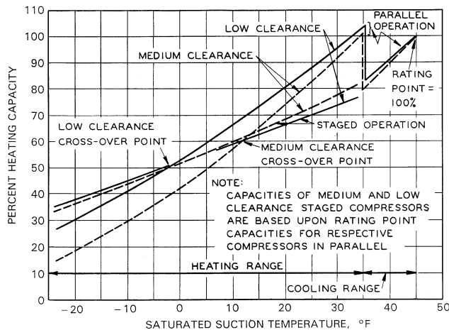
Fig. 6 Comparison of Parallel and Staged Operation for Air-Source Heat Pumps
