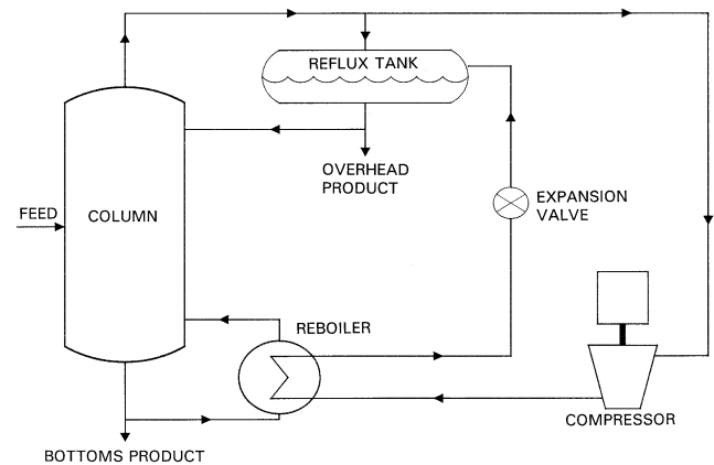
Fig. 18 Distillation Heat Pump System
