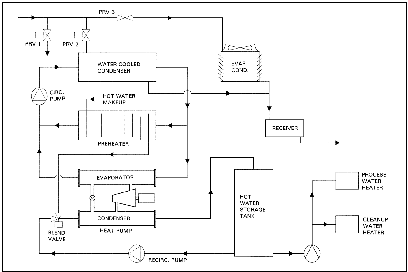
Fig. 13 Refrigeration Heat Recovery Heat Pump
