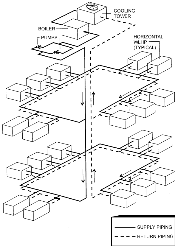
Fig. 28 Heat Recovery System Using Water-to-Air Heat Pumps in a Closed Loop
