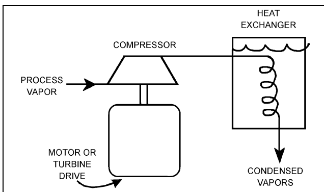
Fig. 2 Mechanical Vapor Recompression Cycle with Heat Exchanger
