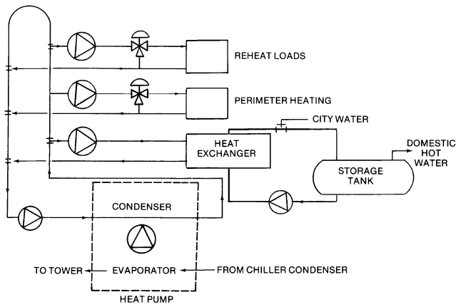
Fig. 21 Heat Recovery Heat Pump
