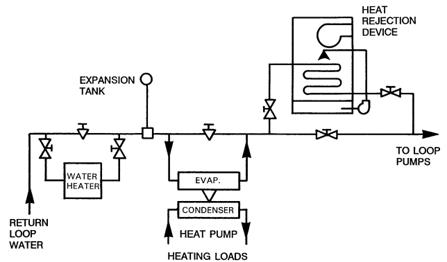
Fig. 30 Secondary Heat Recovery from WLHP System (Adapted from Marketing the Industrial Heat Pump , Edison Electric Institute 1989)
