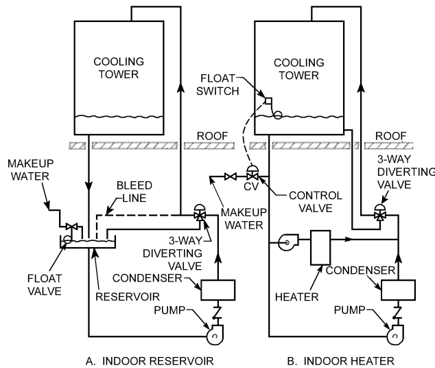
Fig. 4 Cooling Tower Piping to Avoid Freeze-Up
