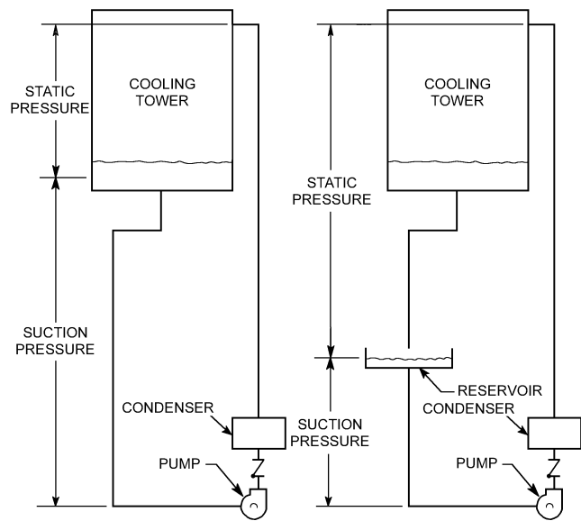
Fig. 3 Schematic Piping Layout Showing Static and Suction Head
