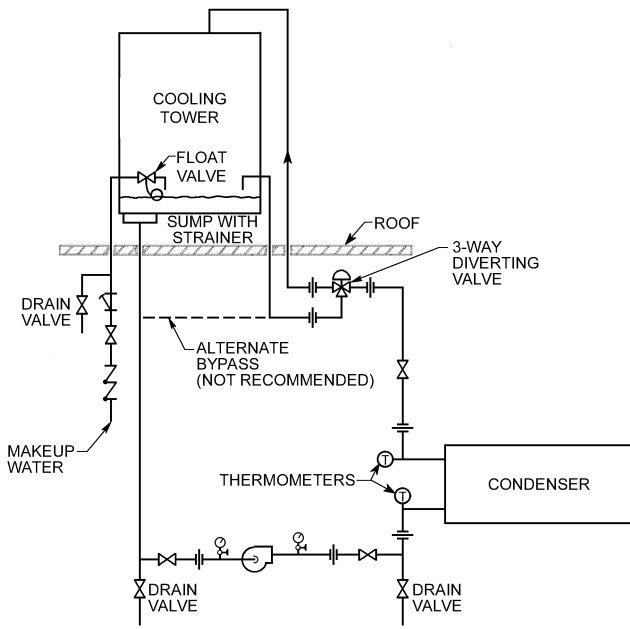
Fig. 2 Cooling Tower Piping System
