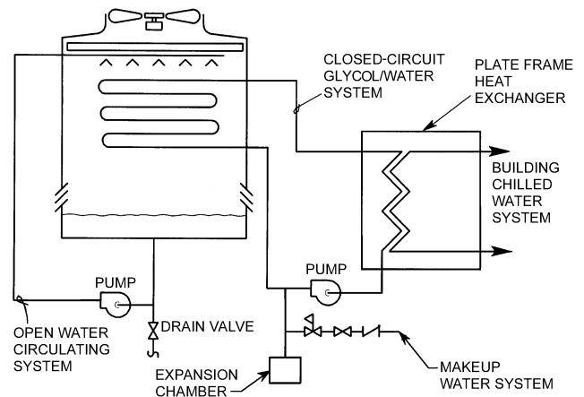
Fig. 5 Closed-Circuit Cooler System
