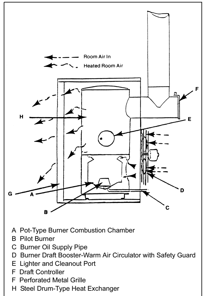
Fig. 4 Oil-Fueled Heater with Vaporizing Pot-Type Burner
