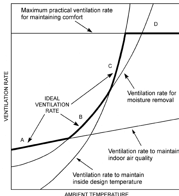
Fig. 1 Logic for Selecting the Appropriate Ventilation Rate in Livestock Buildings
