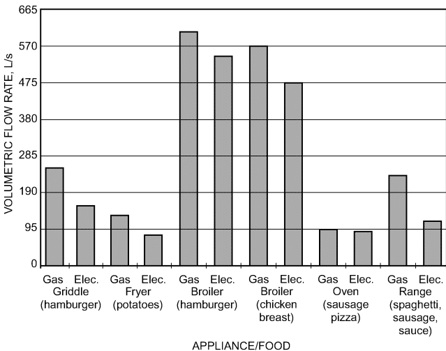
Fig. 2 Plume Volumetric Flow Rate at Hood Entrance from Various Commercial Cooking Appliances Source: Kuehn et al. (1999)
