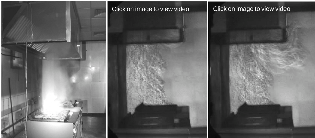
A. TEST SETUP: Two charbroilers under 2.5 m long wall-mounted canopy hood, cooking hamburgers. B. Schlieren photo of capture and containment at 1700 L/s exhaust rate. Hot, clear air visualization, no cooking. C. Schlieren photo of spillage and containment at 1300 L/s exhaust rate. Hot, clear air visualization, no cooking.
