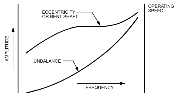
Fig. 17 Vibration Caused by Eccentricity
