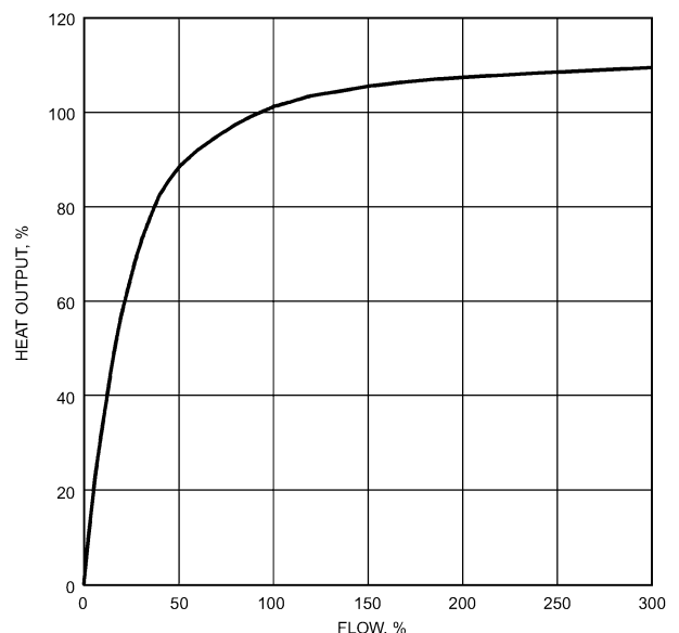
Fig. 3 Typical Heating Coil Heat Transfer Versus Water
