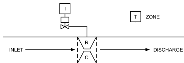
Fig. 33 Single-Duct Constant-Volume Zone Reheat
