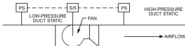
Fig. 61 High-Limit Static Pressure Controller
