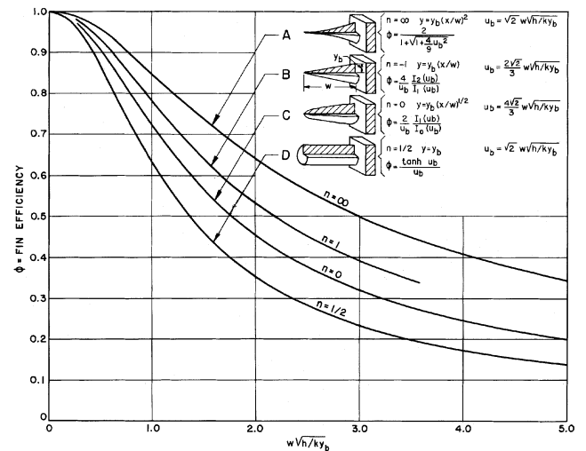
Fig. 19 Efficiency of Four Types of Spine
