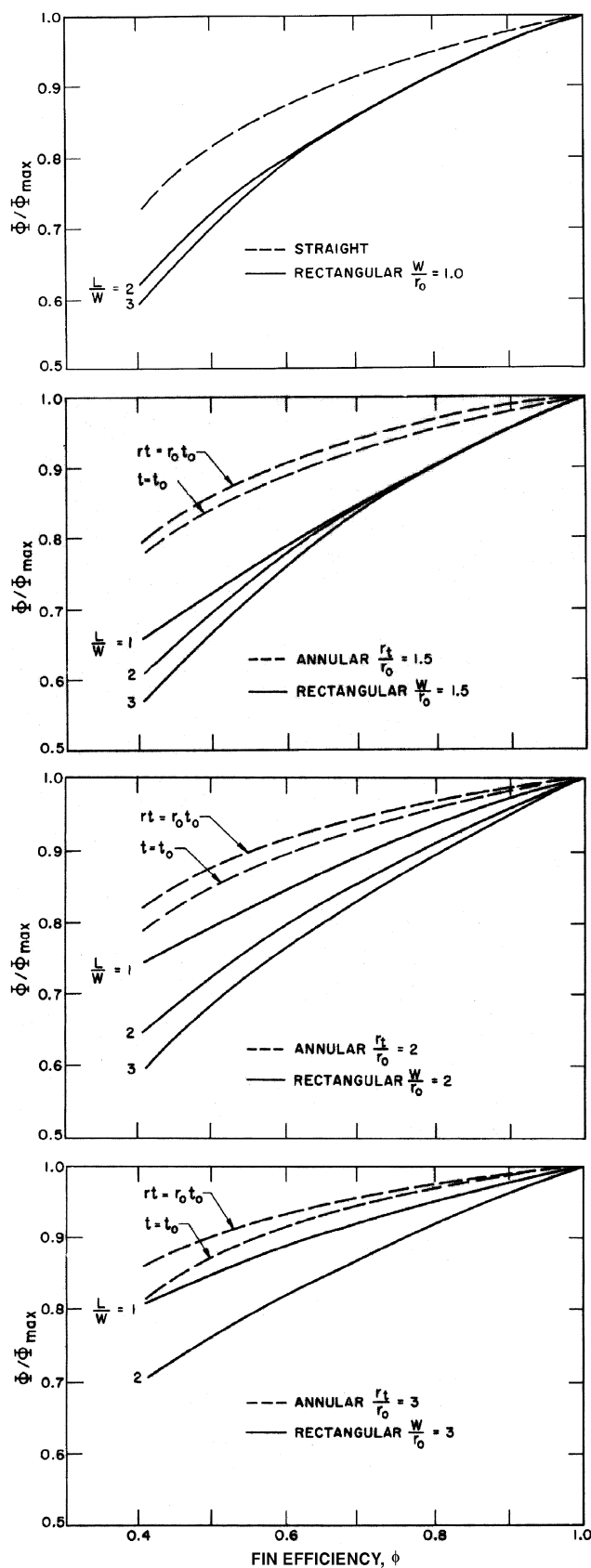
Fig. 22 Variation of Fin Resistance with Efficiency for Annular and Rectangular Fins (Gardner 1945)
