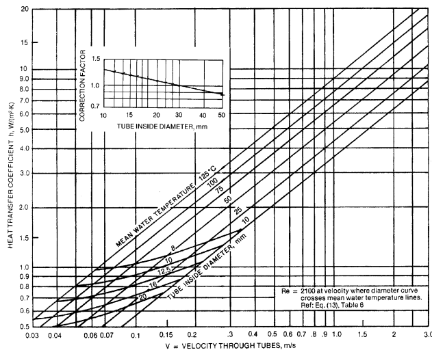
Fig. 11 Heat Transfer Coefficient for Turbulent Flow of Water Inside Tubes
