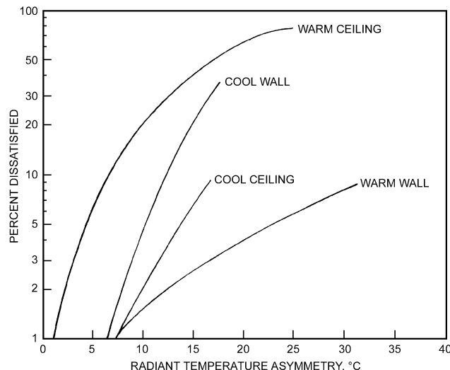
Fig. 6 Percentage of People Expressing Discomfort due to Asymmetric Radiation
