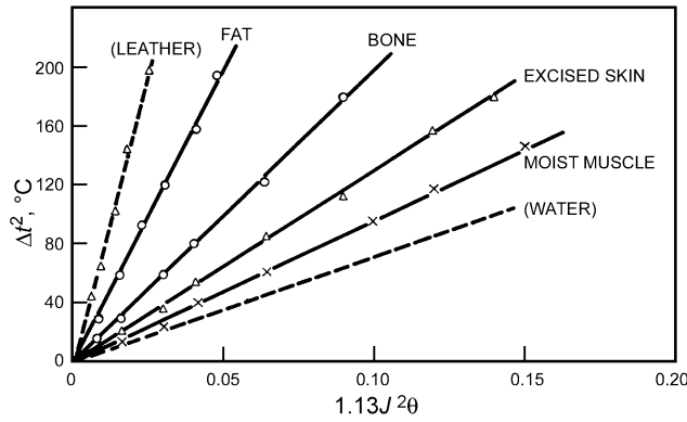
Fig. 19 Comparing Thermal Inertia of Fat, Bone, Moist Muscle, and Excised Skin to That of Leather and Water
