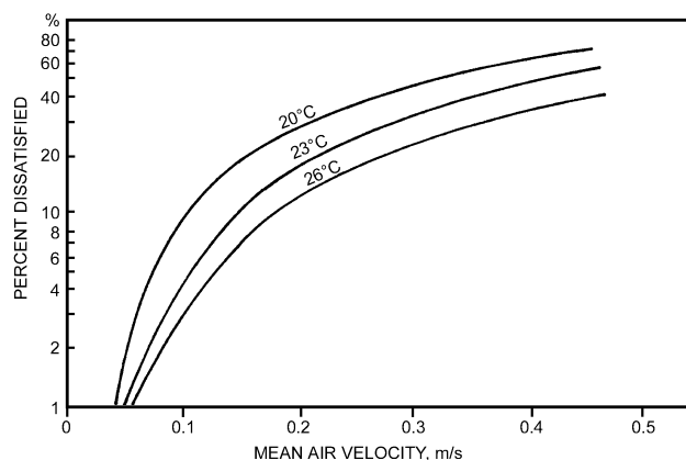
Fig. 7 Percentage of People Dissatisfied as Function of Mean Air Velocity
