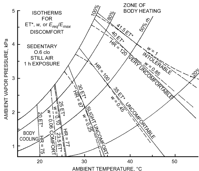
Fig. 15 Effect of Thermal Environment on Discomfort
