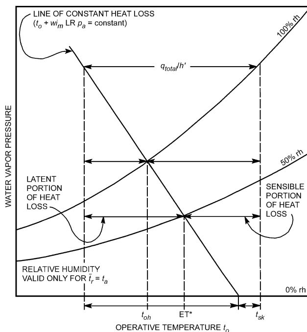
Fig. 2 Constant Skin Heat Loss Line and Its Relationship to t_{oh} and ET^*
