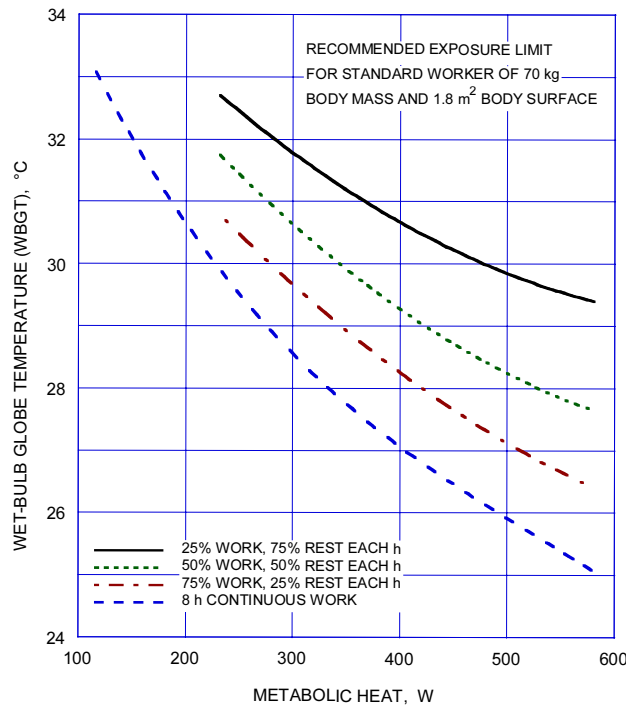
Fig. 17 Recommended Heat Stress Exposure Limits for Heat Acclimatized Workers [Adapted from NIOSH (1986)]
