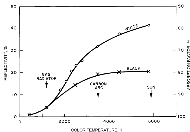
Fig. 18 Variation in Skin Reflection and Absorptivity for Blackbody Heat Sources
