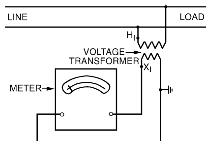
Fig. 18 Voltmeter with Potential Transformer
