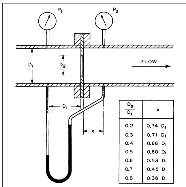
Fig. 9 Sharp Edge Orifice with Pressure Tap Locations From ASME PTC 19.5. Reprinted with permission of ASME.
