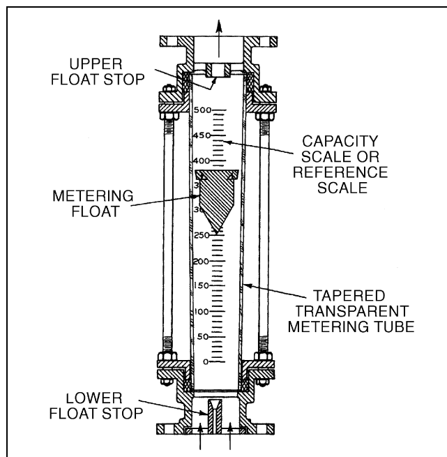
Fig. 10 Variable Area Flowmeter
