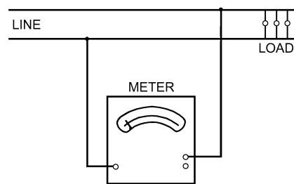
Fig. 17 Voltmeter Connected Across Load
