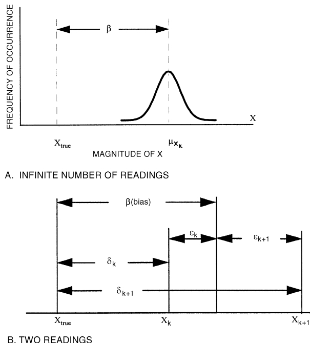
Fig. 1 Errors in the Measurement of a Variable X
