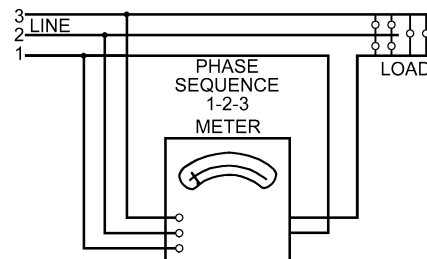
Fig. 25 Three-Wire, Three-Phase Power-Factor Meter
