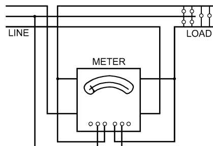
Fig. 23 Polyphase Wattmeter in Three-Phase, Three-Wire Circuit
