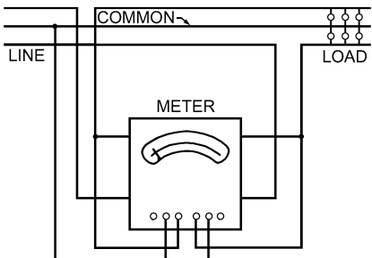
Fig. 22 Polyphase Wattmeter in Two-Phase, Three-Wire Circuit with Balanced or Unbalanced Voltage or Load
