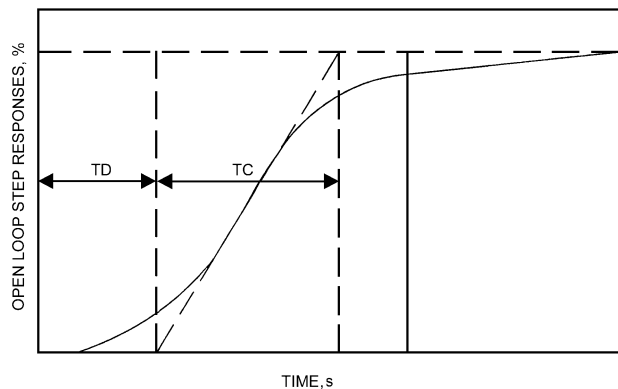
Fig. 26 Open Loop Step Response Versus Time
