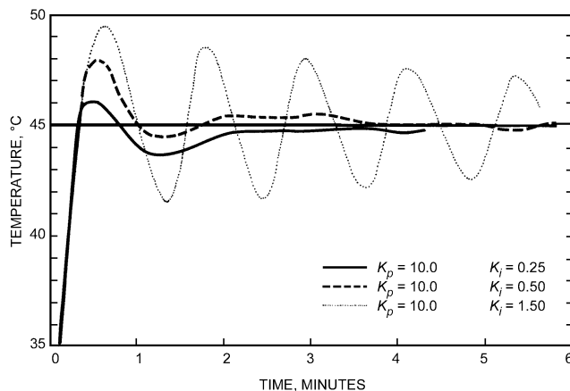
Fig. 27 Response of Discharge Air Temperature to Step Change in Set Points at Various Integral Constants with Fixed Proportional Constant
