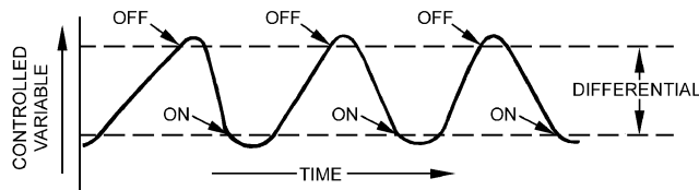
Fig. 4 Two-Position Control
