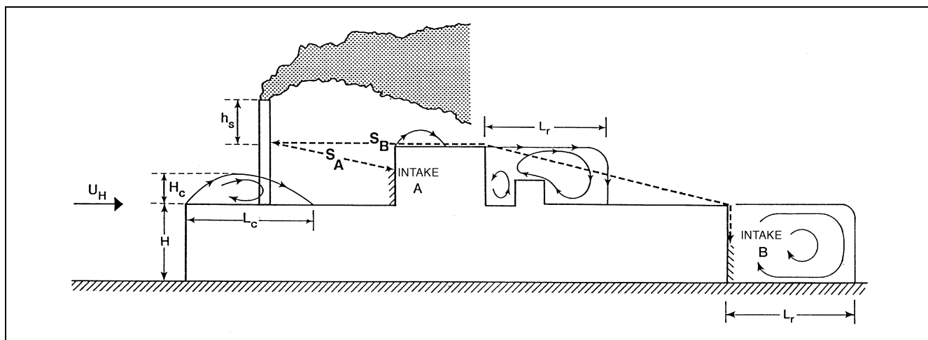
Fig. 3 Flow Recirculation Regions and Exhaust-to-Intake Stretched-String Distances
