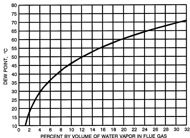
Fig. 2 Water Vapor and Dew Point of Flue Gas
