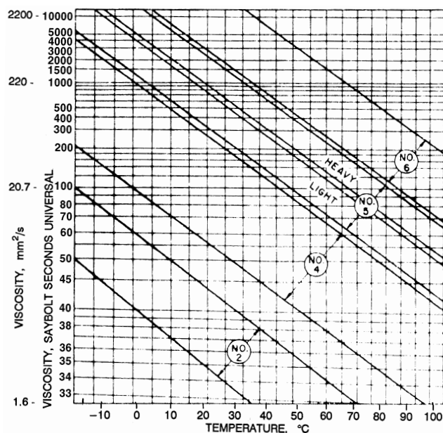
Fig. 1 Approximate Viscosity of Fuel Oils
