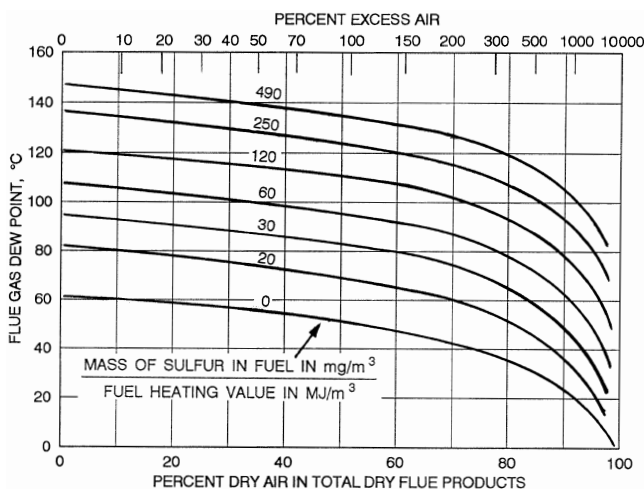
Fig. 4 Influence of Sulfur Oxides on Flue Gas Dew Point (Stone 1969)
