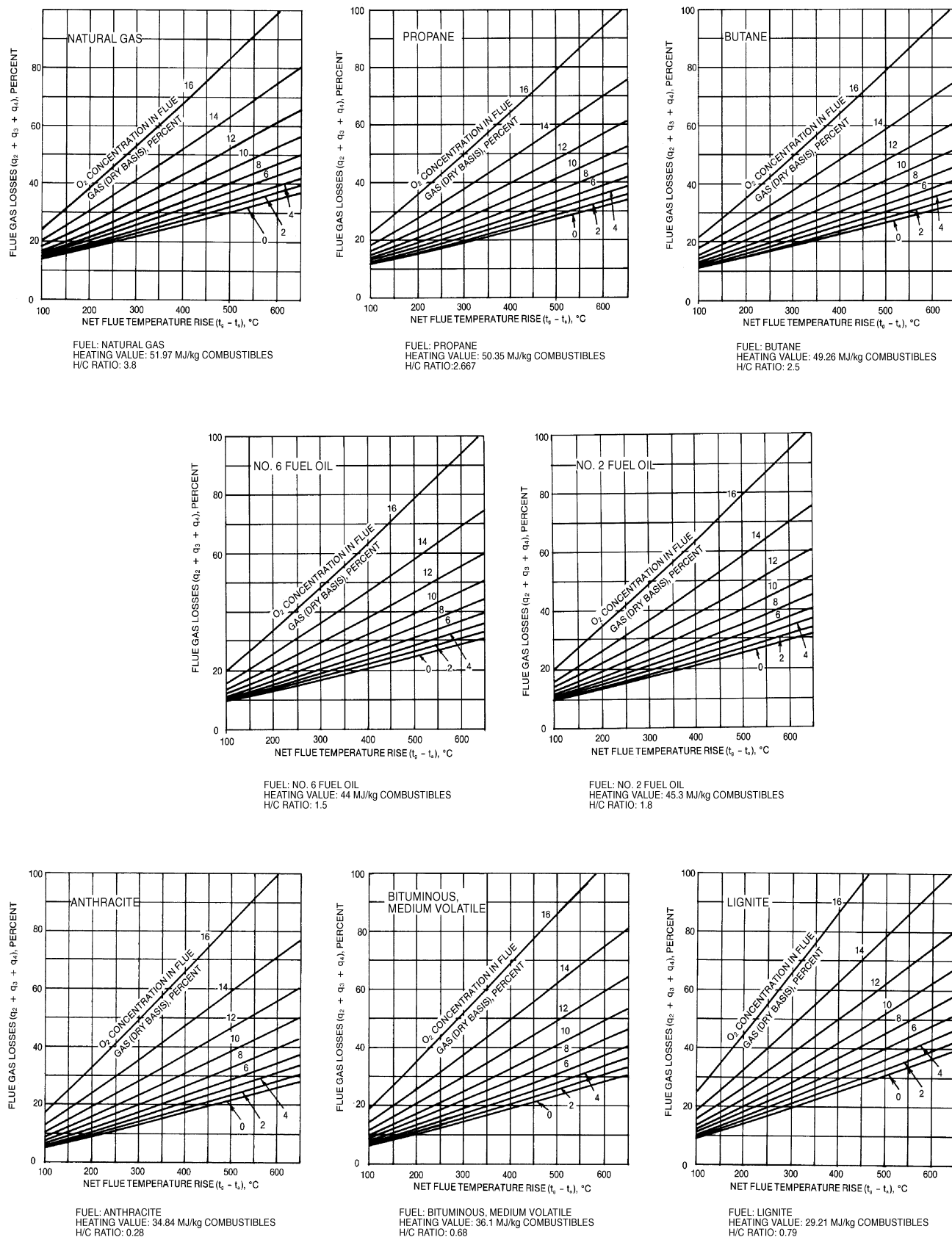
Fig. 5 Flue Gas Losses with Various Fuels (Flue gas temperature rise shown. Loss is based on 18°C room temperature.)
