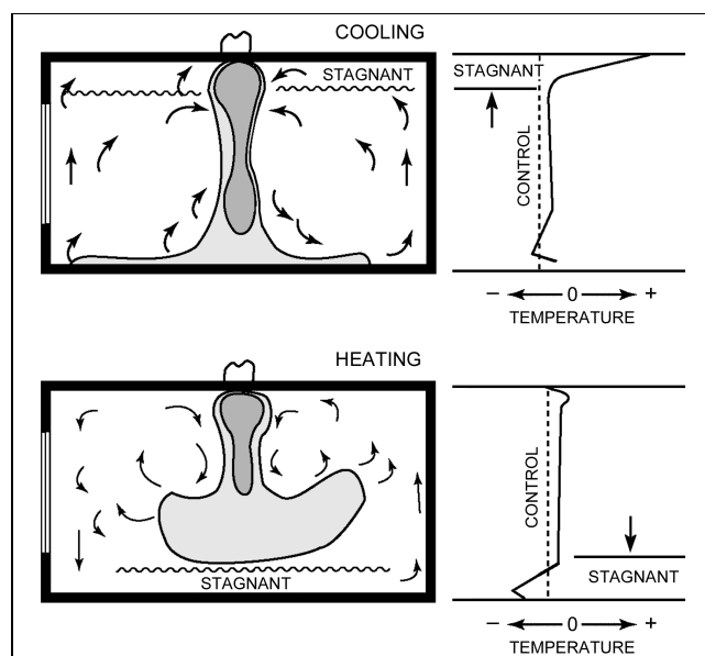
Fig. 8 Air Motion Characteristics of Group E Outlets (Straub et al. 1956)
