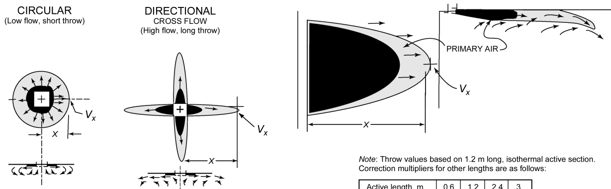
D. CEILING DIFFUSERS
