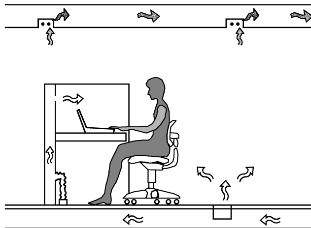
Fig. 11 Underfloor TAC and Personal HVAC System (Matsunawa et al. 1995)
