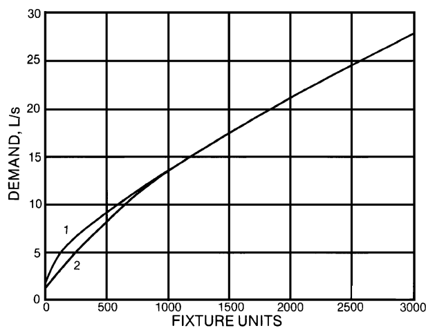
Fig. 5 Demand Versus Fixture Units, Mixed System, High Part of Curve (Hunter 1941)
