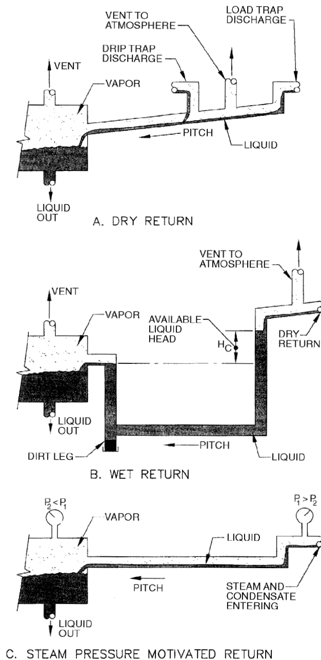
Fig. 12 Types of Condensate Return Systems
