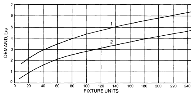
Fig. 6 Estimate Curves for Demand Load (Hunter 1941)
