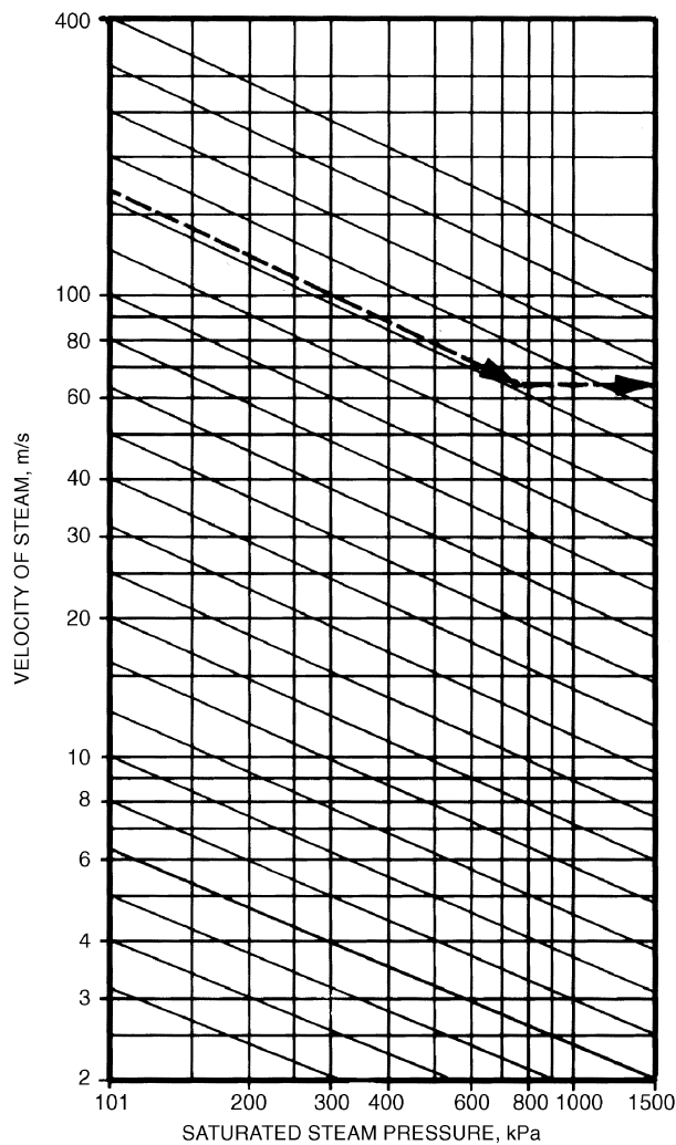
Fig. 11 Velocity Multiplier Chart for Figure 10
