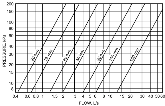
Fig. 8 Pressure Losses in Disk-Type Water Meters
