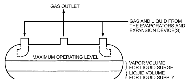
Fig. 8 Basic Horizontal Gas-and-Liquid Separator
