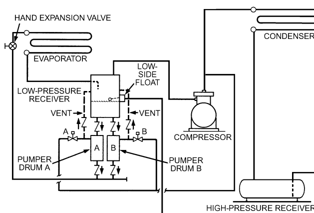
Fig. 3 Double Pumper Drum System
