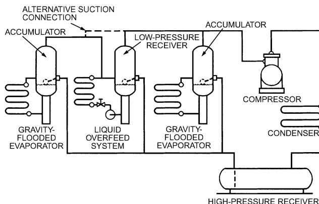
Fig. 5 Liquid Overfeed System Connected on Common System with Gravity-Flooded Evaporators
