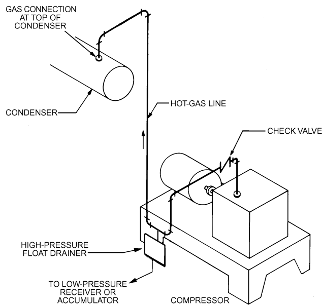
Fig. 7 Hot-Gas Loop
