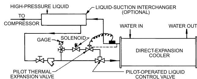
Fig. 21 Direct-Expansion Cooler with Pilot-Operated Control Valve
