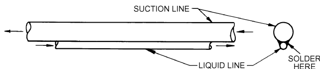
Fig. 27 Soldered Tube Heat Exchanger
