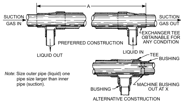
Fig. 30 Tube-in-Tube Heat Exchanger
