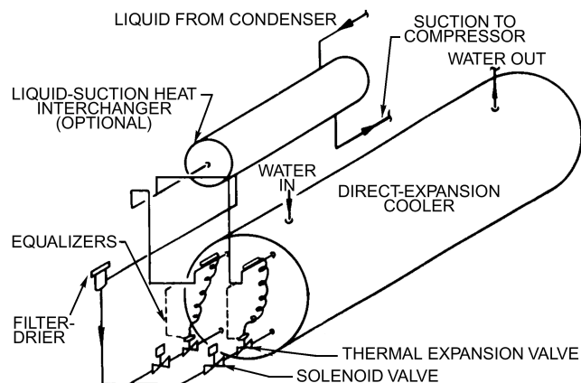
Fig. 19 Two-Circuit Direct-Expansion Cooler Connections (for Single-Compressor System)
