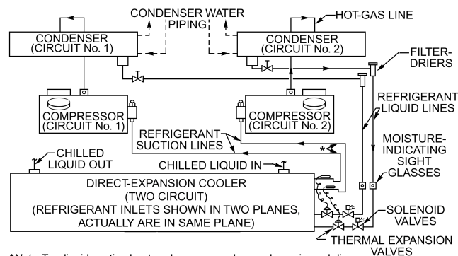
Fig. 20 Typical Refrigerant Piping in Liquid Chilling Package with Two Completely Separate Circuits
