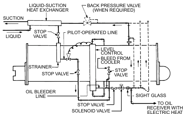
Fig. 18 Typical Piping at Flooded Fluid Cooler
