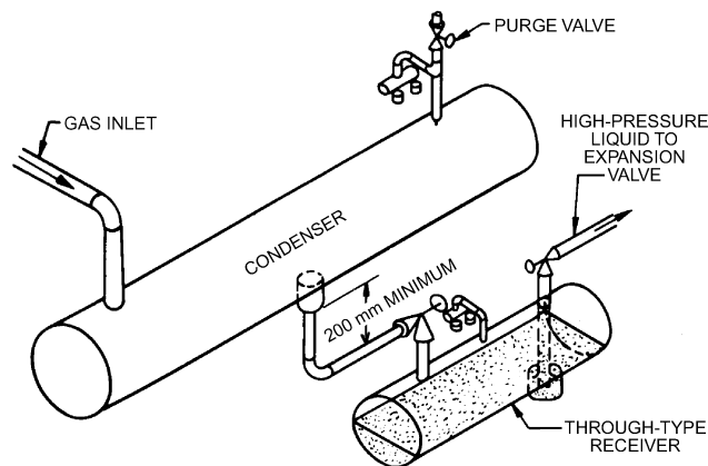
Fig. 8 Shell-and-Tube Condenser to Receiver Piping (Through-Type Receiver)
