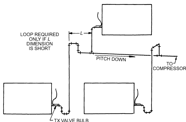
Fig. 5 Typical Piping from Evaporators Located above and below Common Suction Line
