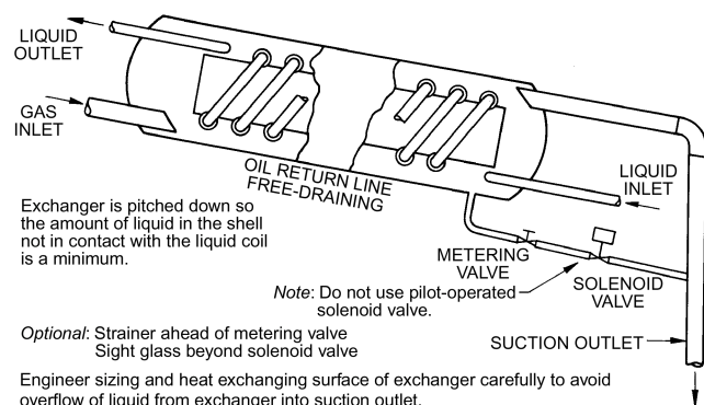
Fig. 29 Shell-and-Finned-Coil Exchanger Installed to Prevent Liquid Floedback
