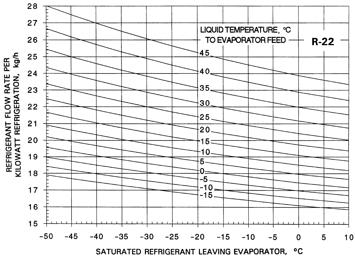
Fig. 1 Flow Rate per Kilowatt of Refrigeration for Refrigerant 22
