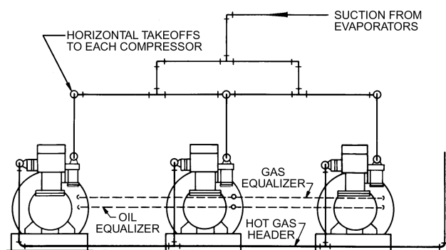
Fig. 15 Suction and Hot-Gas Headers for Multiple Compressors
