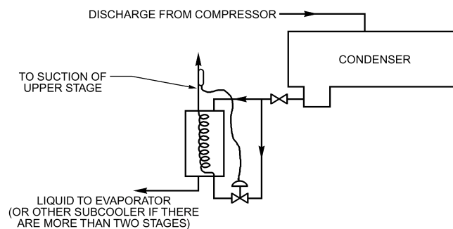
Fig. 32 Closed-Type Subcooler
