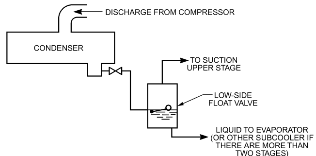
Fig. 31 Flash-Type Cooler
