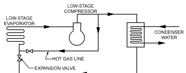
Fig. 12 Hot-Gas Injection Evaporator for Operations at Low Load
