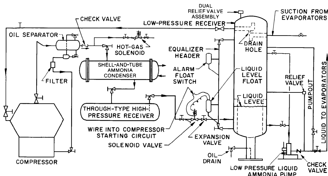
Fig. 41 Piping for Single-Stage System with Low-Pressure Receiver and Liquid Ammonia Recirculation
