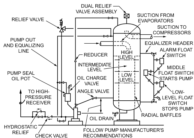
Fig. 8 Piping for Vertical Suction Trap and High-Head Pump
