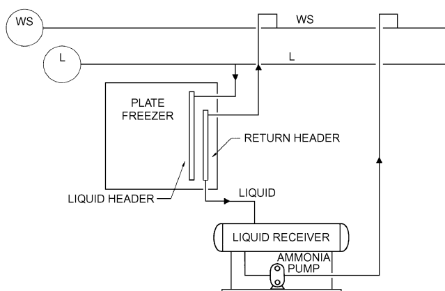
Fig. 48 Recirculated Liquid Return System
