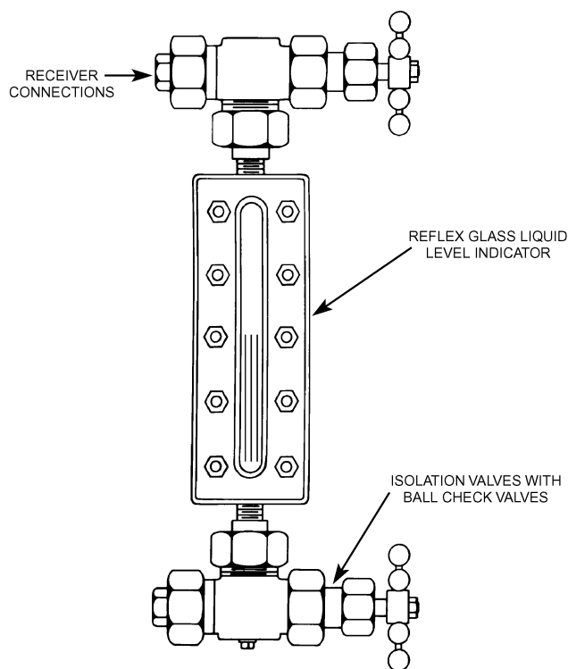
Fig. 9 Gage Glass Assembly for Ammonia
