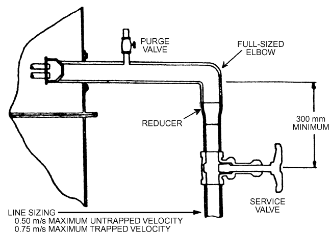
Fig. 32 Method of Reducing Condenser Outlet Sizes
