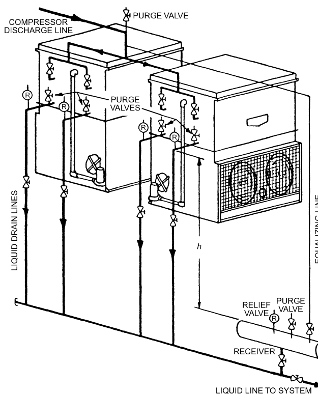
Fig. 34 Piping for Parallel Condensers with Surge-Type Receiver
