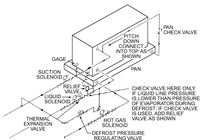
Fig. 36 Piping for Thermostatic Expansion Valve Application for Automatic Defrost on Unit Cooler
