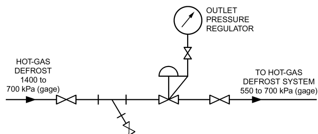
Fig. 44 Equipment Room Hot-Gas Pressure Control System
