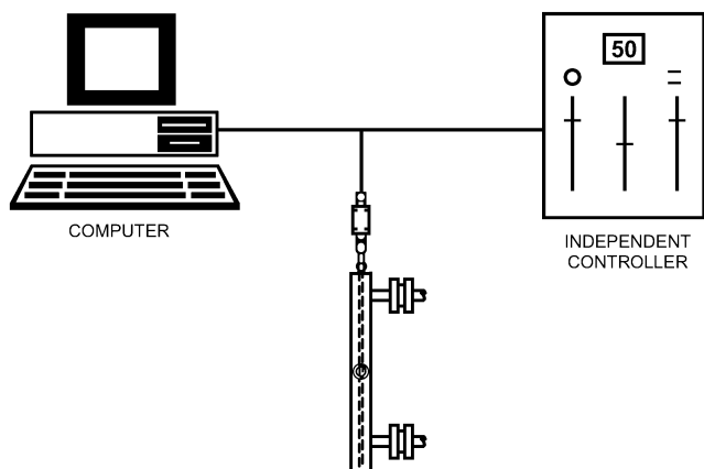
Fig. 10 Electronic Liquid Level Control
