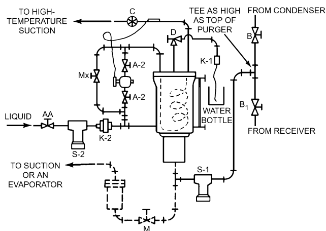
Fig. 11 Purge Unit and Piping for Noncondensable Gas
