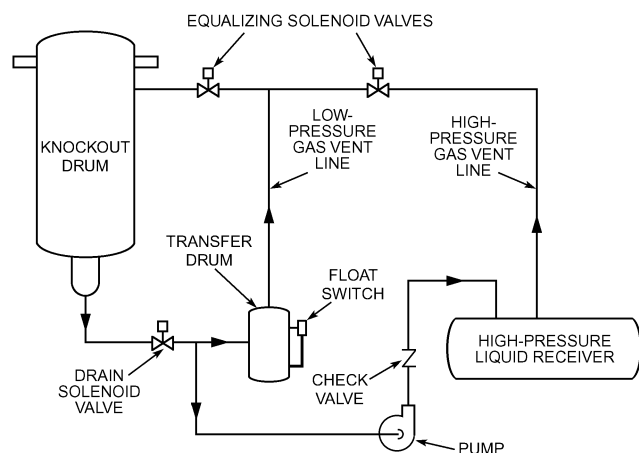
Fig. 6 Equalized Pressure Pump Transfer System
