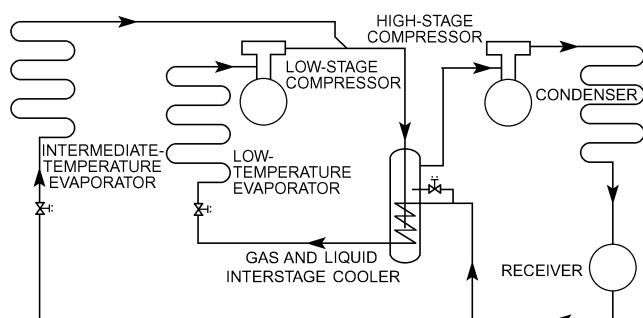
Fig. 2 Two-Stage System with High- and Low-Temperature Loads
