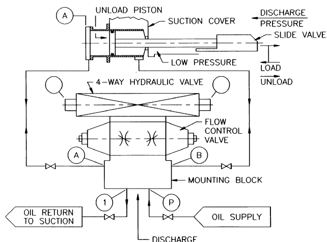
Fig. 25 Typical Hydraulic System for Slide Valve Capacity Control for Screw Compressor with Fixed V_i
