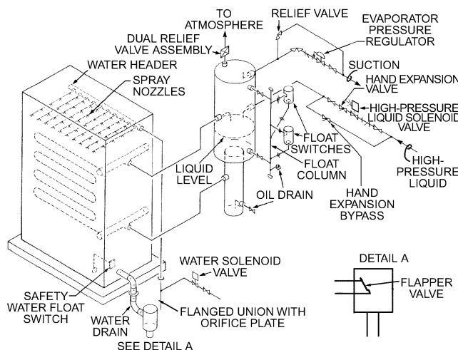
Fig. 37 Arrangement for Automatic Defrost of Air Blower with Flooded Coil
