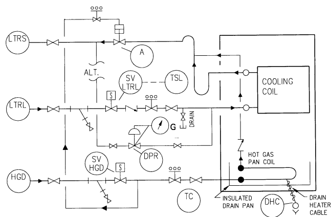
UPFEED COILS
