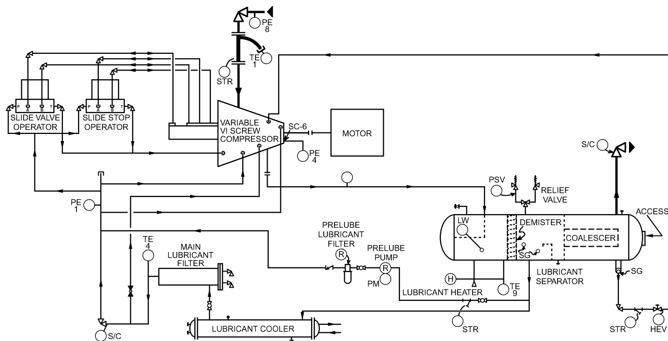
Fig. 20 Flow Diagram for Variable V_i Screw Compressor High-Stage Only
