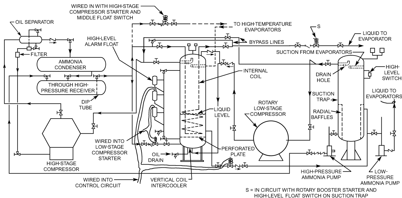
Fig. 4 Arrangement for Compound System with Vertical Intercooler and Suction Trap
