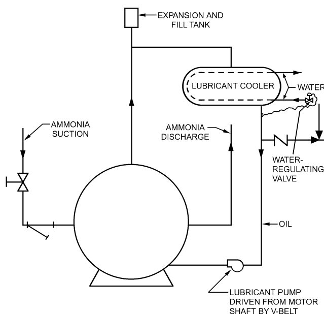
Fig. 17 Rotary Vane Booster Compressor Cooling with Lubricant
