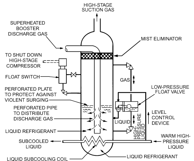
Fig. 3 Intercooler
