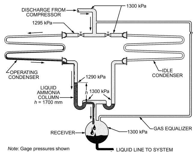
Fig. 31 Two Evaporative Condensers with Trapped Piping to Receiver
