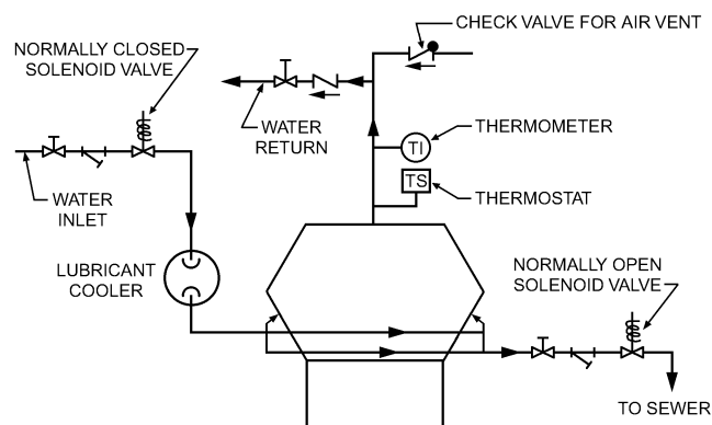
Fig. 16 Jacket Water Cooling for Ambient Temperatures Below Freezing
