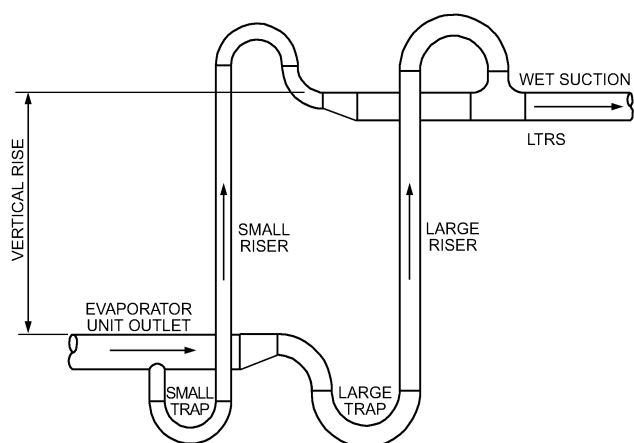
Fig. 47 Double Low-Temperature Suction Risers
