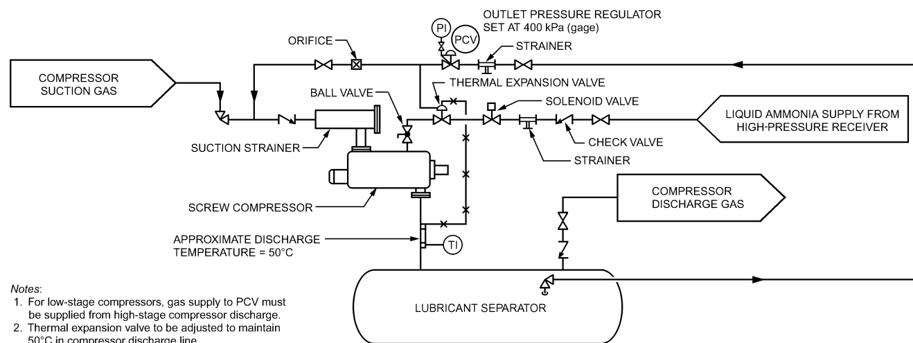
Fig. 21 Flow Diagram for Screw Compressors with Refrigerant Injection Cooling
