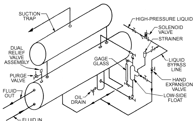
Fig. 39 Piping for Evaporator and Low-Side Float with Horizontal Liquid Cooler
