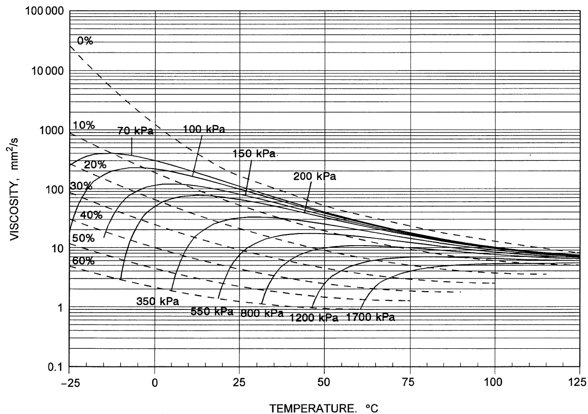
Fig. 40 Viscosity-Temperature-Pressure Plot for 80 ISO VG Polyoxypolypropylene Diol with R-134a
