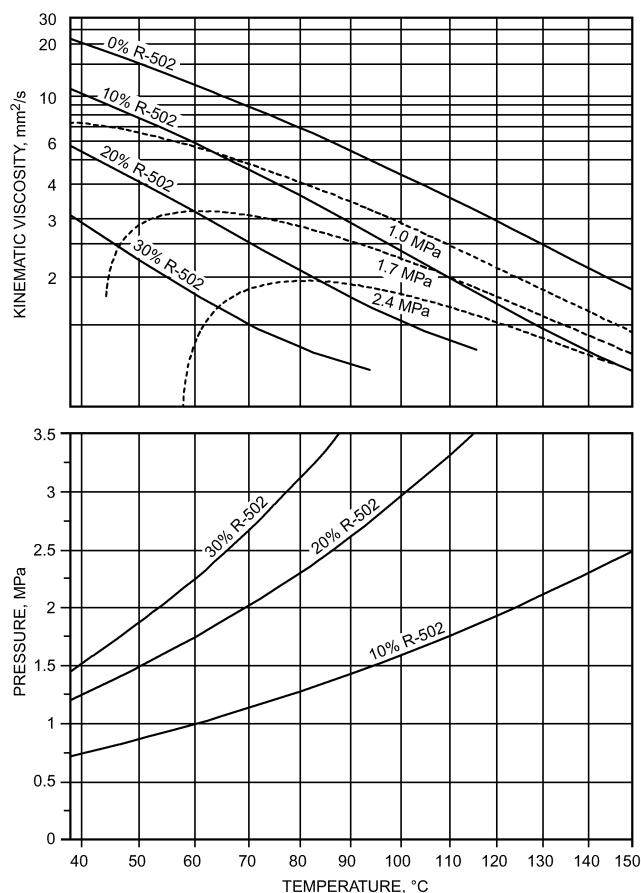
Fig. 36 Viscosity-Temperature-Pressure Chart for Solutions of R-502 in 32 mm 2 /s Naphthenic Oil
