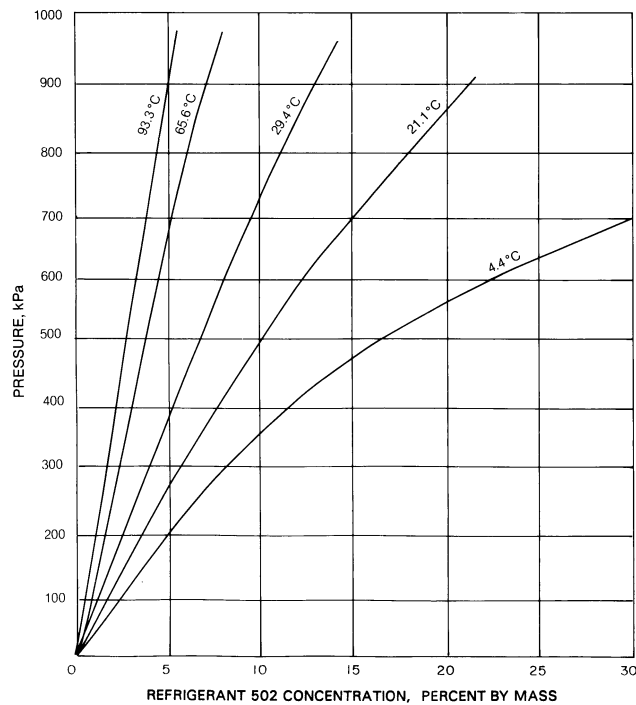
Fig. 24 Solubility of R-502 in 32 Naphthenic Oil ( C_A 12%, C_N 44%, C_P 44%)
