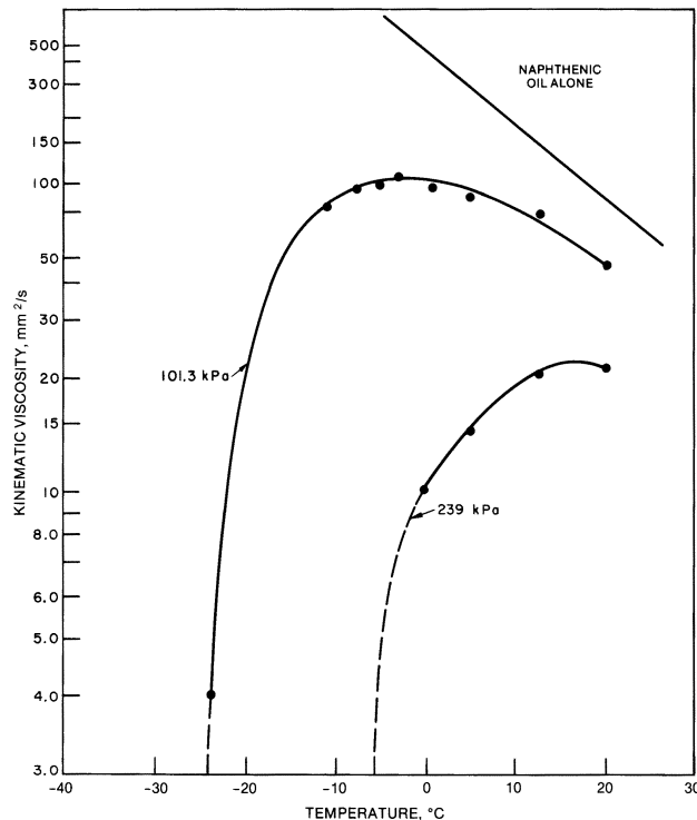
Fig. 32 Viscosity of R-12/Oil Solutions at Low-Side Conditions (Parmelee 1964)
