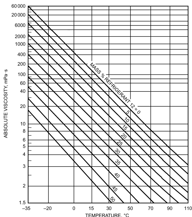
Fig. 28 Viscosity-Temperature Chart for Solutions of R-12 in 32 Naphthene Base Oil
