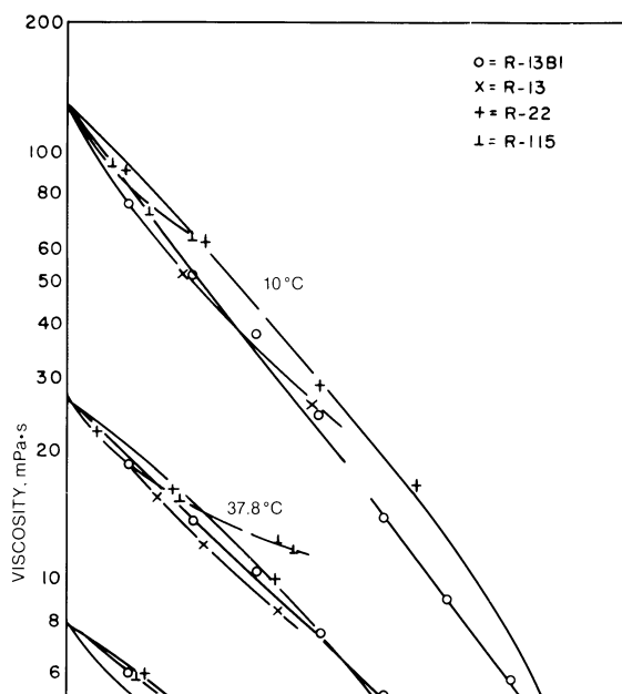
Fig. 14 P-T-S Relations of R-22 with 43 White Oil (0% C_A , 55% C_N , 45% C_P ) (Spauschus 1964)
