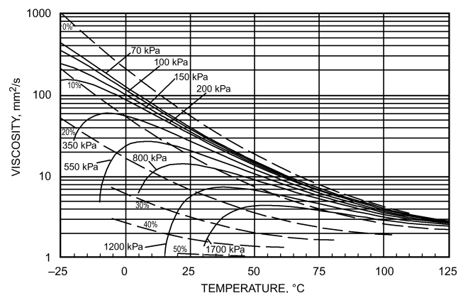
Fig. 45 Viscosity-Temperature-Pressure Plot for a Mixture of R-410A and 32 ISO VG Branched Acid Polyol Ester Lubricant
