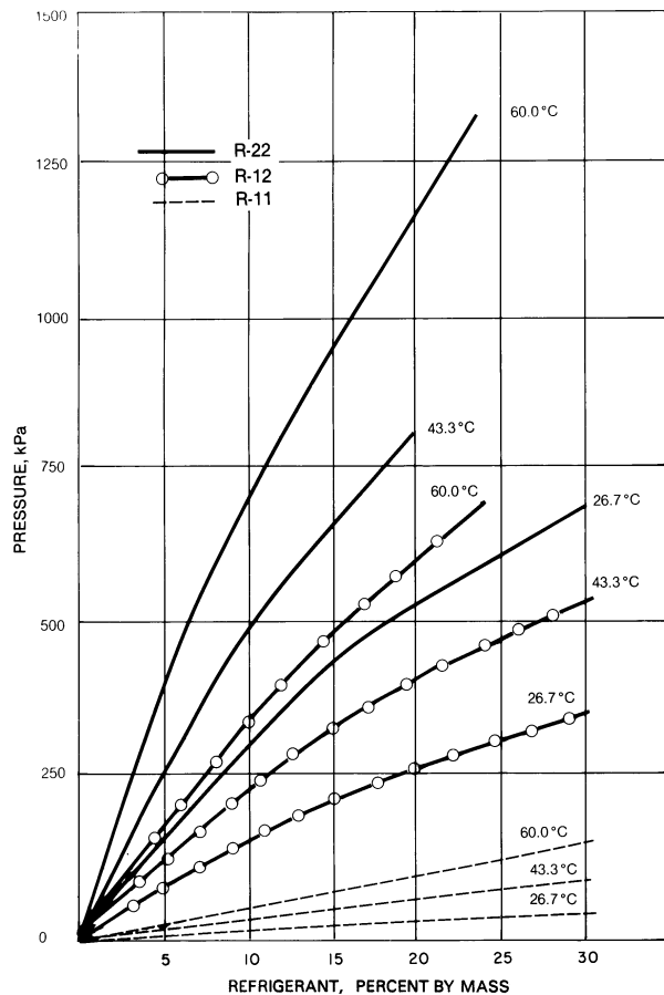
Fig. 31 Solubility of Refrigerants in 32 Alkylbenzene Oil
