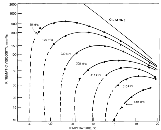
Fig. 34 Viscosity of R-502/Naphthenic Oil Solutions at Low-Side Conditions
