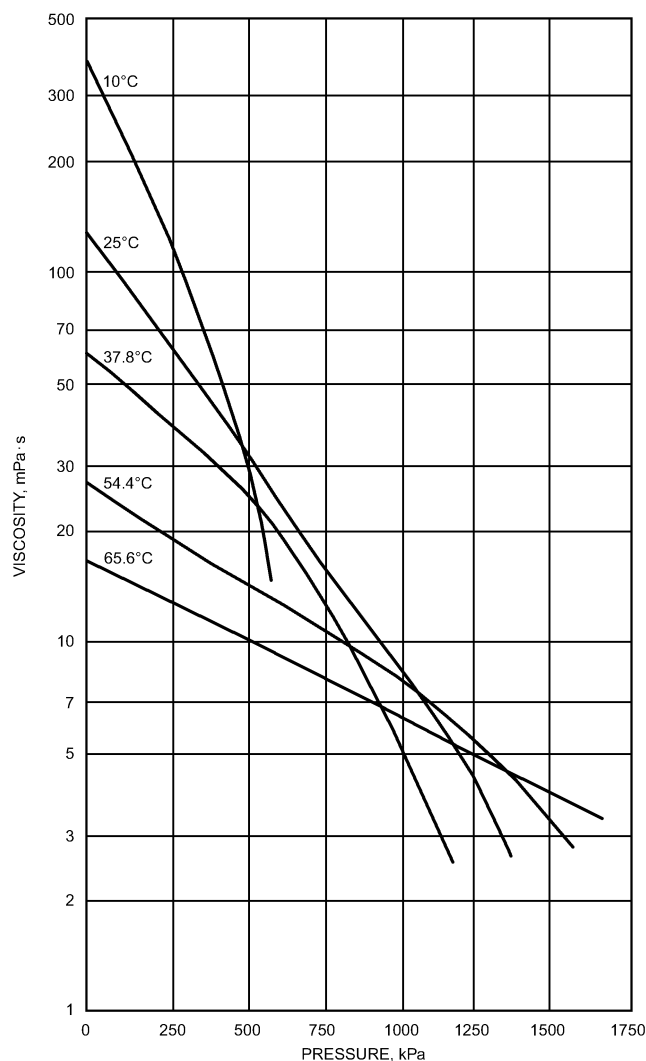
Fig. 23 Viscosity of Mixtures of 65 Paraffin Base Oil and R-22 (Albright and Mandelbaum 1956)
