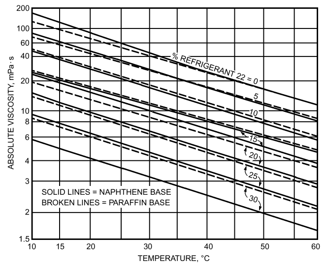
Fig. 20 Viscosity-Temperature Chart for Solutions of R-22 in 32 Naphthene and Paraffin Base Oils
