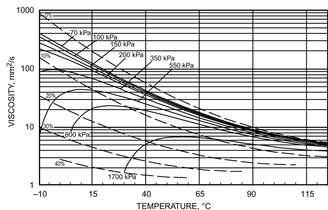
Fig. 44 Viscosity-Temperature-Pressure Plot for a Mixture of R-410A and 68 ISO VG Mixed Acid Polyol Ester Lubricant
