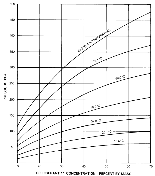
Fig. 26 Solubility of R-11 in 65 Oil
