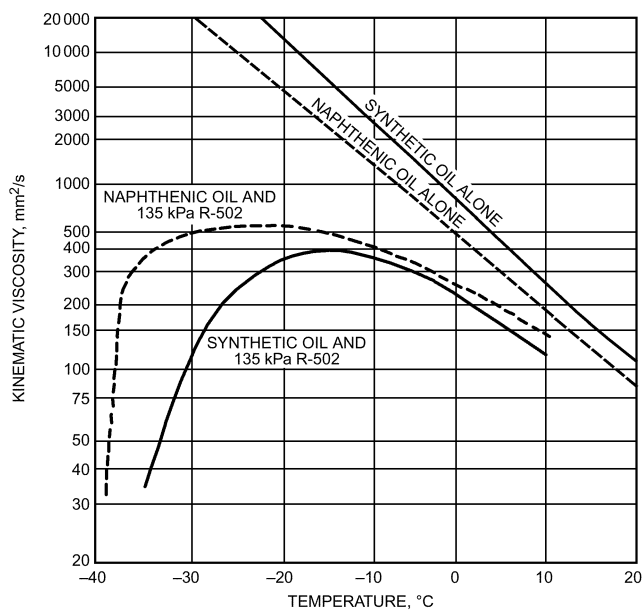
Fig. 35 Viscosities of Solutions of R-502 with 32 mm 2 /s Naphthenic Oil (C A 12%, C N 44%, C P 44%) and 32 mm 2 /s Synthetic Alkylbenzene Oil
