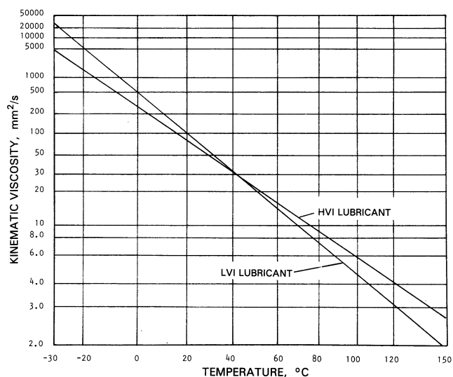
Fig. 1 Viscosity-Temperature Chart for 108 HVI and LVI Lubricants
