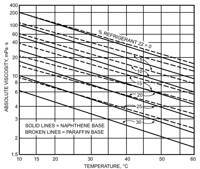
Fig. 21 Viscosity-Temperature Chart for Solutions of R-22 in 65 Naphthene and Paraffin Base Oils
