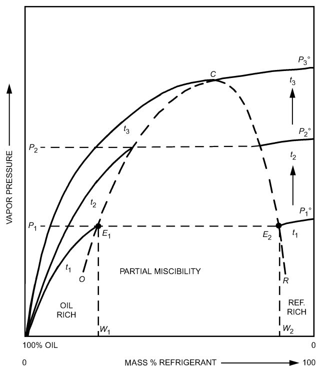
Fig. 13 P-T-S Diagram for Partially Miscible Refrigerant-Oil Solutions
