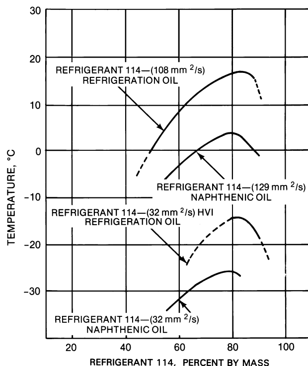
Fig. 29 Critical Solution Temperatures of R-114/Oil Mixtures
