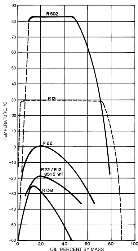
Fig. 15 Critical Solubilities of Refrigerants with 32 Naphthenic Lubricant ( C_A 12%, C_N 44%, C_P 44%)
