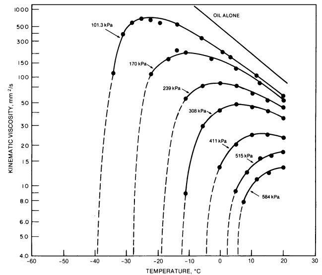
Fig. 33 Viscosity of R-22/Naphthenic Oil Solutions at Low-Side Conditions (Parmelee 1964)
