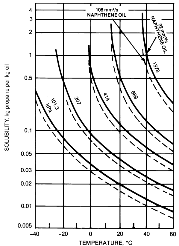
Fig. 51 Solubility of Propane in Oil
