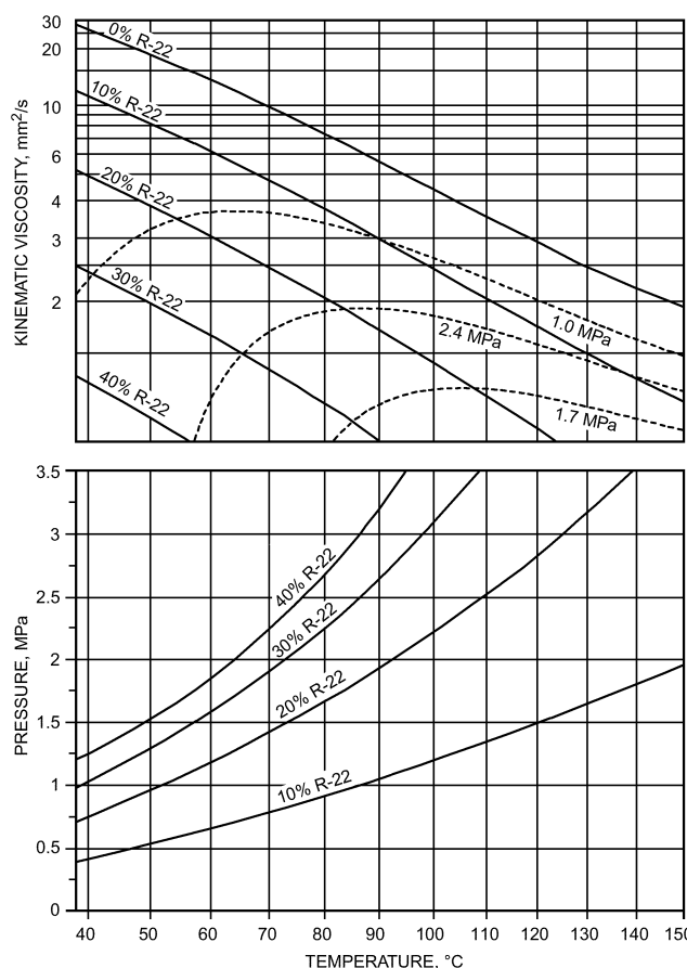
Fig. 37 Viscosity-Temperature-Pressure Chart for Solutions of R-22 in 32 mm 2 /s Alkylbenzene Oil
