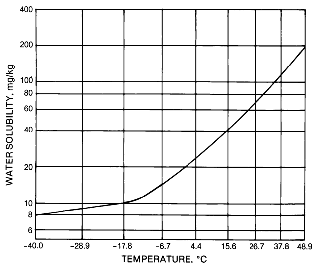
Fig. 53 Solubility of Water in Mineral Oil
