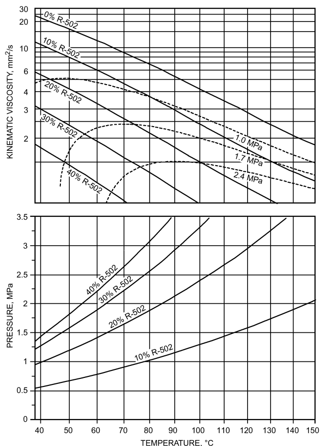
Fig. 38 Viscosity-Temperature-Pressure Chart for Solutions of R-502 in 32 mm 2 /s Alkylbenzene Oil
