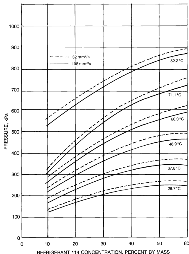
Fig. 30 Solubility of R-114 in HVI Oils
