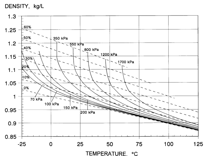
Fig. 5 Density as Function of Temperature and Pressure for Mixture of R-134a and 100 ISO VG Branched Acid Polyol Ester Lubricant
