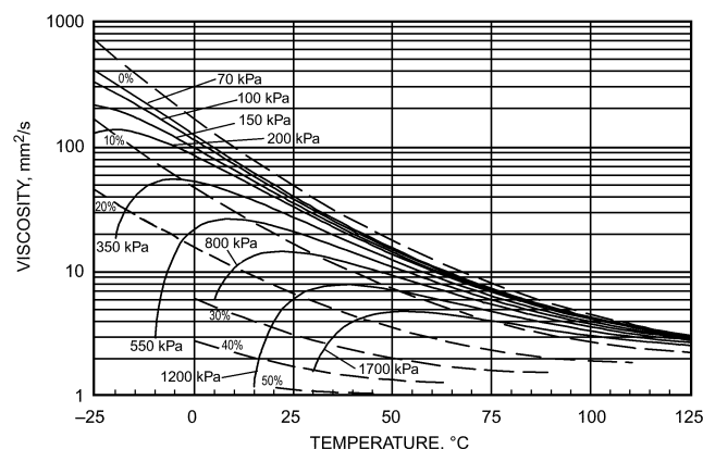
Fig. 43 Viscosity-Temperature-Pressure Plot for a Mixture of R-410A and 32 ISO VG Mixed Acid Polyol Ester Lubricant
