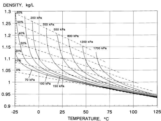
Fig. 4 Density as Function of Temperature and Pressure for Mixture of R-134a and 32 ISO VG Branched Acid Polyol Ester Lubricant
