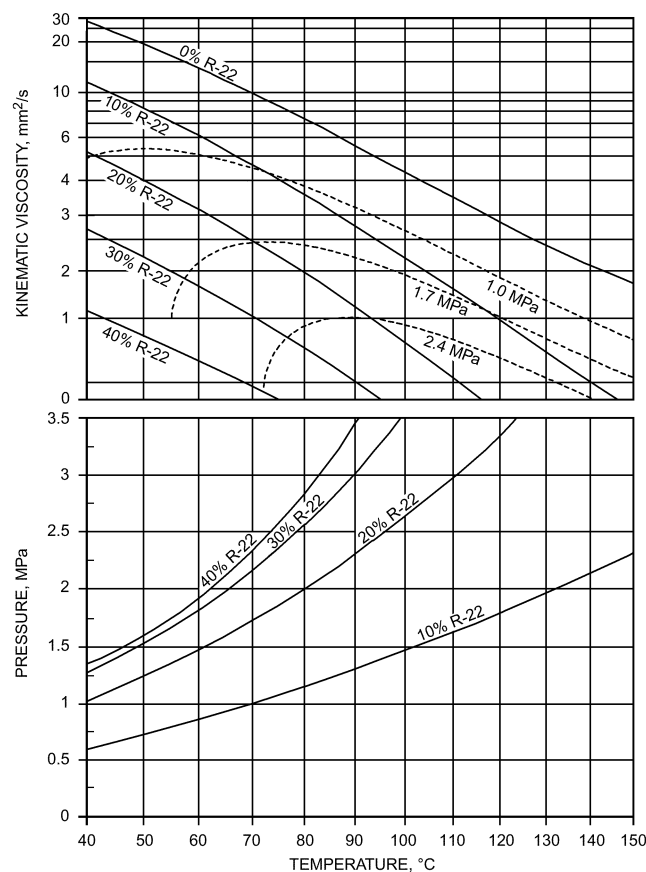
Fig. 22 Viscosity-Temperature Chart for Solutions of R-22 in 32 Naphthenic Oil (Van Gaalen, et al. 1990 and 1991a)
