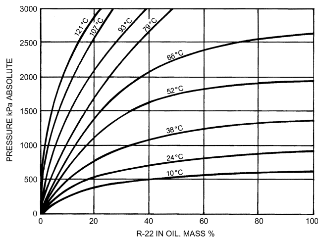
Fig. 19 Solubility of R-22 in 32 Naphthenic Oil
