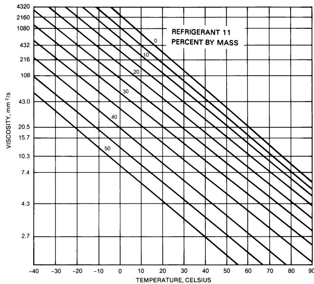
Fig. 25 Viscosity-Temperature Curves for Solutions of R-11 in 65 Naphthene Base Oil
