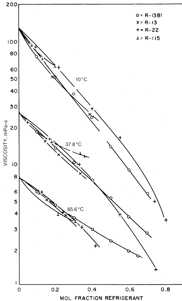
Fig. 18 Viscosity of Mixtures of Various Refrigerants and 32 Paraffinic Oil (Albright and Lawyer 1959)
