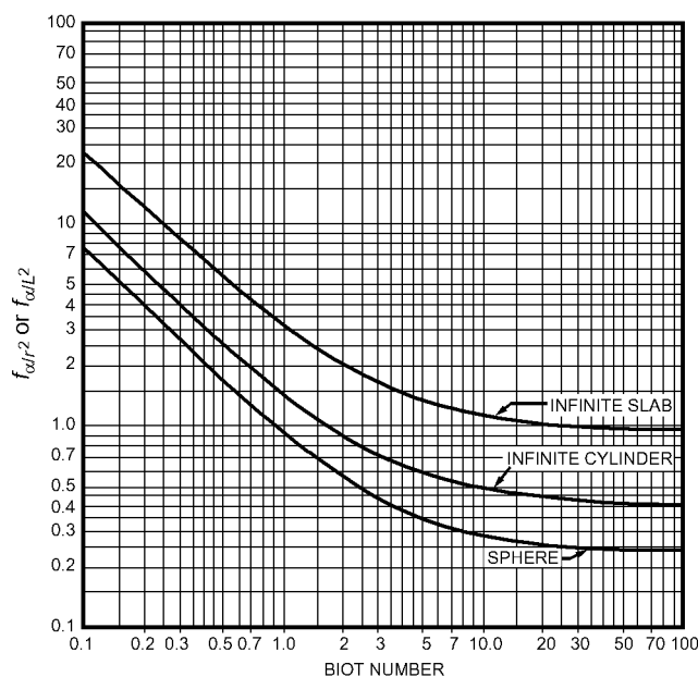
Fig. 2 Relationship Between f_{0.9}/r^2 and Biot Number for Infinite Slab, Infinite Cylinder, and Sphere
