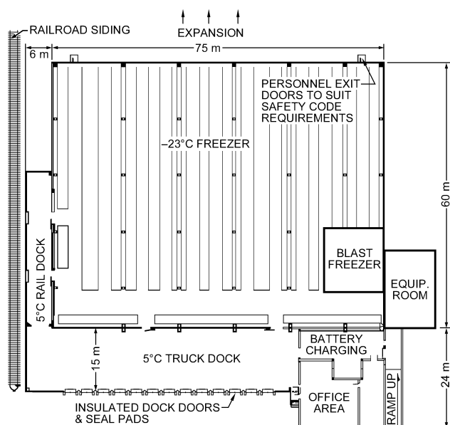
Fig. 1 Typical Plan for One-Story Refrigerated Facility
