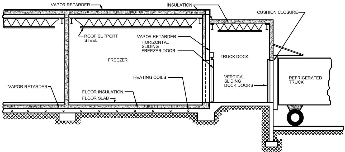
Fig. 9 Typical One-Story Construction with Underfloor Warming Pipes
