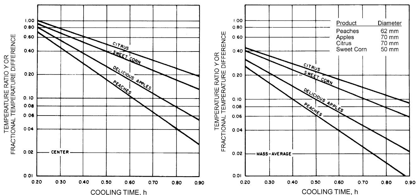
Fig. 2 Time-Temperature Response for Hydrocooled Produce
