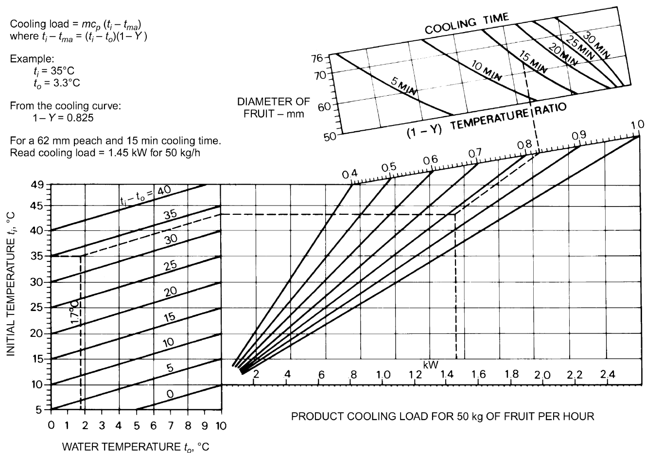
Fig. 1 Nomograph to Determine Product Heat Load of Hydrocooled Peaches
