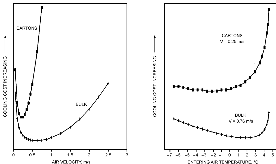
Fig. 4 Engineering-Economic Model Output for a Forced-Air Cooler
