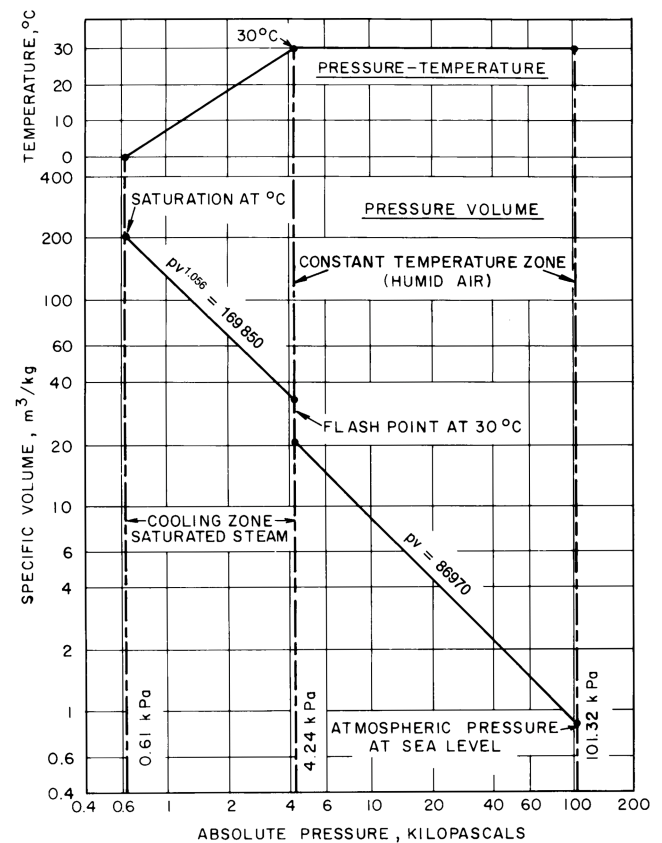
Fig. 5 Pressure, Volume, and Temperature in a Vacuum Cooler Cooling Product from
