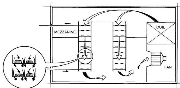
Fig. 8 Vertical Airflow Spiral Freezer
