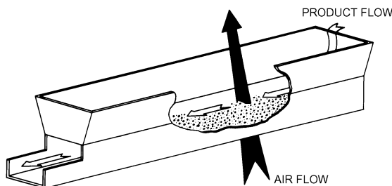
Fig. 6 Fluidized Bed Freezer
