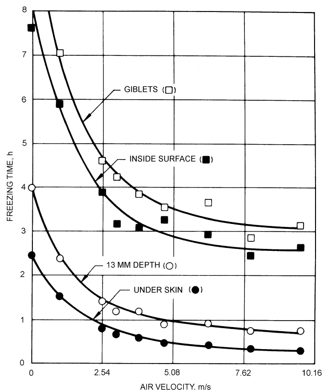
Fig. 11 Relation Between Freezing Time and Air Velocity (van den Berg and Lentz 1958)
