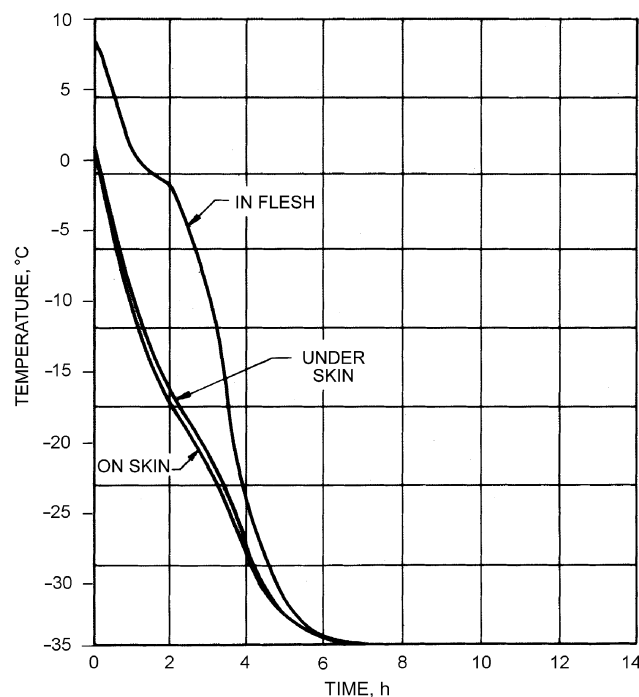
Fig. 13 Temperature During Freezing of Packaged, Ready-to-Cook Turkeys (Klose and Pool 1956)
