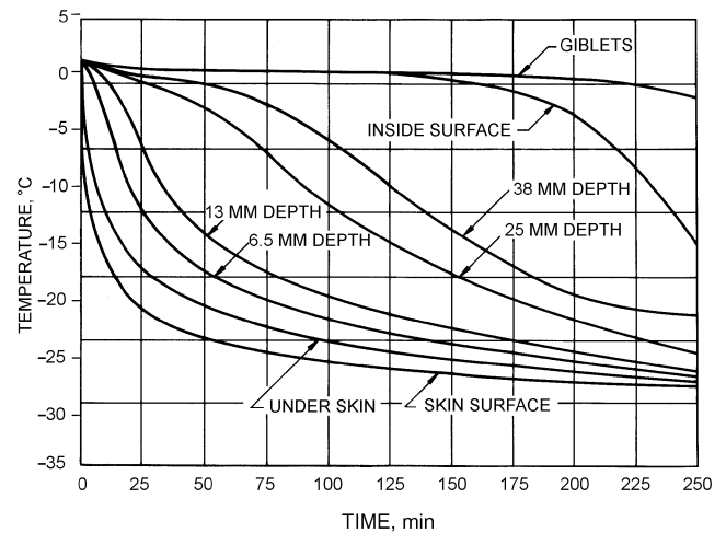
Fig. 14 Temperatures at Various Depths in Breast of 6.8 kg Turkeys During Immersion Freezing at -30°C (Lentz and van den Berg 1957)
