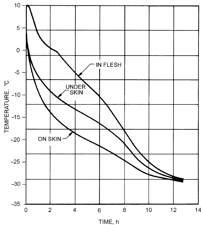
Fig. 12 Temperature During Freezing of Packaged, Ready-to-Cook Turkeys (Klose and Pool 1956)
