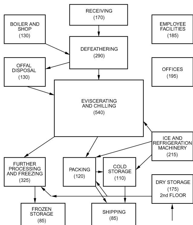
Fig. 4 Space-Relationship-Flow Diagram for Poultry Processing Plant (square metres of floor space needed)
