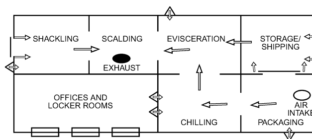
Fig. 15 Air Movement Pattern in Positively-Pressurized Poultry Processing Plant (further processing is not included) (Source: Keener 2000)
