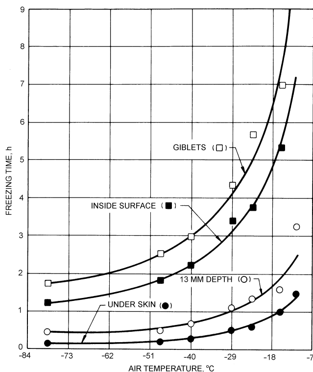
Fig. 10 Relation Between Poultry Freezing Time and Air Temperature (van den Berg and Lentz 1958)
