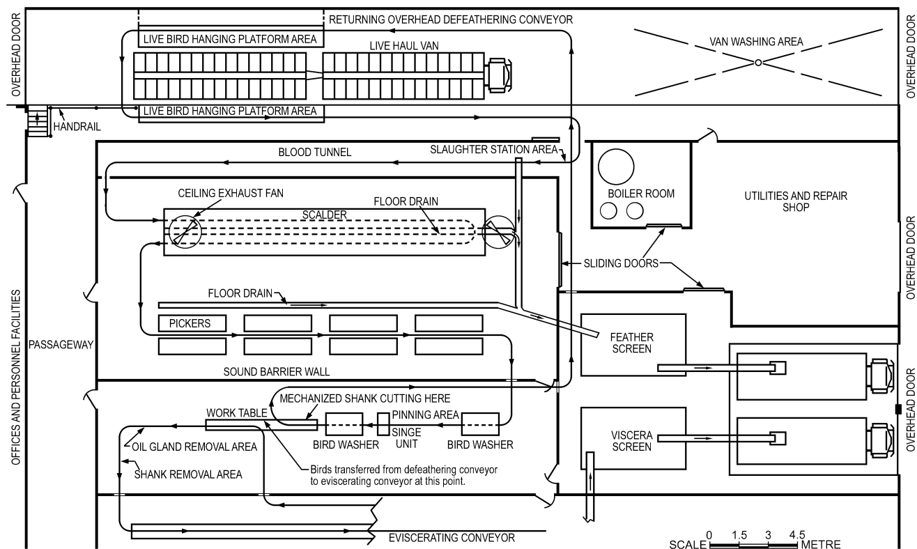
Fig. 2 Equipment Layout for Live Bird Recieving, Slaughtering, and Defeathering Areas
