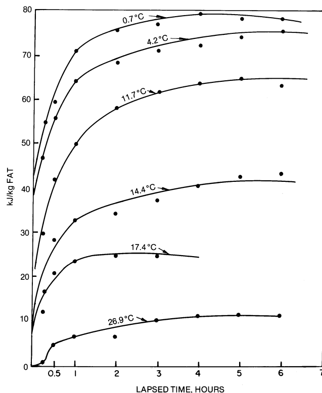
Fig. 3 Heat Liberated from Fat in Cream Cooled Rapidly from Approximately 30°C to Various Temperatures (Rishoi 1951)
