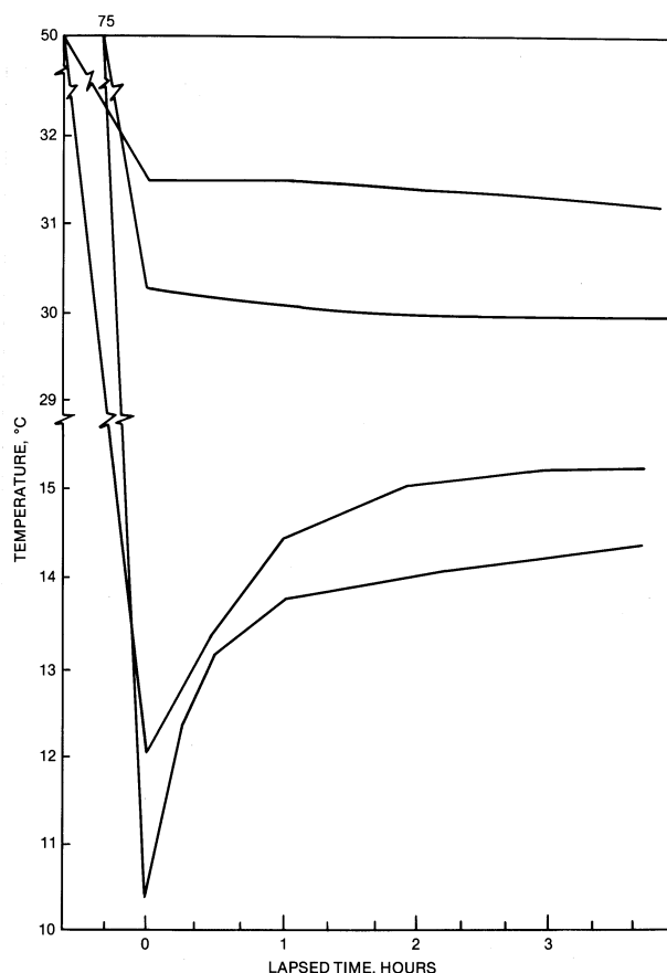
Fig. 2 Thermal Behavior of Cream Heated to 75°C Followed by Rapid Cooling to 30°C and to 10.4°C; Comparison with Cream Heated to 50°C, then Rapid Cooling to 31.4°C and to 12°C
