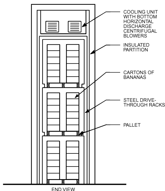
Fig. 3 Three-Tier Forklift Banana Room (End View)
