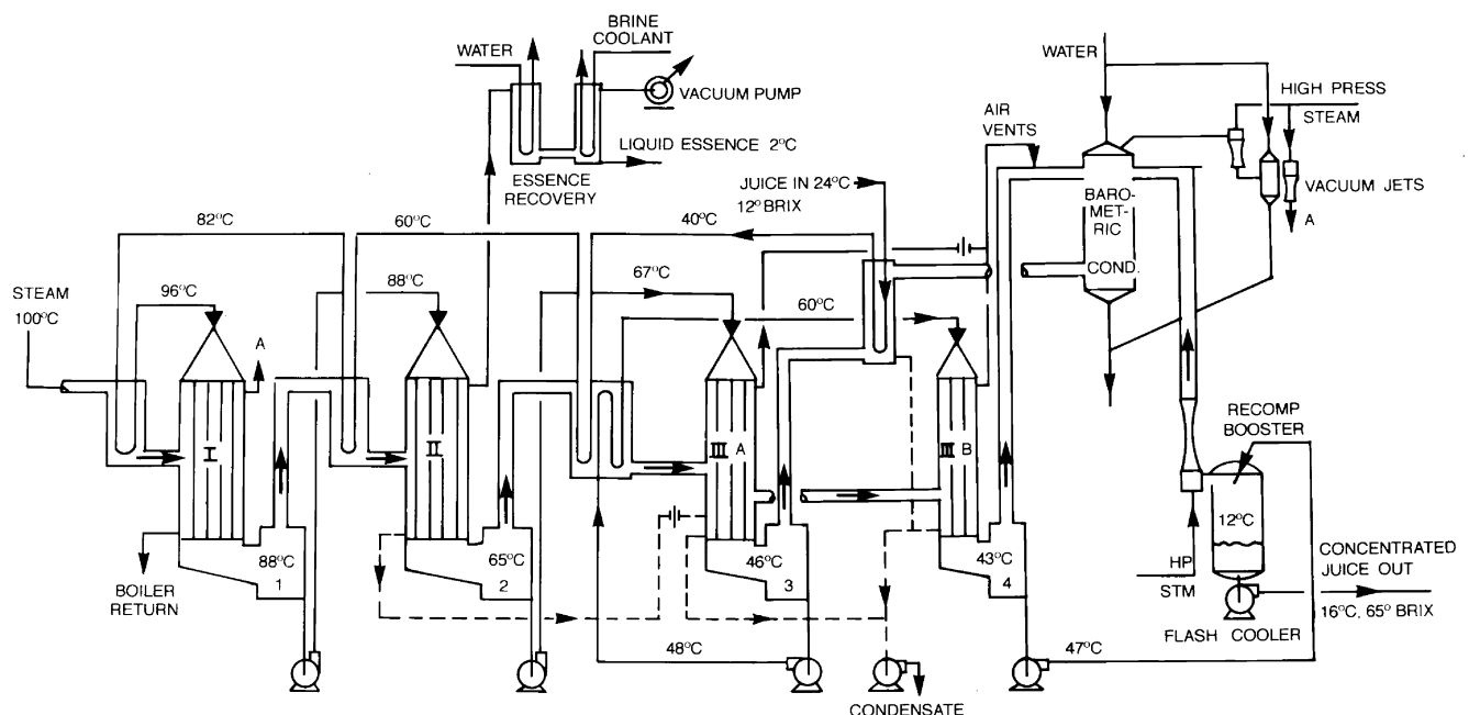
Fig. 2 Thermally Accelerated Short-Time Evaporator (TASTE) Schematic
