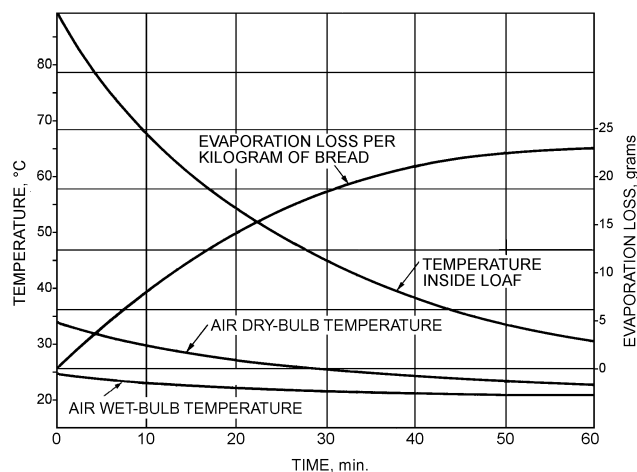
Fig. 1 Moisture Loss and Air Temperature Rise in Counterflow Bread-Cooling Tunnel
