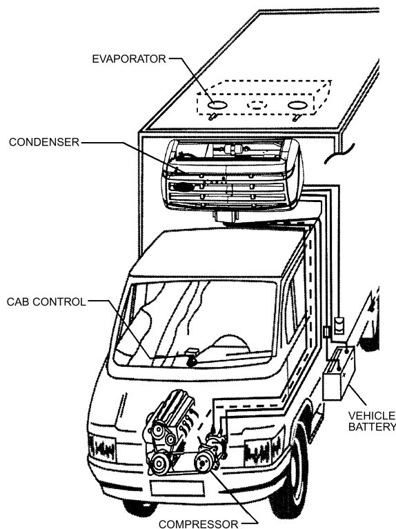
Fig. 7 Small Truck Refrigeration System
