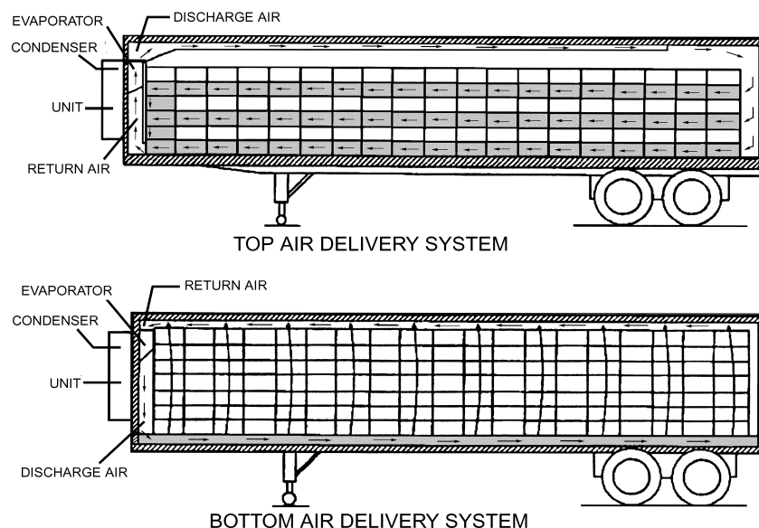
Fig. 4 Sections of Vehicle Showing Air Circulation
