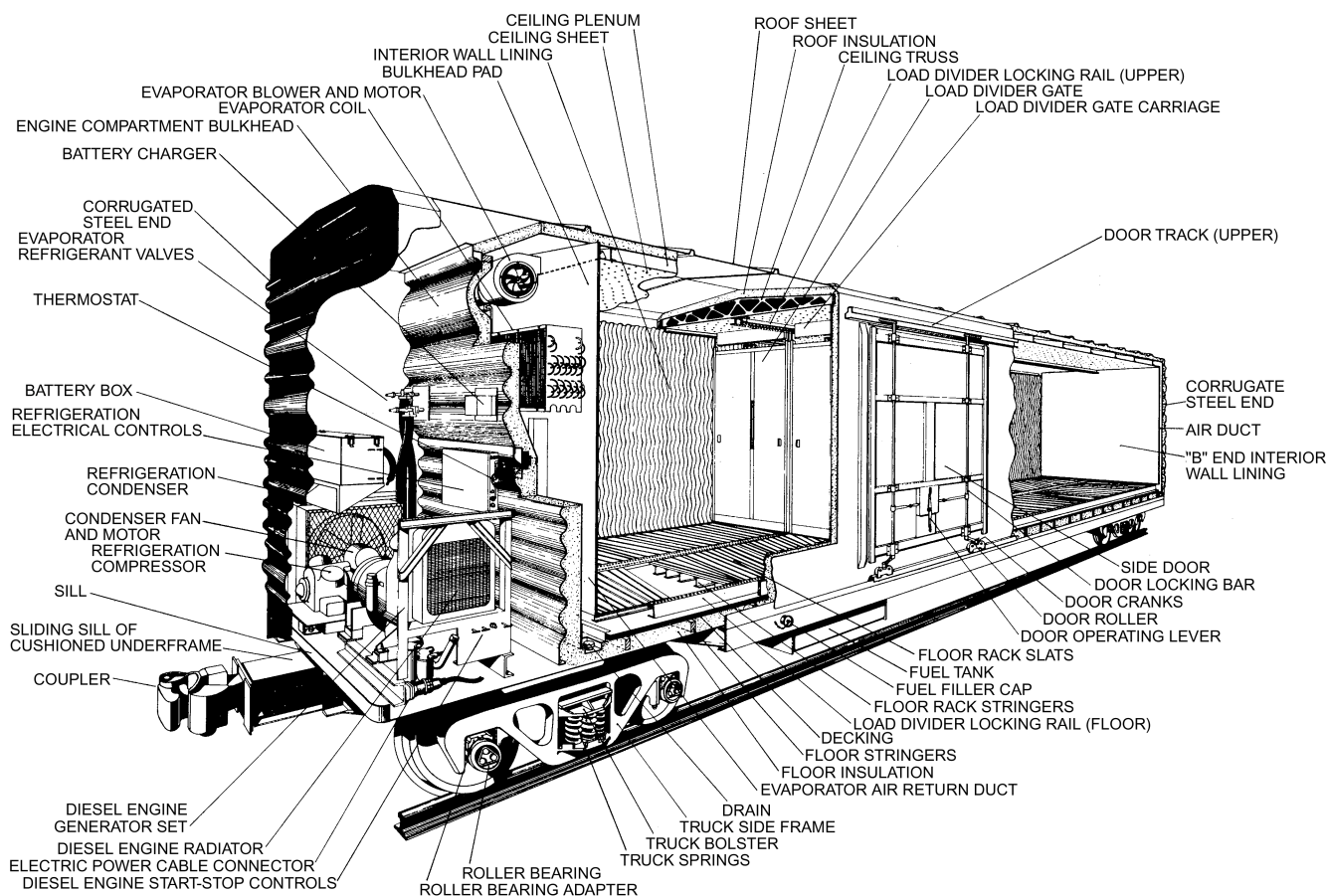
Fig. 2 Mechanical Railway Refrigerator Car
