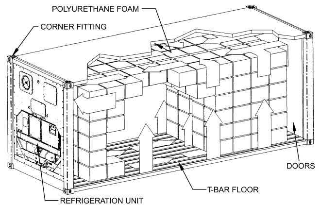
Fig. 1 Refrigerated Cargo Container
