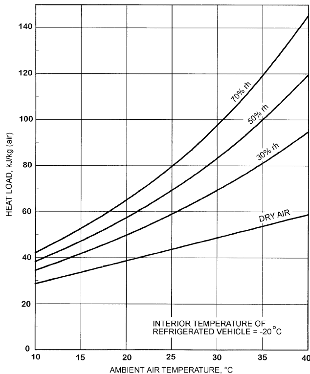
Fig. 3 Heat Load from Air Leakage
