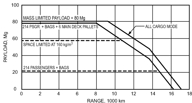
Fig. 2 Payload-Range Comparison for Wide-Body Jet
