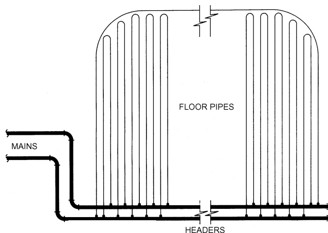
Fig. 4 Two-Pipe Header and Distribution
