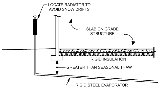
Fig. 4 Typical Thermo-Probe Installation
