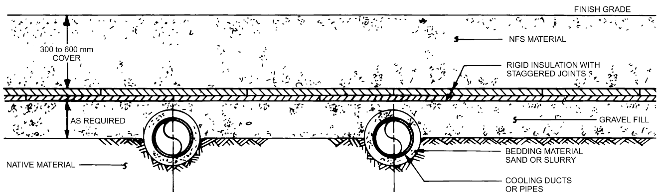
Fig. 5 Active Ground Stabilization System
