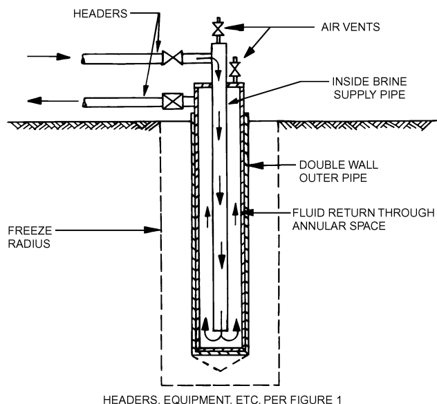
Fig. 2 Typical Freezing Point
