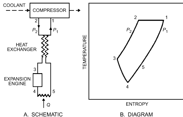
Fig. 5 Schematic for Cold Gas Expansion Refrigerator and Temperature-Entropy Diagram for Cycle
