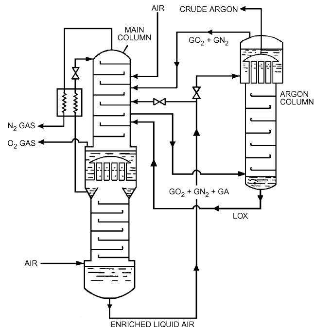
Fig. 23 Argon Recovery Subsystem
