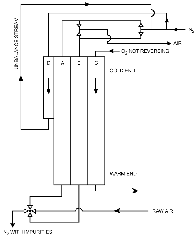
Fig. 27 Typical Flow Arrangement for Reversing Heat Exchanger in Air Separation Plant
