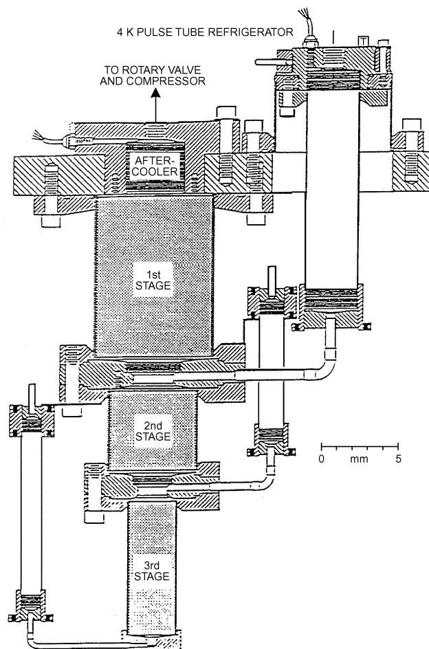
Fig. 18 Three-Stage Series Orifice Pulse Tube Cryocooler for Liquefying Helium
