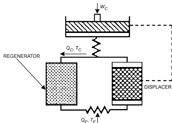
Fig. 14 Schematic of Stirling Cryocooler
