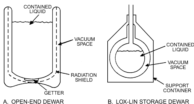
Fig. 32 Laboratory Storage Dewars for Liquid Oxygen and Nitrogen
