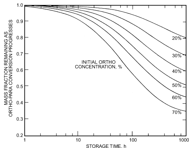
Fig. 2 Fraction of Liquid Hydrogen Evaporated due to Ortho-Parahydrogen Conversion as Function of Storage Time
