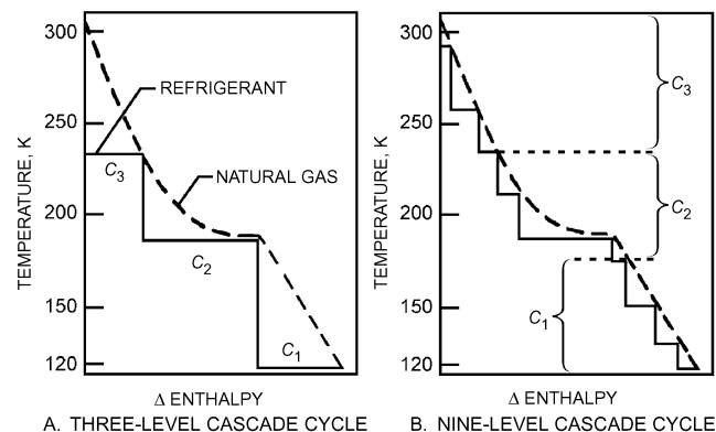
Fig. 8 (A) Three-Level and (B) Nine-Level Cascade Cycle Cooling Curves for Natural Gas
