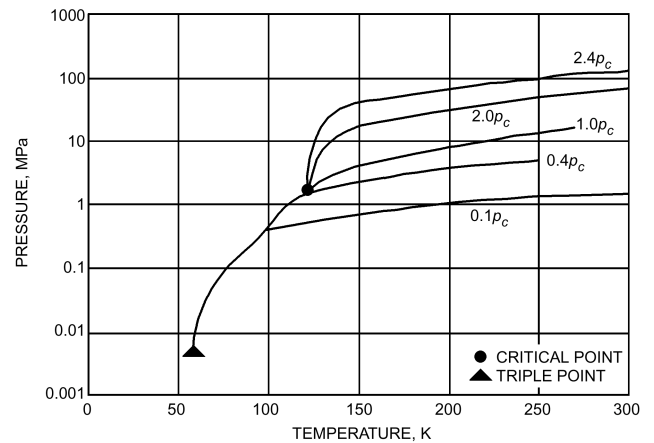
Fig. 34 Pressure Developed During Warming of Liquid Nitrogen in Closed Container
