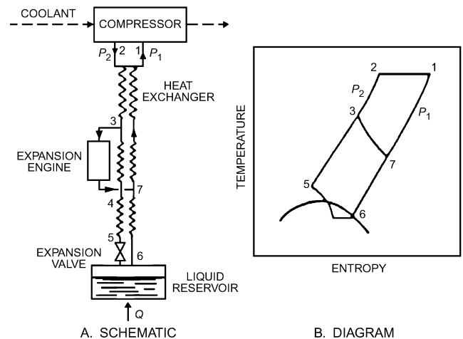
Fig. 6 Schematic for Claude Cycle Refrigerator and Temperature-Entropy Diagram for Cycle
