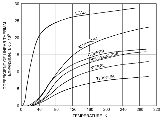
Fig. 33 Coefficient of Linear Expansion for Several Metals as Function of Temperature
