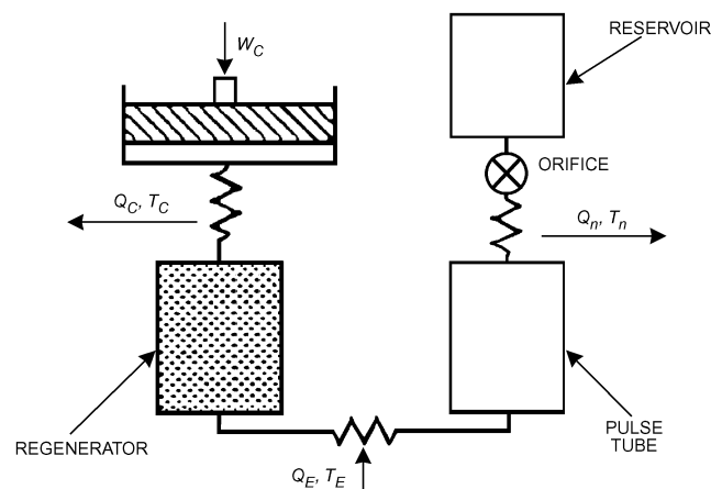
Fig. 15 Schematic for Orifice Pulse Tube Cryocooler
