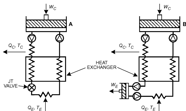
Fig. 12 Schematic of Joule-Thomson and Brayton Cycles (Two recuperative types of cycles used in cryocoolers)
