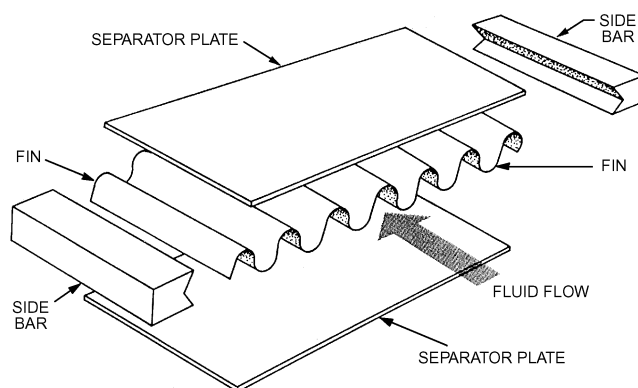
Fig. 26 Enlarged View of One Layer of Plate-and-Fin Heat Exchanger Before Assembly
