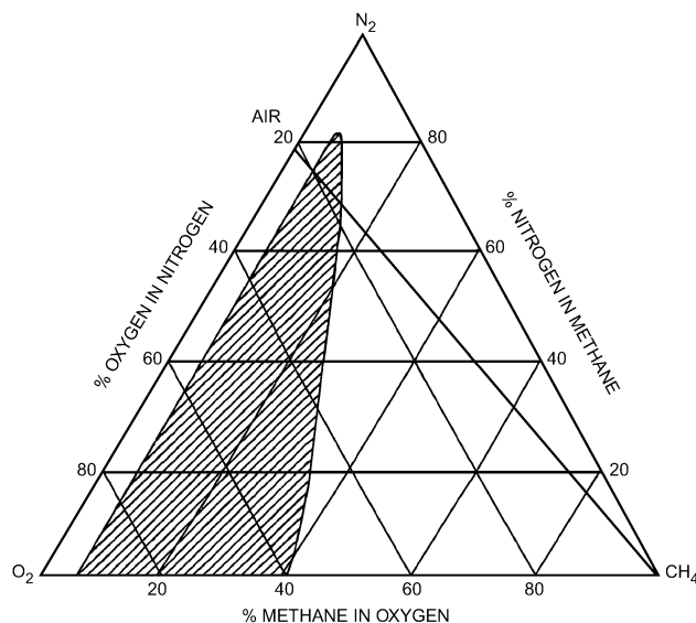
Fig. 35 Flammable Limits for O 2 -N 2 -CH 4 System (Courtesy of Air Products and Chemicals, Inc., Allentown, PA)
