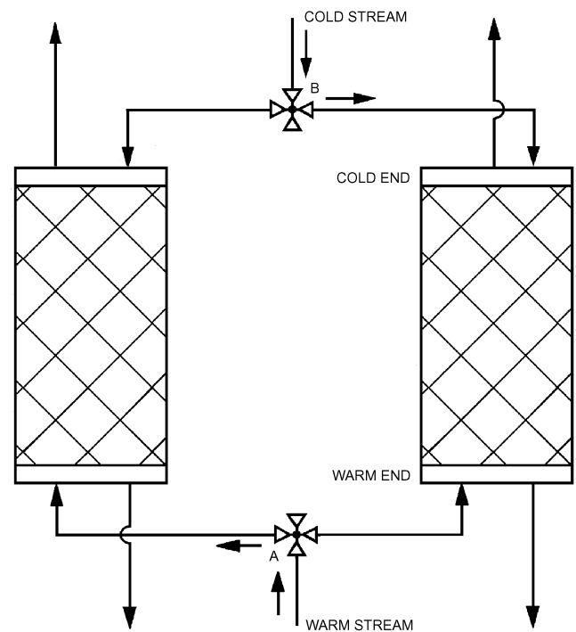
Fig. 28 Flow Arrangement in Regenerator Operation
