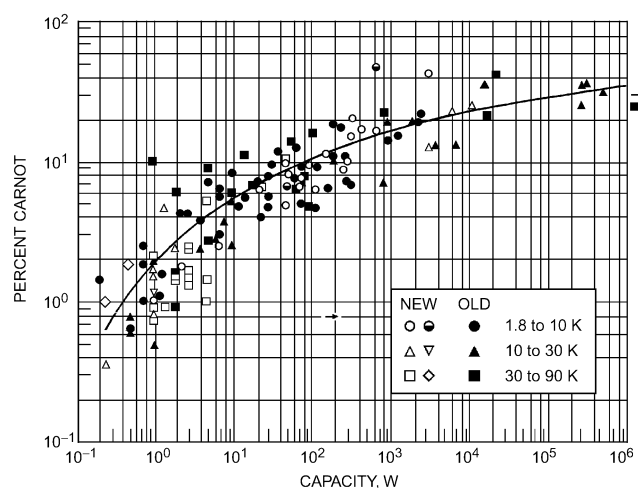
Fig. 11 Efficiency as Percent of Carnot Efficiency (For low-temperature refrigerators and liquefiers as function of refrigeration capacity)
