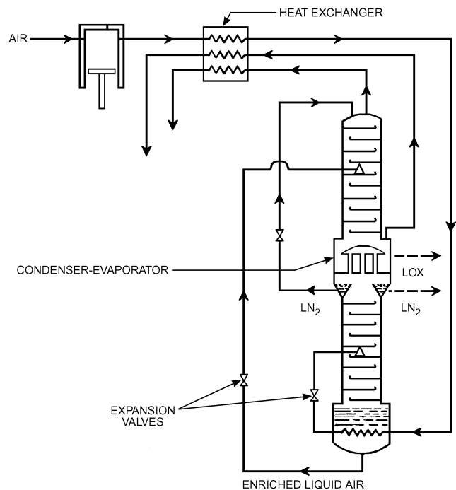
Fig. 22 Traditional Linde Double-Column Gas Separator
