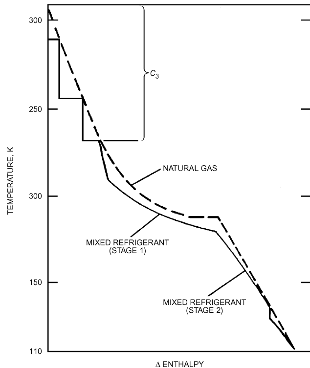
Fig. 10 Propane Precooled Mixed Refrigerant Cycle Cooling Curve for Liquefaction of Natural Gas
