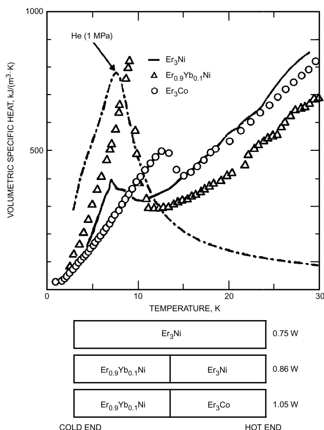
Fig. 29 Specific Heat of Several Rare Earth Matrix Materials
