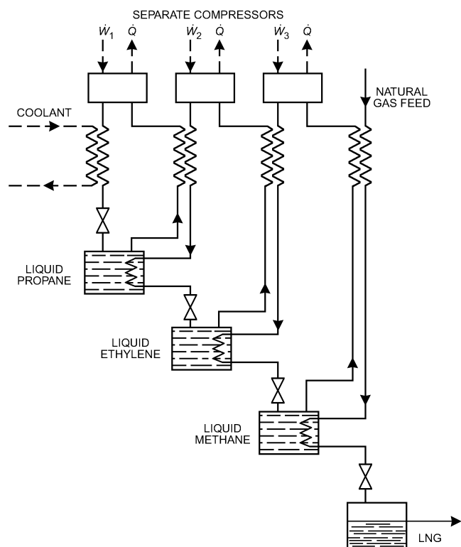
Fig. 7 Classical Cascade Compressed Vapor Refrigerator
