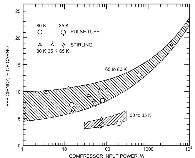
Fig. 17 Comparison of Carnot Efficiency for Several Recent Pulse Tube Cryocoolers with Similarly Powered Stirling Cryocoolers
