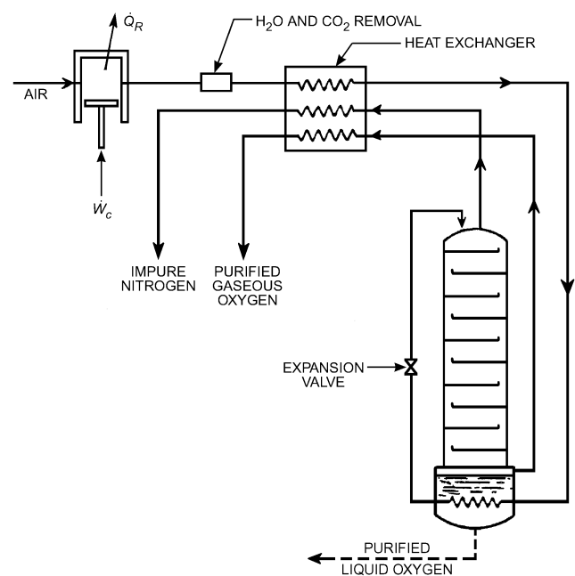
Fig. 21 Linde Single-Column Gas Separator
