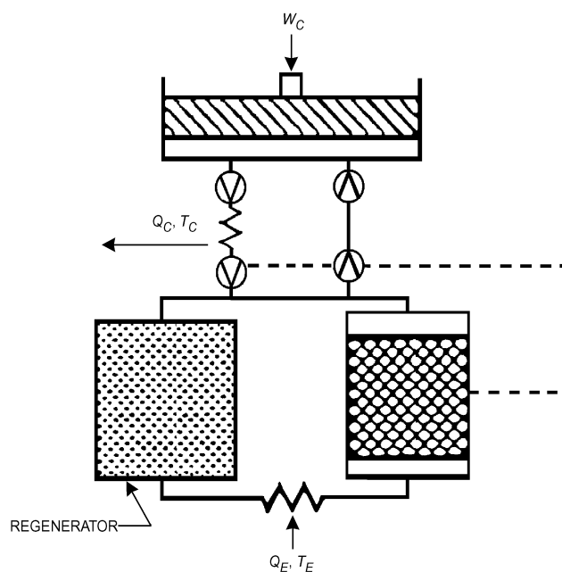
Fig. 19 Schematic for Single-Stage Gifford-McMahon Refrigerator
