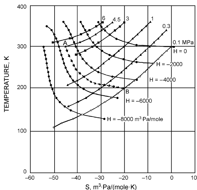
Fig. 13 Isenthalpic Expansion of Multicomponent Gaseous Mixture
