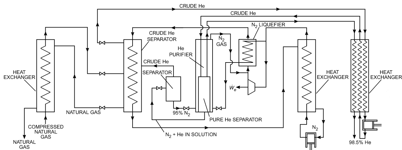
Fig. 25 Schematic of U.S. Bureau of Mines Helium Separation Plant
