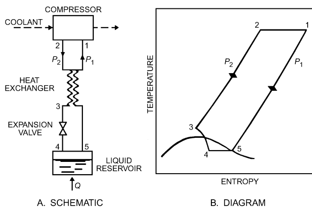
Fig. 3 Schematic and Temperature-Entropy Diagram for Simple Joule-Thomson Cycle Refrigerator
