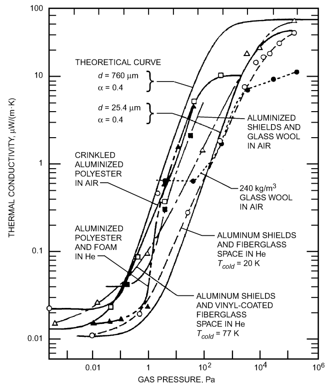
Fig. 30 Effect of Residual Gas Pressure on Apparent Thermal Conductivity of Multilayer Insulation
