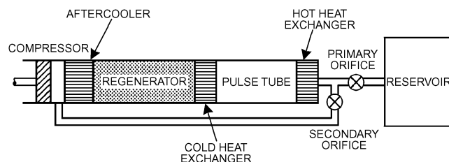
Fig. 16 Schematic of Double-Inlet Pulse Tube Refrigerator Using Secondary Orifice
