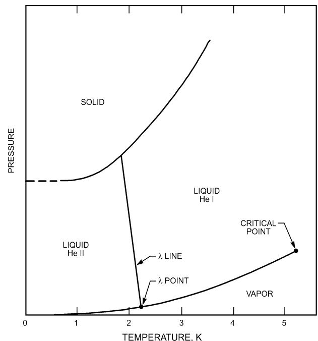
Fig. 1 Phase Diagram for Helium 4
