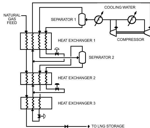
Fig. 9 Mixed Refrigerant Cycle Used for Liquefaction of Natural Gas
