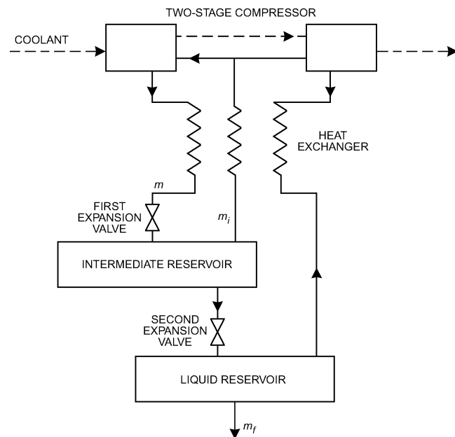
Fig. 4 Dual Pressure Joule-Thomson Cycle Used as Liquefier
