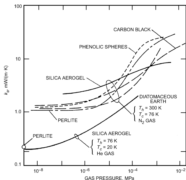
Fig. 31 Apparent Thermal Conductivity of Several Powder Insulations as Function of Residual Gas Pressure
