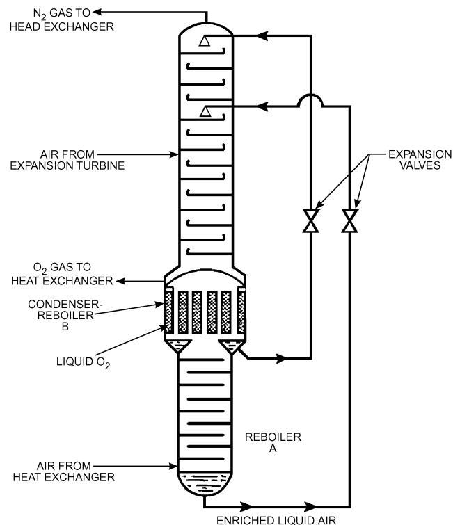
Fig. 24 Contemporary Double-Column Gas Separator
