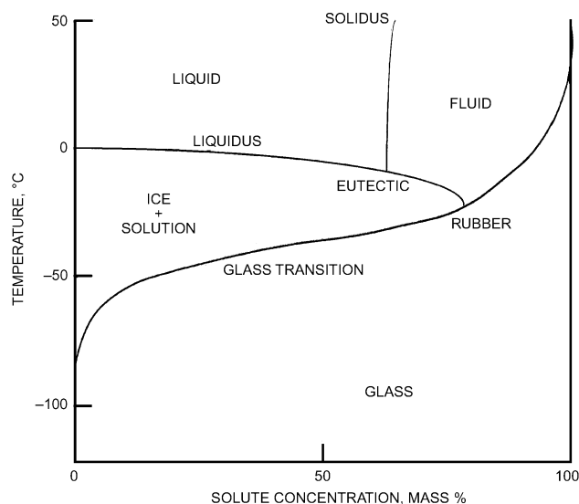
Fig. 4 Generic State Diagram for Aqueous Solution
