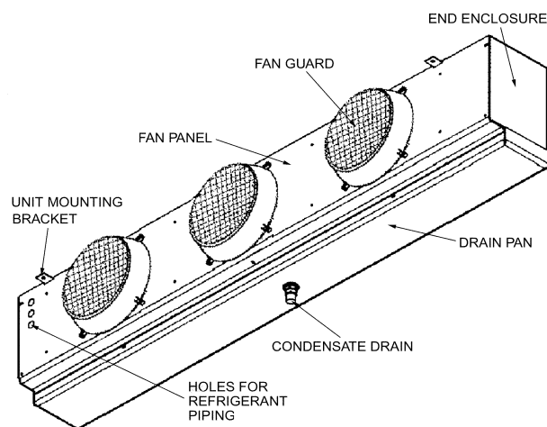
Fig. 3 Low-Profile Cooler
