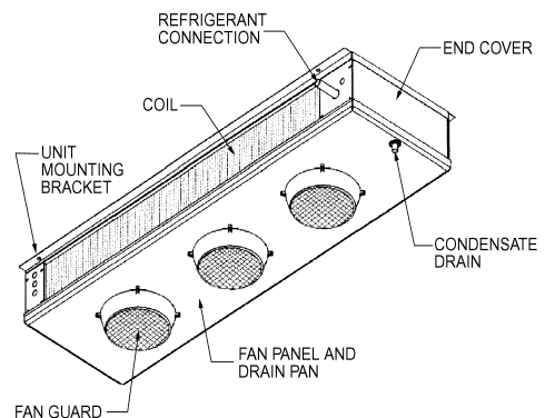
Fig. 2 Low-Air-Velocity Units
