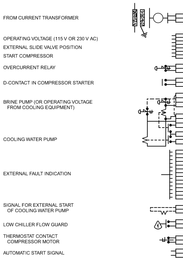
Fig. 15 Typical External Connections for Screw Compressor Chiller
