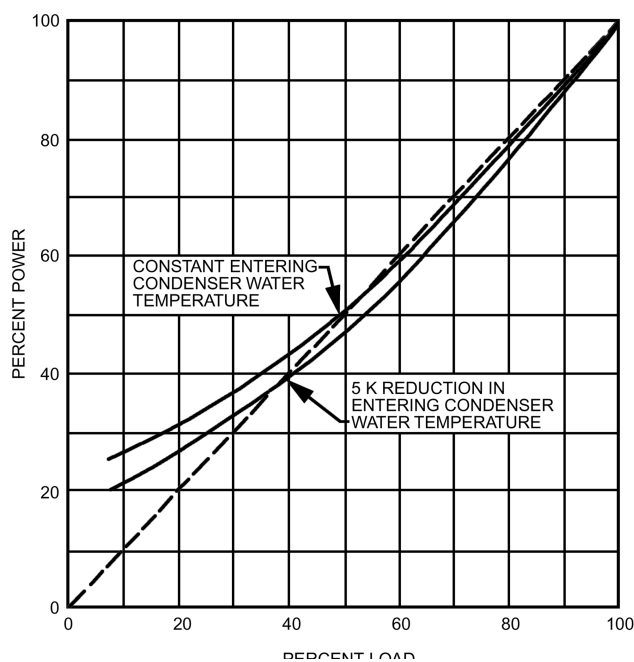
Fig. 14 Typical Screw Compressor Chiller Part-Load Power Consumption
