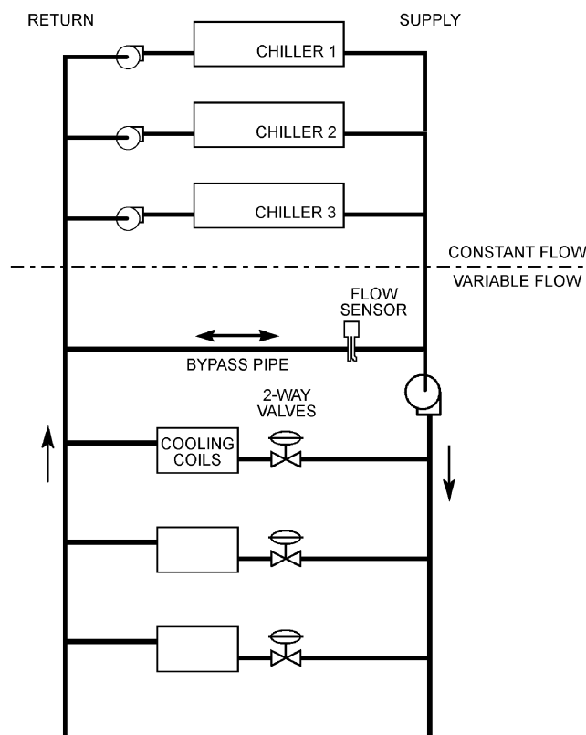
Fig. 2 Decoupled System
