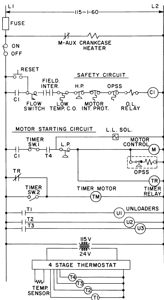
Fig. 9 Reciprocating Liquid Chiller Control System
