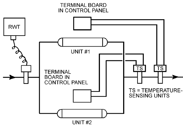
Fig. 3 Parallel Operation High Design Water Leaving Coolers (Approximately 7°C and Above)
