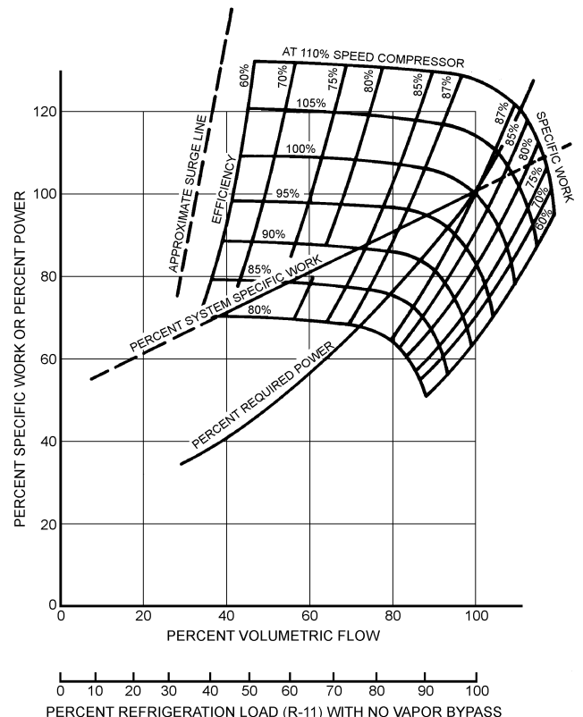
Fig. 11 Typical Centrifugal Compressor Performance at Various Speeds
