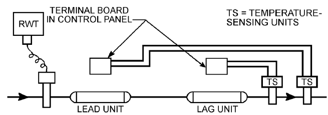
Fig. 5 Series Operation
