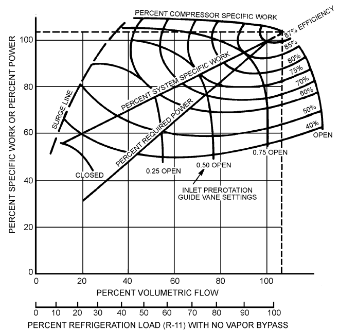
Fig. 10 Typical Centrifugal Compressor and System at Constant Speed
