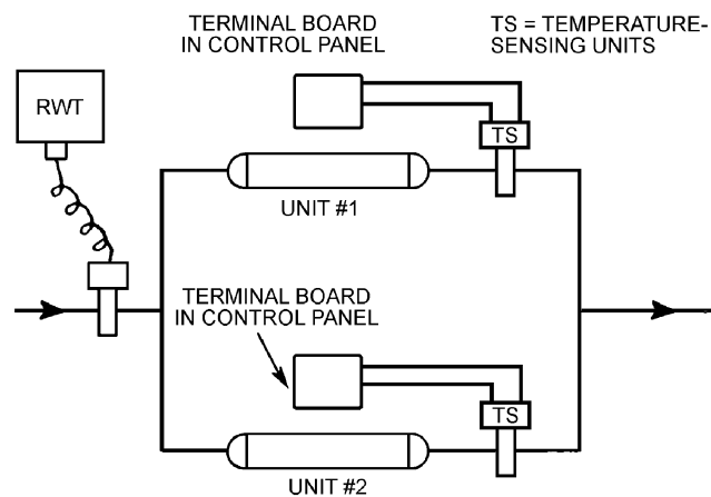
Fig. 4 Parallel Operation Low Design Water Leaving Coolers (Below Approximately 7°C)
