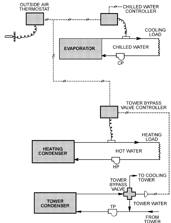
Fig. 6 Heat-Recovery Control System
