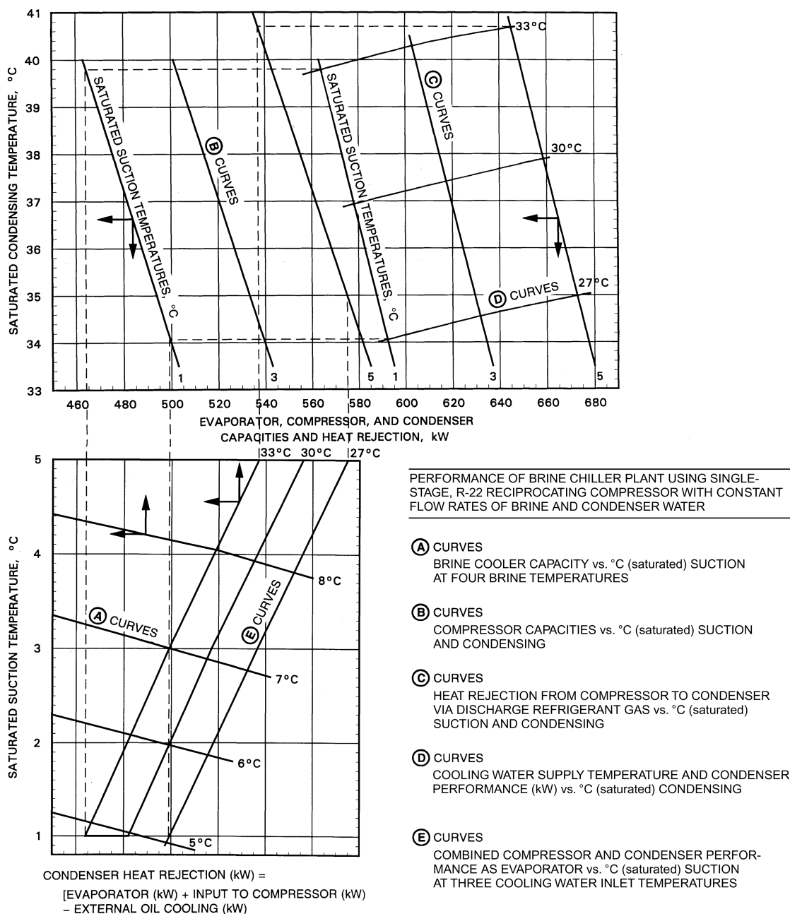
Fig. 1 Brine Chiller Balance Curve
