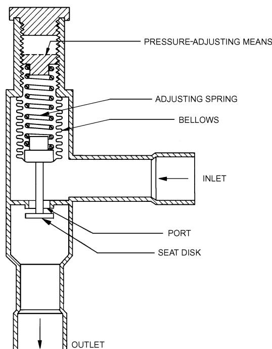
Fig. 25 Direct-Acting Suction Pressure Regulator
