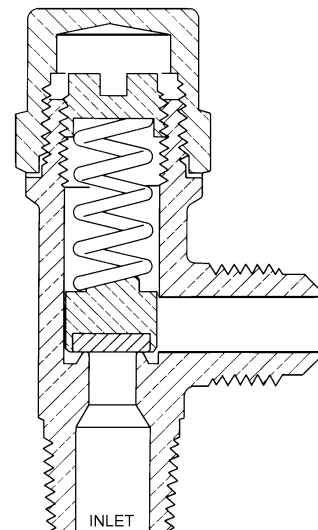
Fig. 37 Pop-Type Safety Relief Valves
