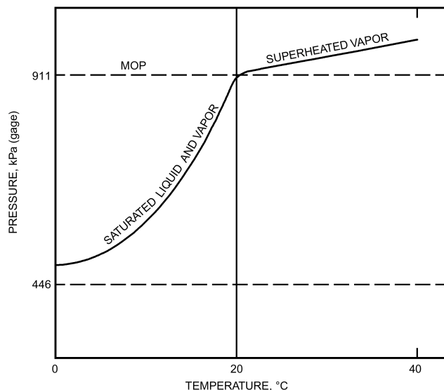
Fig. 13 Pressure-Temperature Relationship of R-22 Gas Charge in Thermostatic Element
