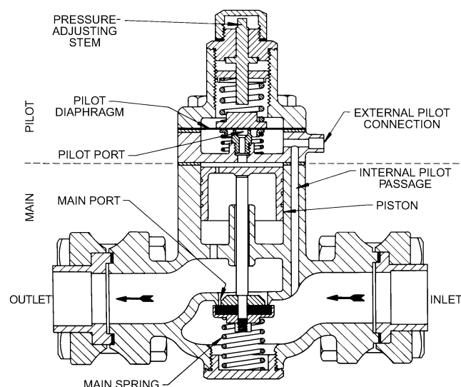
Fig. 21 Pilot-Operated Evaporator Pressure Regulator (Self-Powered)
