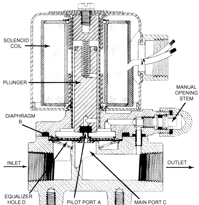
Fig. 31 Normally Closed Pilot-Operated Solenoid Valve with Direct-Lift Feature
