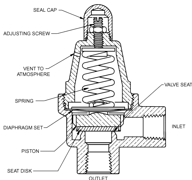
Fig. 38 Diaphragm Relief Valve
