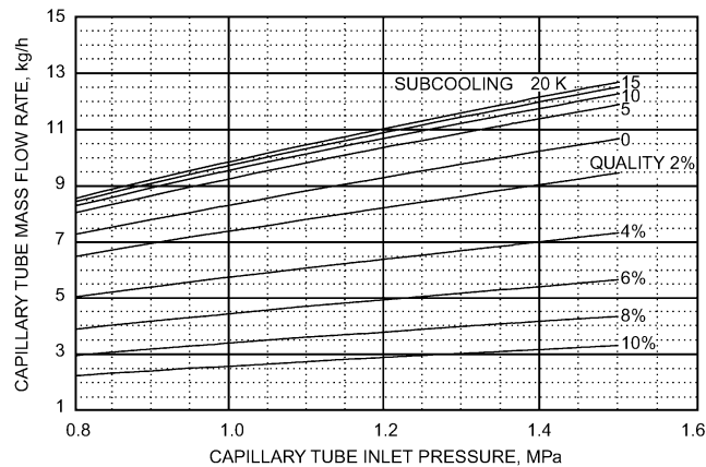
Fig. 53 Mass Flow Rate of R-134a Through a Capillary Tube-Suction Line Heat Exchange
