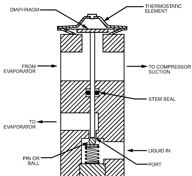
Fig. 18 Typical Block Valve
