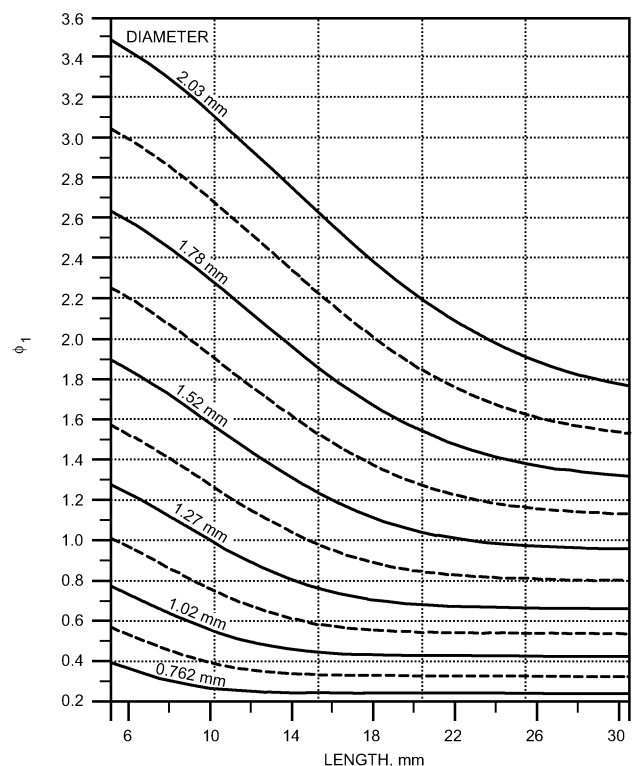
Fig. 62 Correction Factor for Short Tube Geometry (R-22) (Adapted from Aaron and Domanski 1990)
