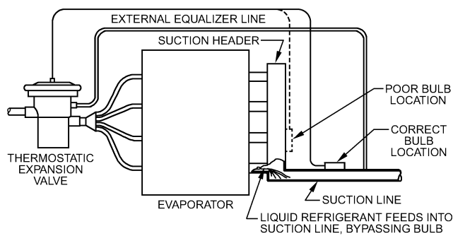
Fig. 15 Bulb Location for Thermostatic Expansion Valve
