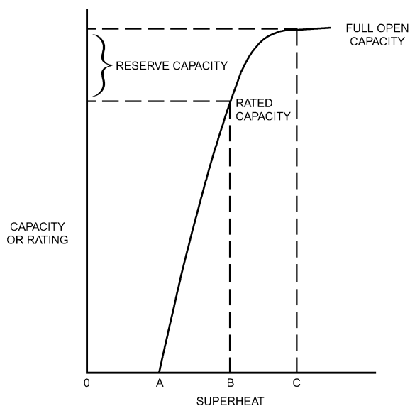
Fig. 12 Typical Gradient Curve for Thermostatic Expansion Valves
