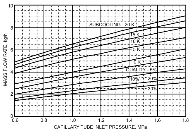
Fig. 45 Mass Flow Rate of R-134a Through Capillary Tube (Capillary tube diameter is 0.86 mm ID and length is 3300 mm)
