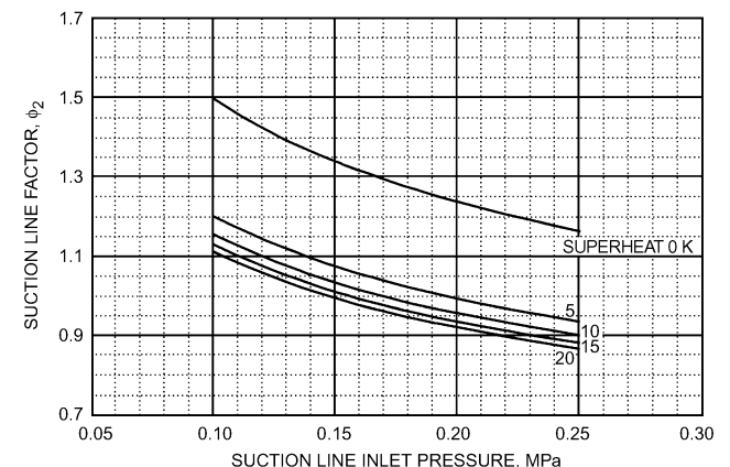
Fig. 58 Suction Line Condition Correction Factor for Quality R-134a Inlet Conditions
