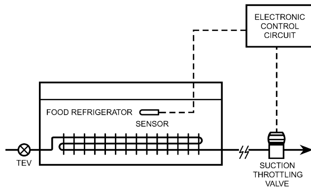
Fig. 19 Electronically Controlled, Electrically Operated Suction-Throttling Regulator
