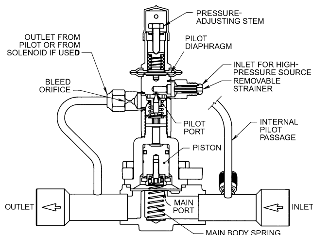
Fig. 22 Pilot-Operated Evaporator Pressure Regulator (High-Pressure-Driven)
