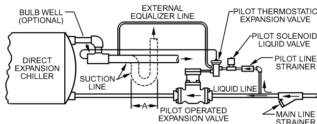
Fig. 16 Pilot-Operated Thermostatic Expansion Valve Controlling Liquid Refrigerant Flow to Direct-Expansion Chiller
