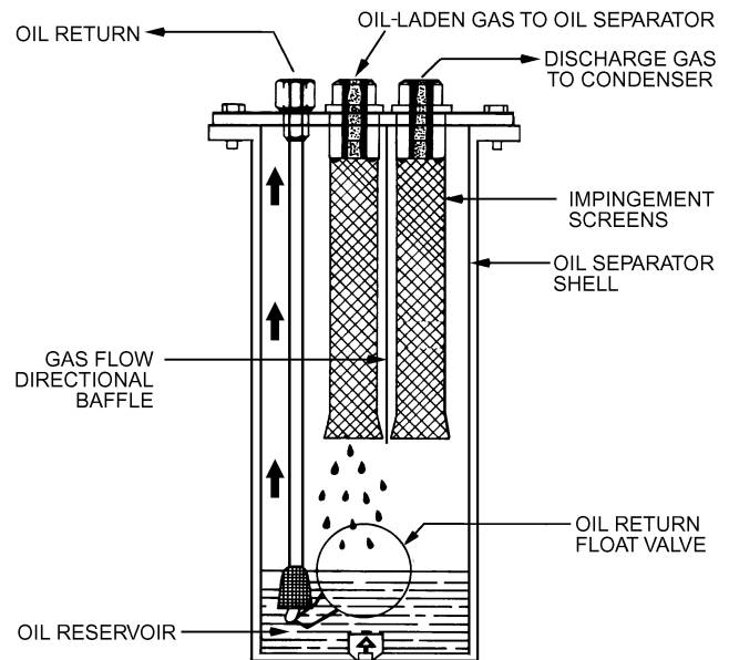
Fig. 40 Discharge-Line Lubricant Separator
