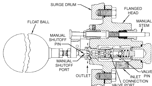
Fig. 29 Low-Side Float Valve
