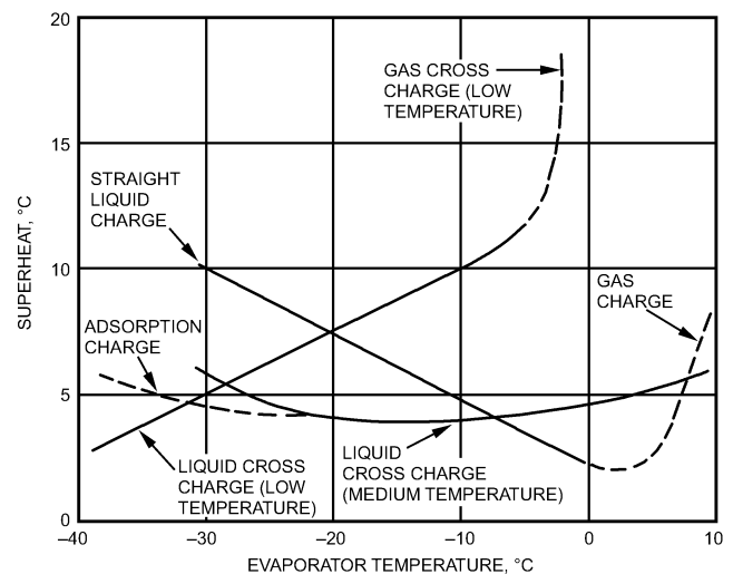
Fig. 14 Typical Superheat Characteristics of Common Thermostatic Charges
