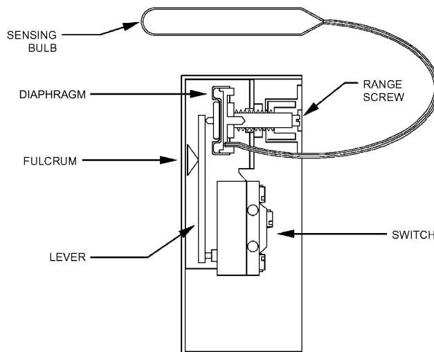
Fig. 3 Indirect Temperature Switch
