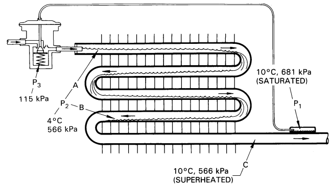
Fig. 11 Thermostatic Expansion Valve Controlling Flow of Liquid R-22 Entering Evaporator, Assuming R-22 Charge in Bulb
