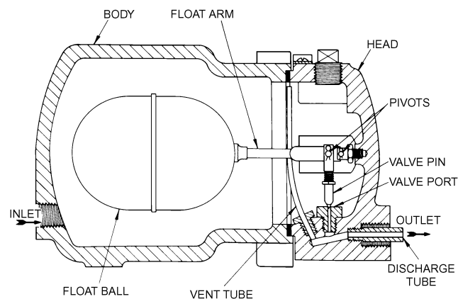
Fig. 28 High-Side Float Valve
