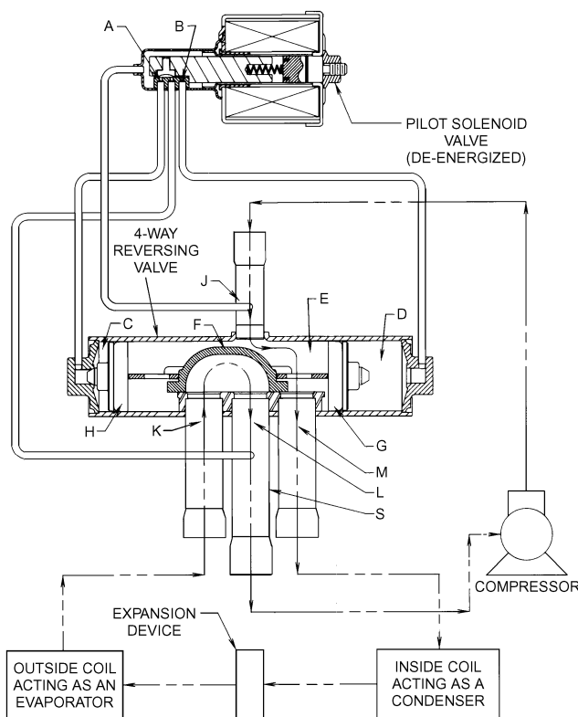
Fig. 34 Four-Way Slide Refrigerant-Reversing Valve Used in Heating Cycle of Refrigeration System
