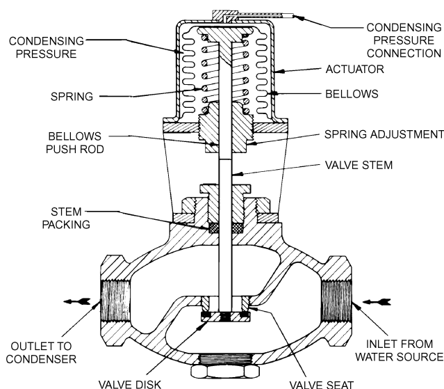
Fig. 35 Two-Way Condensing Water Regulator
