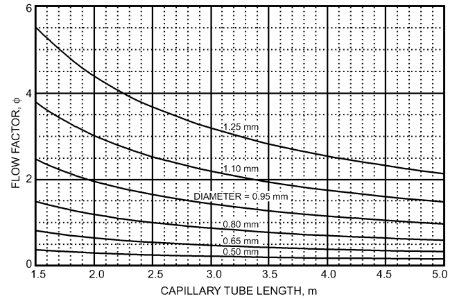
Fig. 49 Flow Rate Correction Factor \phi for R-410A for Two-Phase Condition at Capillary Tube Inlet
