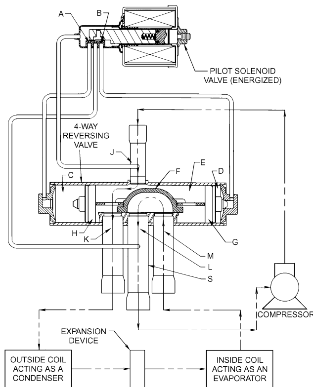
Fig. 33 Four-Way Slide Refrigerant-Reversing Valve Used in Cooling (or Defrosting) Cycle of Refrigeration System
