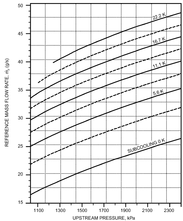
Fig. 61 R-22 Mass Flow Rate vs. Condenser Pressure for Reference Short Tube: L = 12.7 \text{ mm} , D = 1.35 \text{ mm} , Sharp-Edged (Adapted from Aaron and Domanski 1990)
