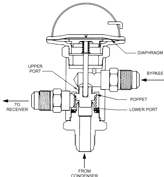
Fig. 27 Three-Way Condenser-Pressure-Regulating Valve
