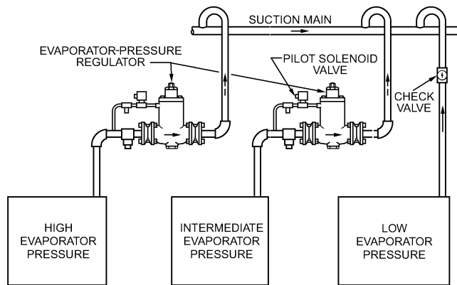
Fig. 23 Evaporator Pressure Regulators in Multiple System
