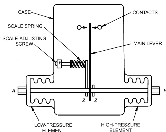
Fig. 5 Differential Switch Schematic
