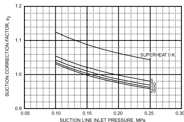
Fig. 55 Suction Line Condition Correction Factor for R-134a Subcooled Inlet Conditions
