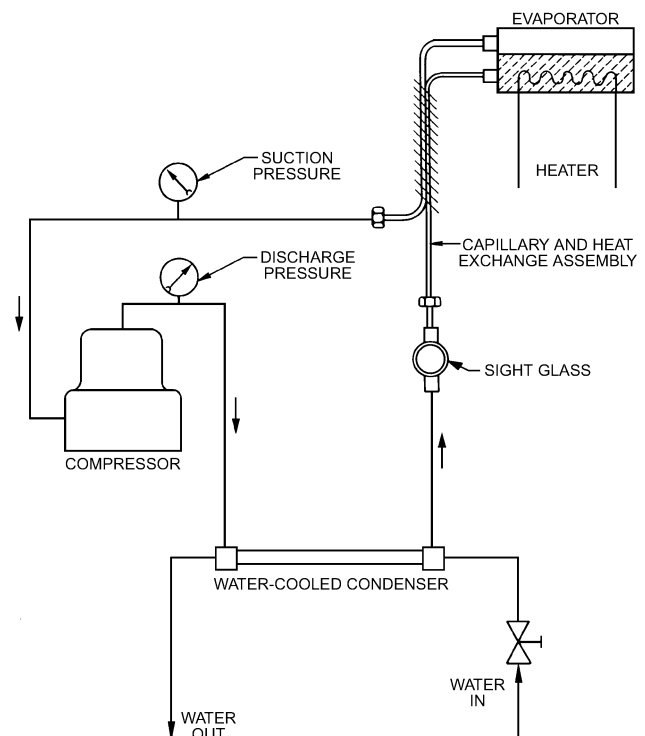
Fig. 44 Test Setup for Determining Capacity Balance Characteristic of Compressor, Capillary, and Heat Exchanger
