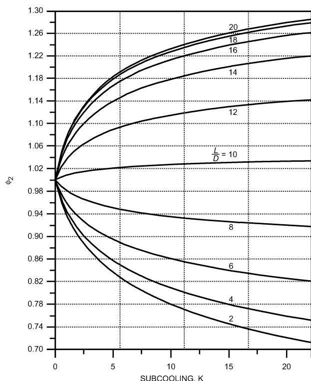
Fig. 63 Correction Factor for L/D Ratio vs. Subcooling (R-22)
