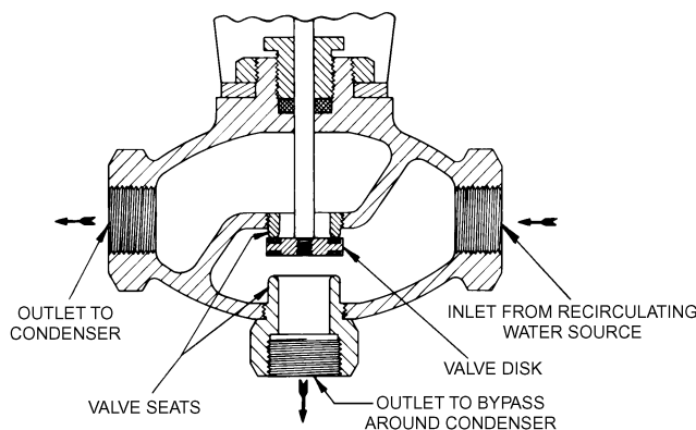
Fig. 36 Three-Way Condensing Water Regulator
