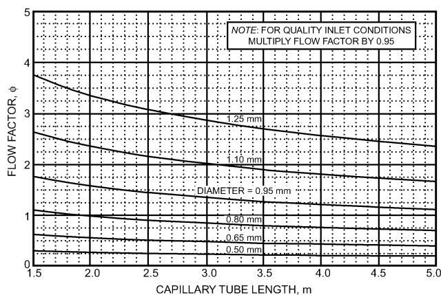
Fig. 46 Flow Rate Correction Factor \phi for R-134a
