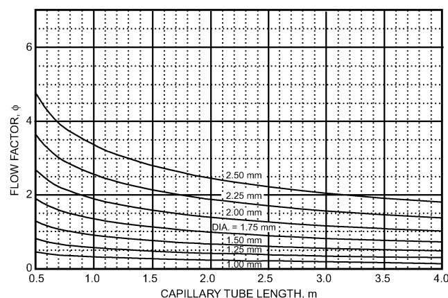
Fig. 51 Flow Rate Correction Factor \phi for R-22 for Subcooled Condition at Capillary Tube Inlet
