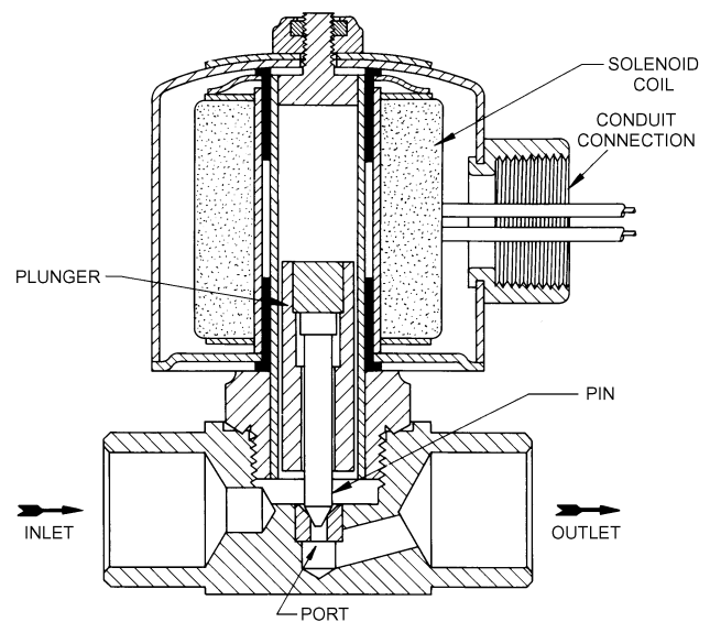
Fig. 30 Normally Closed Direct-Acting Solenoid Valve with Hammer-Blow Feature
