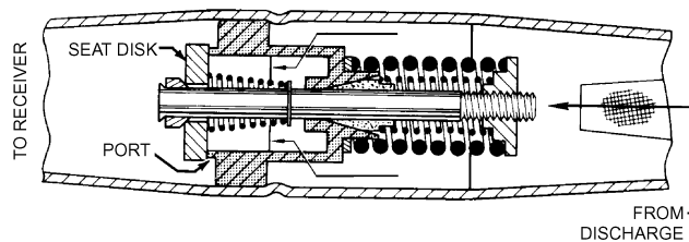
Fig. 26 Condenser Bypass Valve
