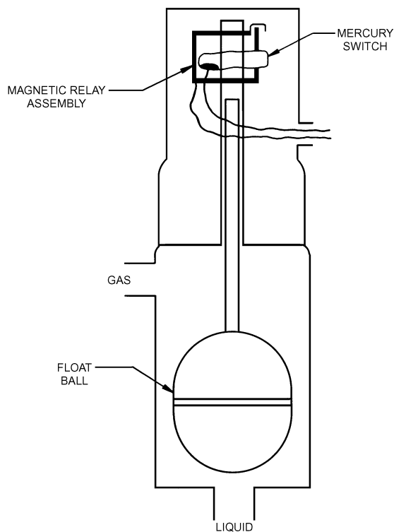
Fig. 7 Magnetic Float Switch
