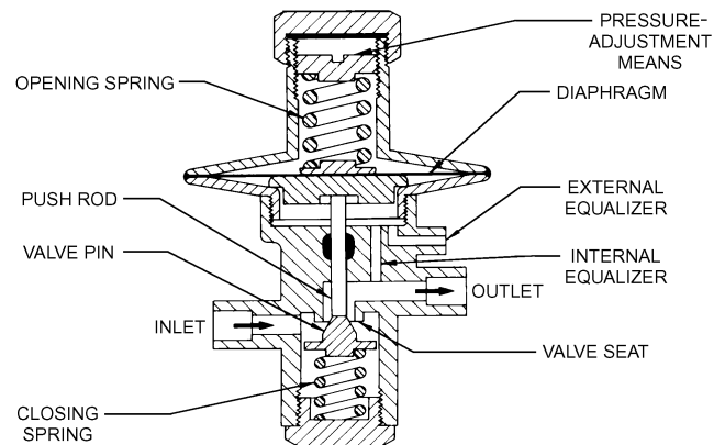
Fig. 24 Constant-Pressure Expansion Valve
