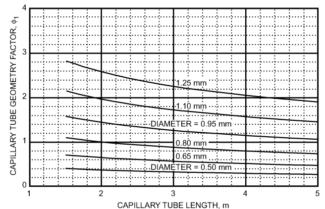
Fig. 57 Capillary Tube Geometric Correction Factor for Quality R-134a Inlet Conditions
