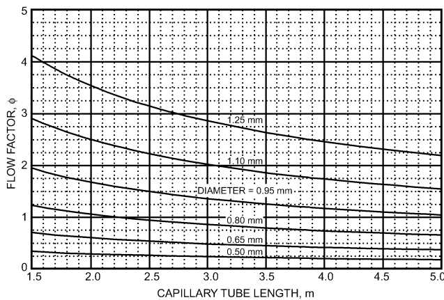
Fig. 48 Flow Rate Correction Factor \phi for R-410A for Subcooled Condition at Capillary Tube Inlet
