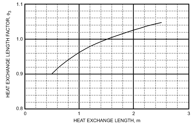
Fig. 56 Heat Exchange Length Correction Factor for Subcooled R-134a Inlet Conditions
