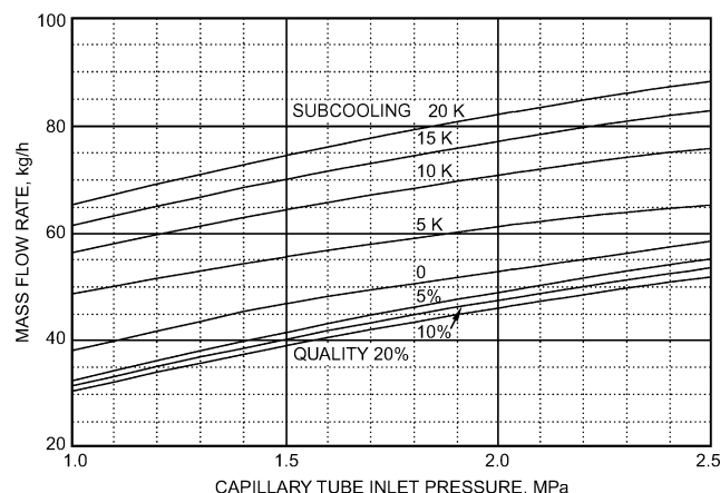
Fig. 50 Mass Flow Rate of R-22 Through Capillary Tube (Capillary tube diameter is 1.68 mm ID and length is 1524 mm)
