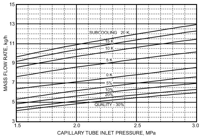
Fig. 47 Mass Flow Rate of R-410A Through Capillary Tube (Capillary tube diameter is 0.86 mm ID and length is 3300 mm)
