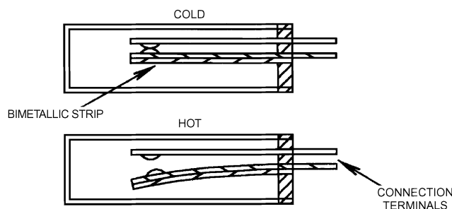
Fig. 4 Direct Temperature Switch
