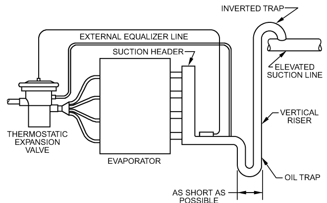
Fig. 17 Bulb Location When Suction Main Is Above Evaporator
