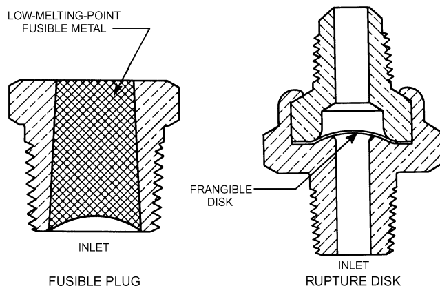
Fig. 39 Safety Relief Devices
