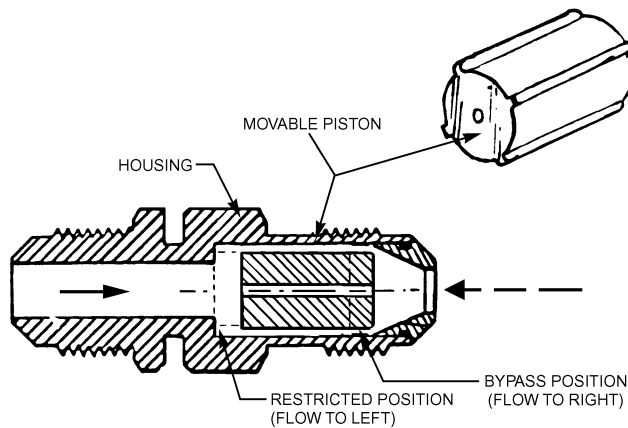
Fig. 59 Schematic of Movable Short-Tube Restrictor
