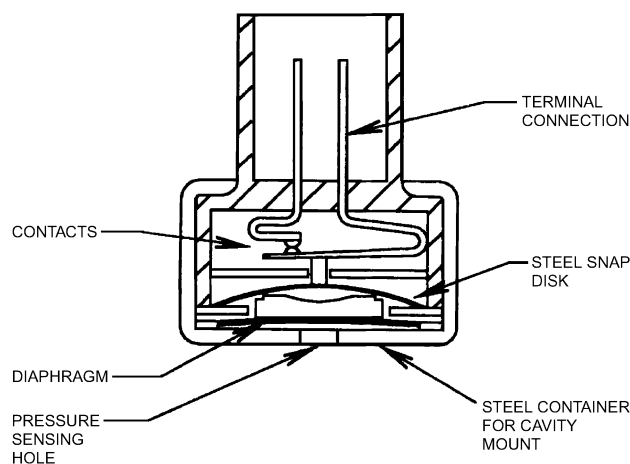
Fig. 2 Miniaturized Pressure Switch
