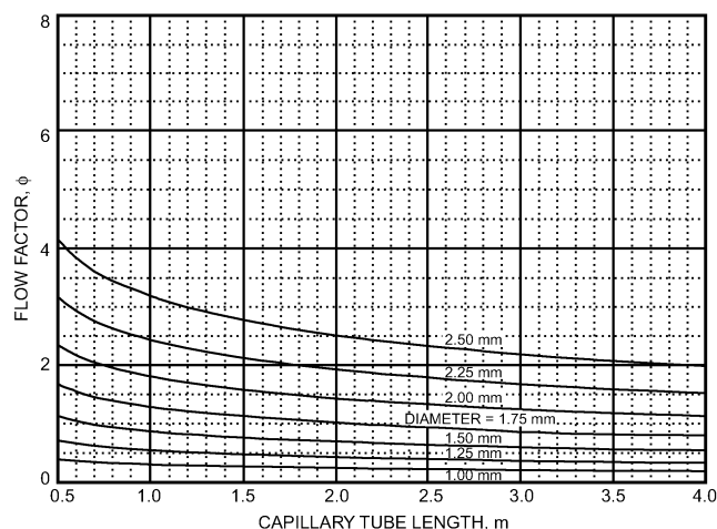
Fig. 52 Flow Rate Correction Factor \phi for R-22 for Two-Phase Condition at Capillary Tube Inlet
