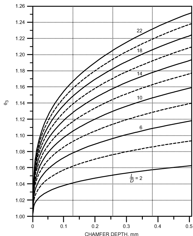
Fig. 64 Correction Factor for Inlet Chamfering (R-22)
