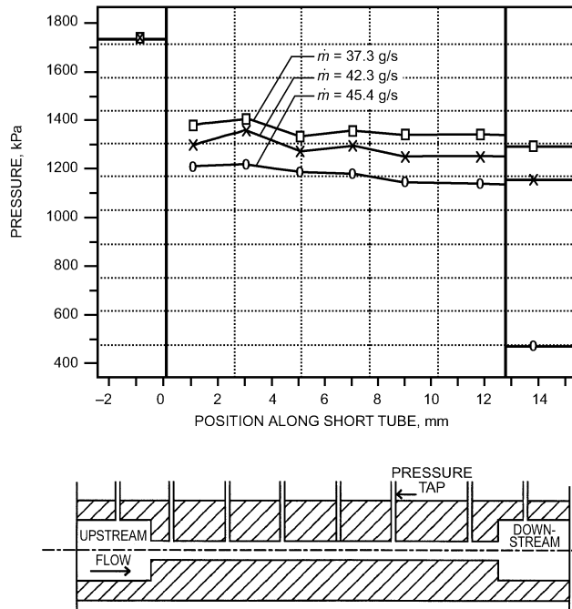
Fig. 60 R-22 Pressure Profile at Various Down-Stream Pressures with Constant Upstream Conditions: L = 12.7 \text{ mm} , D = 1.35 \text{ mm} , Subcooling 13.9 \text{ K} (Adapted from Aaron and Domanski 1990)
