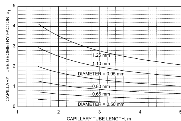
Fig. 54 Capillary Tube Geometric Correction Factor for Subcooled R-134a Inlet Conditions
