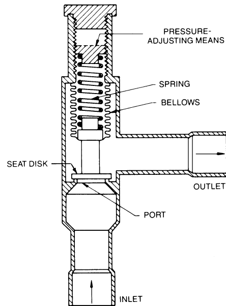
Fig. 20 Direct-Operated Evaporator Pressure Regulator
