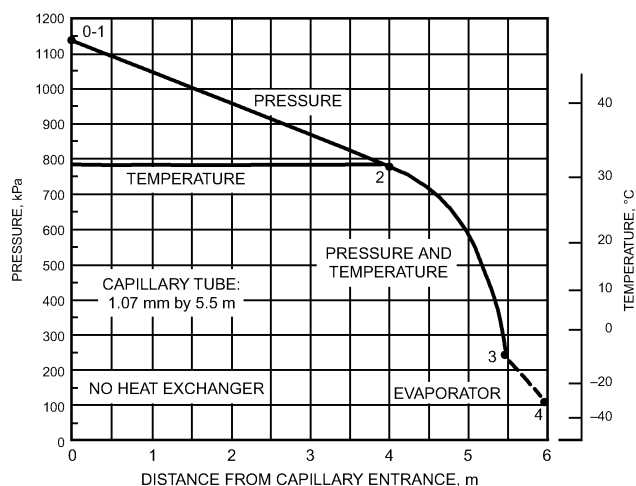
Fig. 41 Pressure and Temperature Distribution Along Typical Capillary Tube (Bolstad and Jordan 1948)
