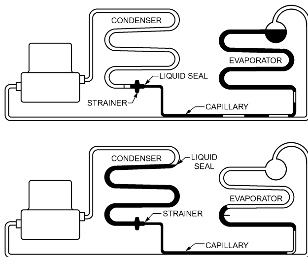
Fig. 42 Effect of Capillary Tube Selection on Refrigerant Distribution
