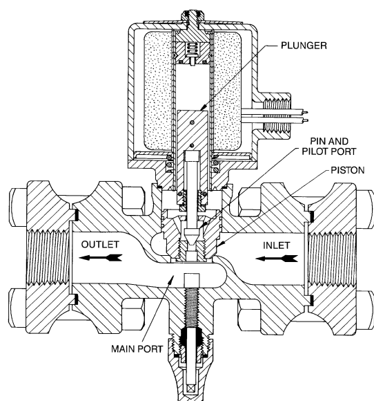
Fig. 32 Normally Closed Pilot-Operated Solenoid Valve with Hammer-Blow and Mechanically Linked Piston-Pin Plunger Features
