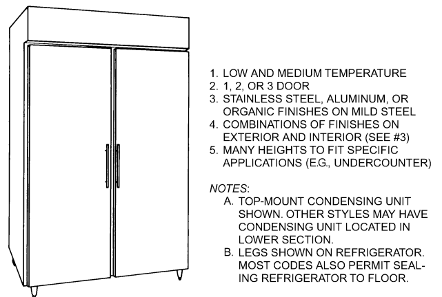
Fig. 1 Reach-In Food Storage Cabinet Features
