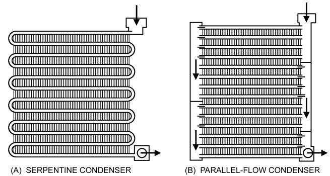
Fig. 6 Basic Automotive Condensers (Mathur 1999b. Reprinted with permission from SAE Paper 1999-01-0236. Copyright © 1999 SAE International.)
