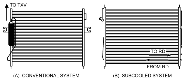
Fig. 7 Conventional and Subcooled PRF Condenser Designs
