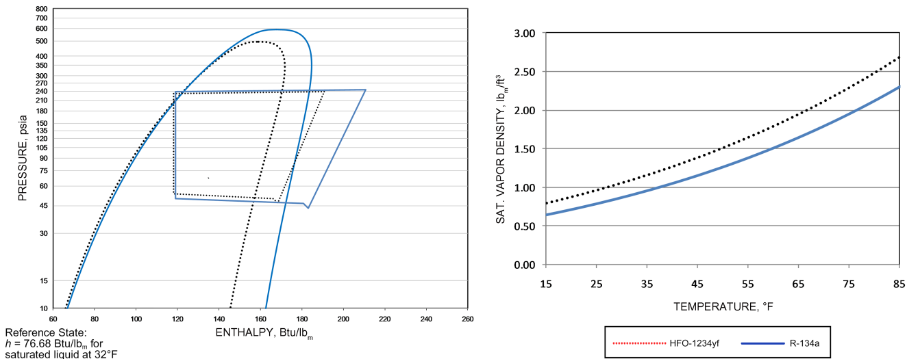
Fig. 9 Comparison of Thermodynamic Cycle Between Base Case (R-134a) and HFO-1234yf (Spatz and Minor 2008)
