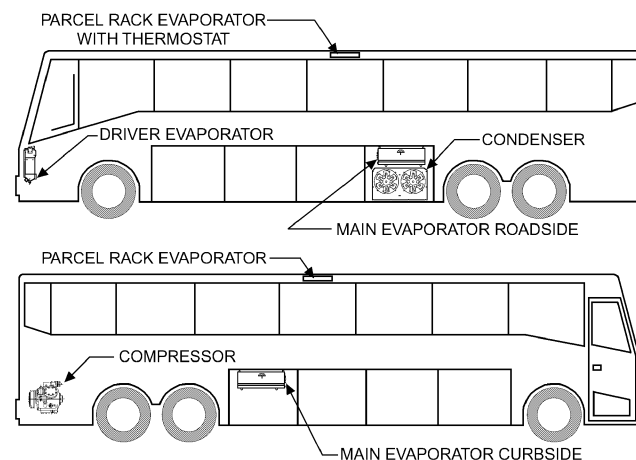
Fig. 3 Typical Arrangement of Air-Conditioning in Interurban Bus
