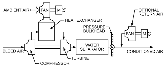
BOOTSTRAP CYCLE
