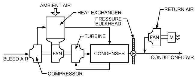
CHILLED RECIRCULATION CYCLE
