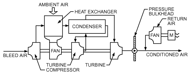
CONDENSING CYCLE
