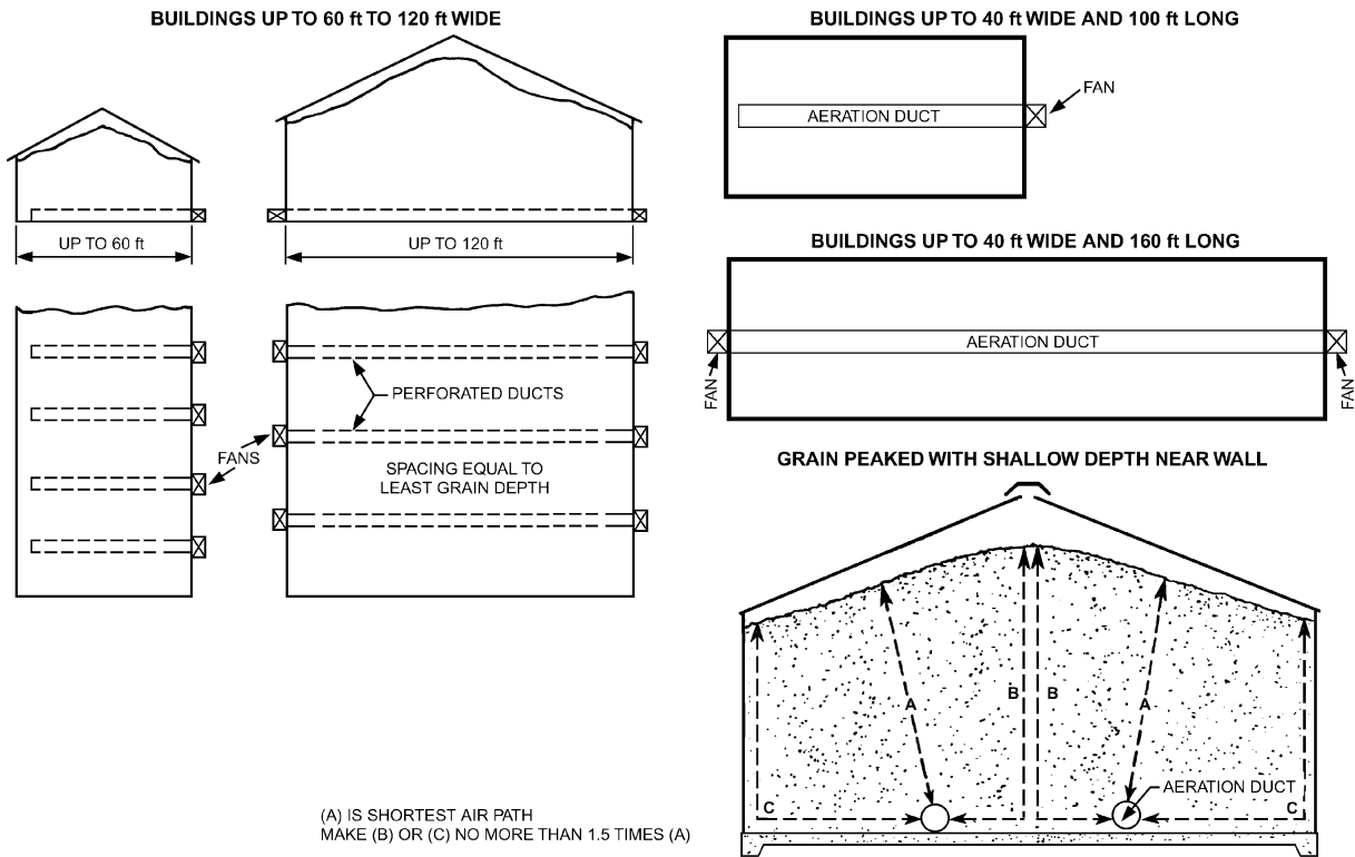
Fig. 13 Duct Arrangements for Large Flat Storages
