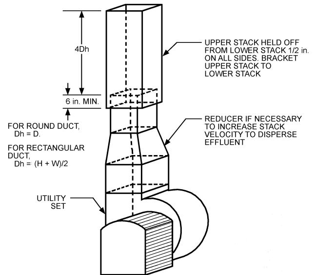
Fig. 35 Rooftop Centrifugal Fan (Utility Set) with Vertical Discharge
