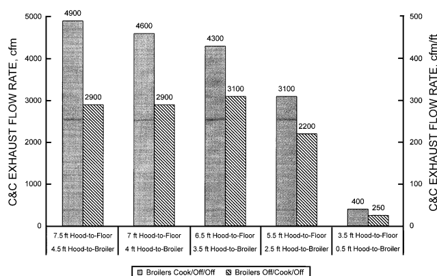
Fig. 9 Exhaust Capture and Containment Rates for Gas Underfired Broiler under 10 ft Wall Canopy Hood at Various Mounting Heights (Swierczyna et al. 2006)
