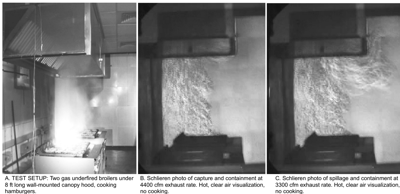
Fig. 13 Hot-Air Plume from Cooking Appliances under Wall-Mounted Canopy Hood
