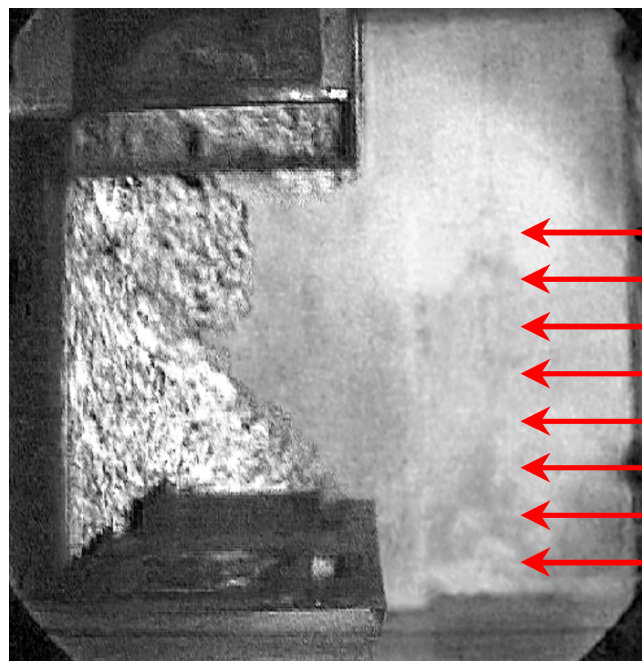
Fig. 27 Schlieren Image Showing Plume Being Effectively Captured when Replacement Air Is Supplied at Low Velocity from Displacement Diffusers (Brohard et al. 2003)
