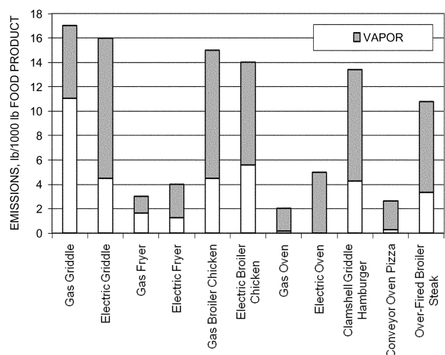
Fig. 12A Grease in Particulate and Vapor Phases for Commercial Cooking Appliances with Total Emissions Approximately Less Than 50 lb/1000 lb of Food Cooked
