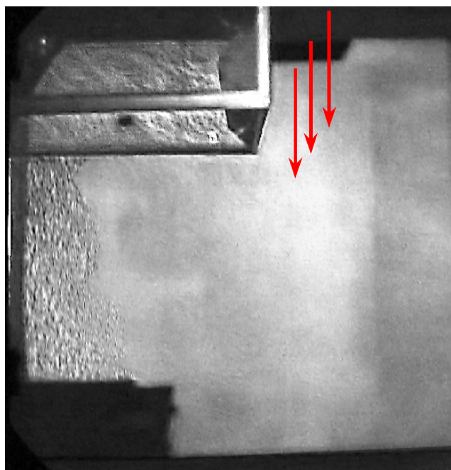
Fig. 25 Schlieren Image Showing Effective Plume Capture with Replacement Air Supplied Through 16 in. Wide Perforated Perimeter Supply, Shown with Additional Front Overhang (Brohard et al. 2003)
