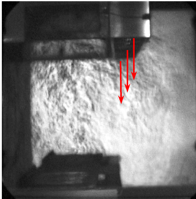
Fig. 21 Schlieren Image Showing Thermal Plume Being Pulled Outside Hood by Air Curtain (Brohard et al. 2003)
