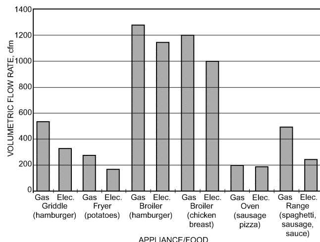
Fig. 12C Plume Volumetric Flow Rate at Hood Entrance from Various Commercial Cooking Appliances (Kuehn et al. 1999)
