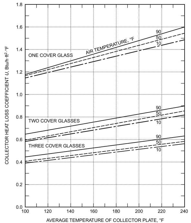
Fig. 12 Variation of Overall Heat Loss Coefficient U_L with Absorber Plate Temperature and Ambient Air Temperatures for Single-, Double-, and Triple-Glazed Collectors
