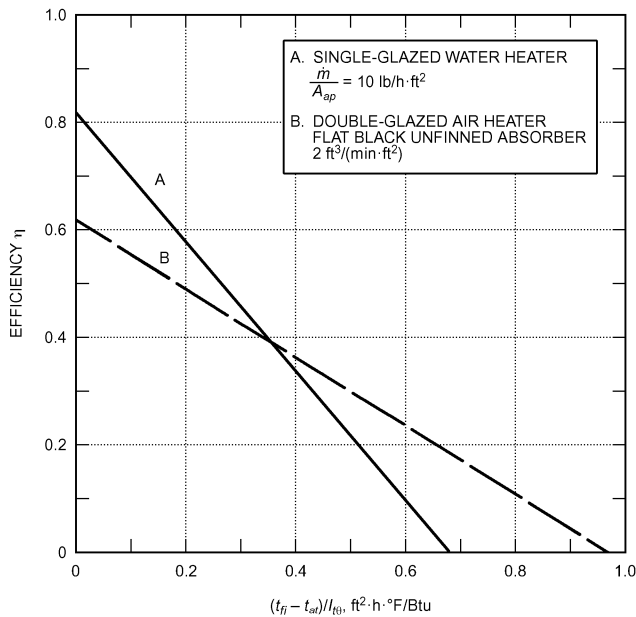
Fig. 13 Efficiency Versus (t_{fi} - t_a)/I_{\theta} for Single-Glazed Solar Water Heater and Double-Glazed Solar Air Heater
