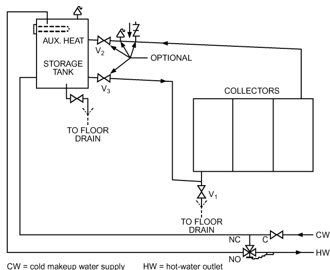
Fig. 14 Thermosiphon System
