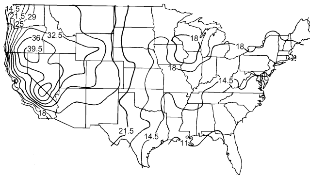
Fig. 22 Average Monthly Sky Temperature Depression ( T_{air} - T_{sky} ) for July, °F (Adapted from Martin and Berdahl 1984)
