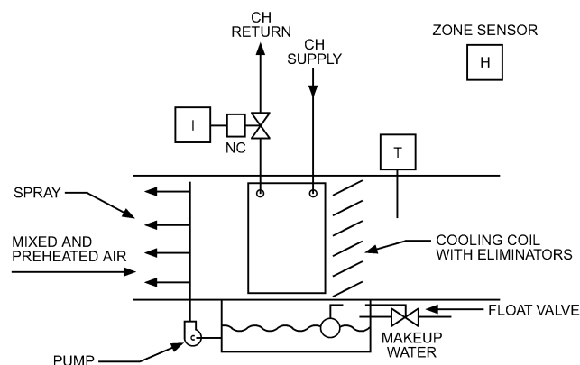
Fig. 33 Sprayed-Coil Dehumidifier
