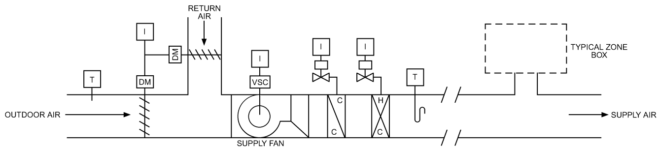
Fig. 42 Multiple-Zone, Single-Duct System
