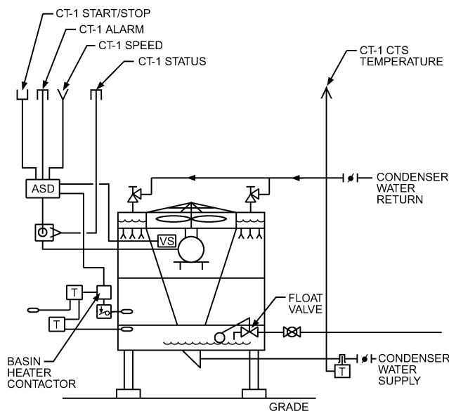
Fig. 13 Cooling Tower
