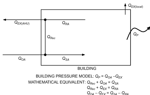
Fig. 18 Building Pressure Model
