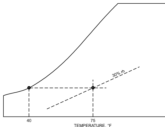
Fig. 31 Psychrometric Chart: Cooling and Dehumidifying, Practical Low Limit
