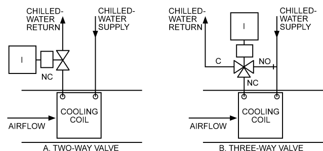
Fig. 14 Control of Chilled-Water Coils
