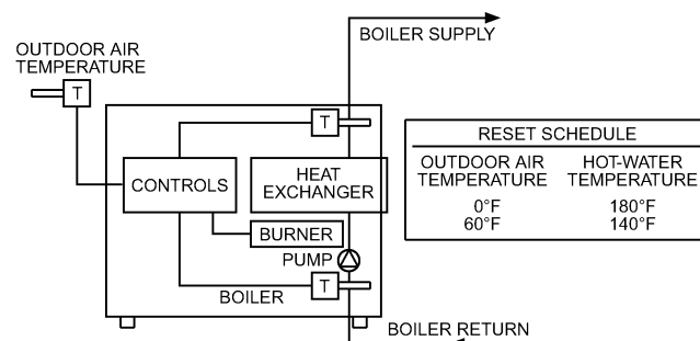
Fig. 1 Boiler Control
