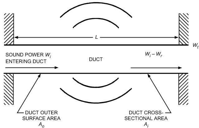
Fig. 28 Breakout Noise
