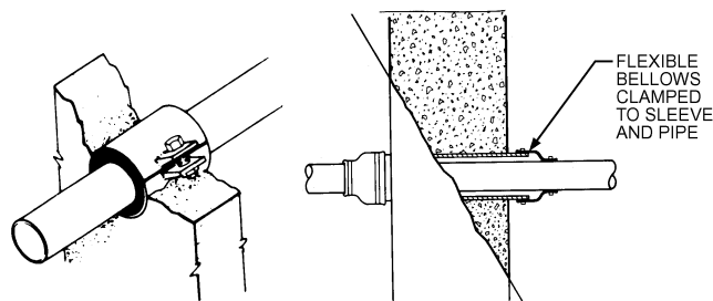
Fig. 45 Acoustical Pipe Penetration Seals
