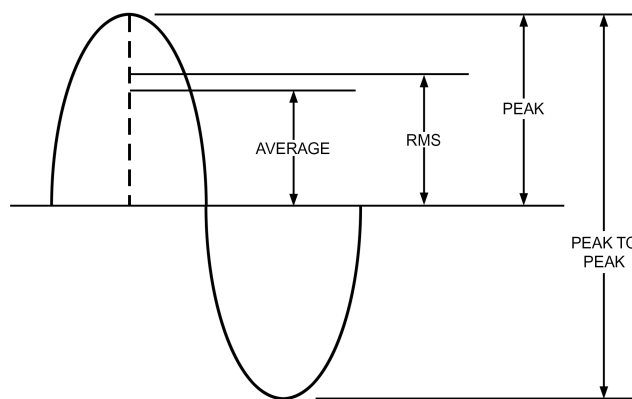
Fig. 39 Vibration Amplitude Terminology
